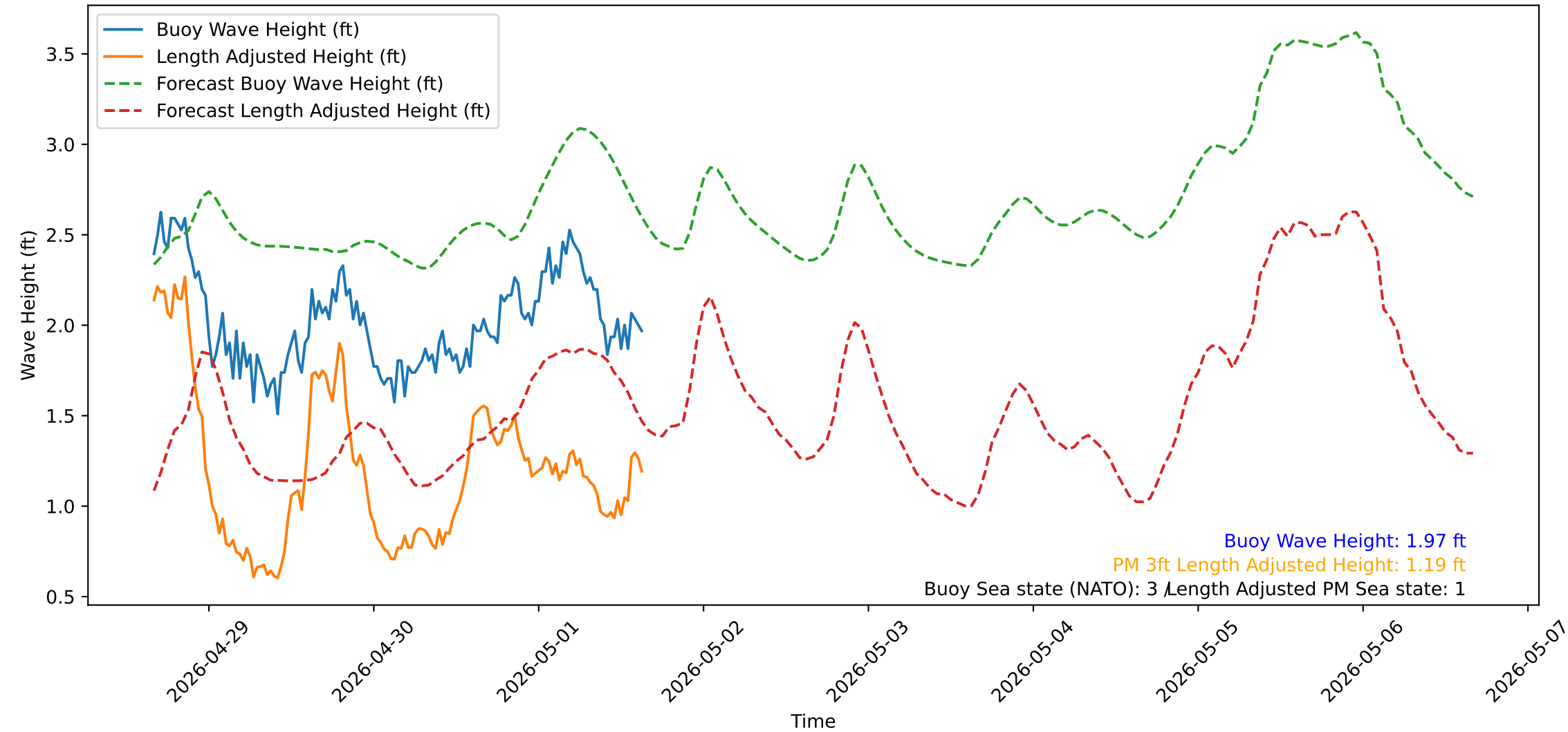
Wave Heights over Time for Red Beach at 2026-05-01 15:40:51
