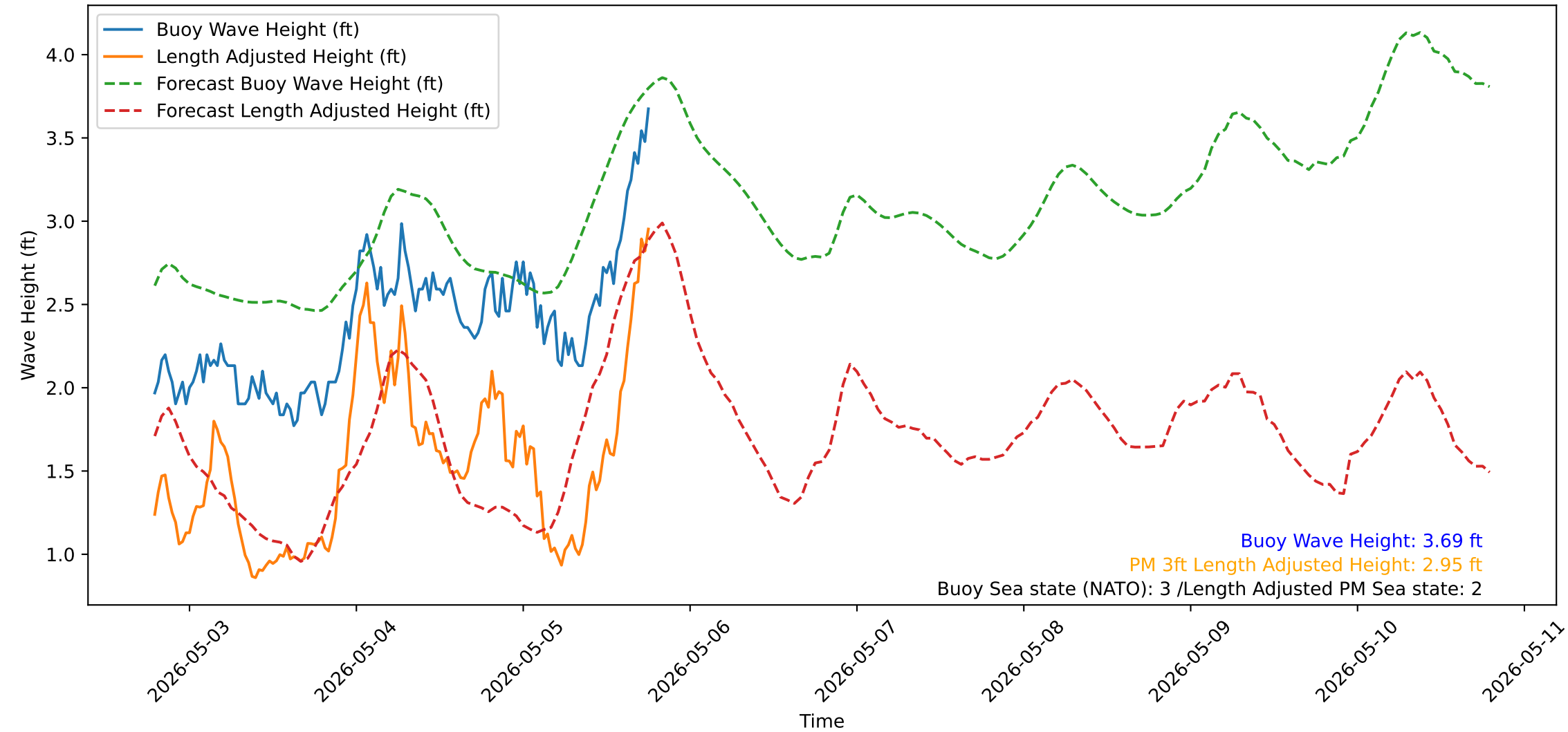
Wave Heights over Time for Green Beach at 2026-05-05 18:51:14
