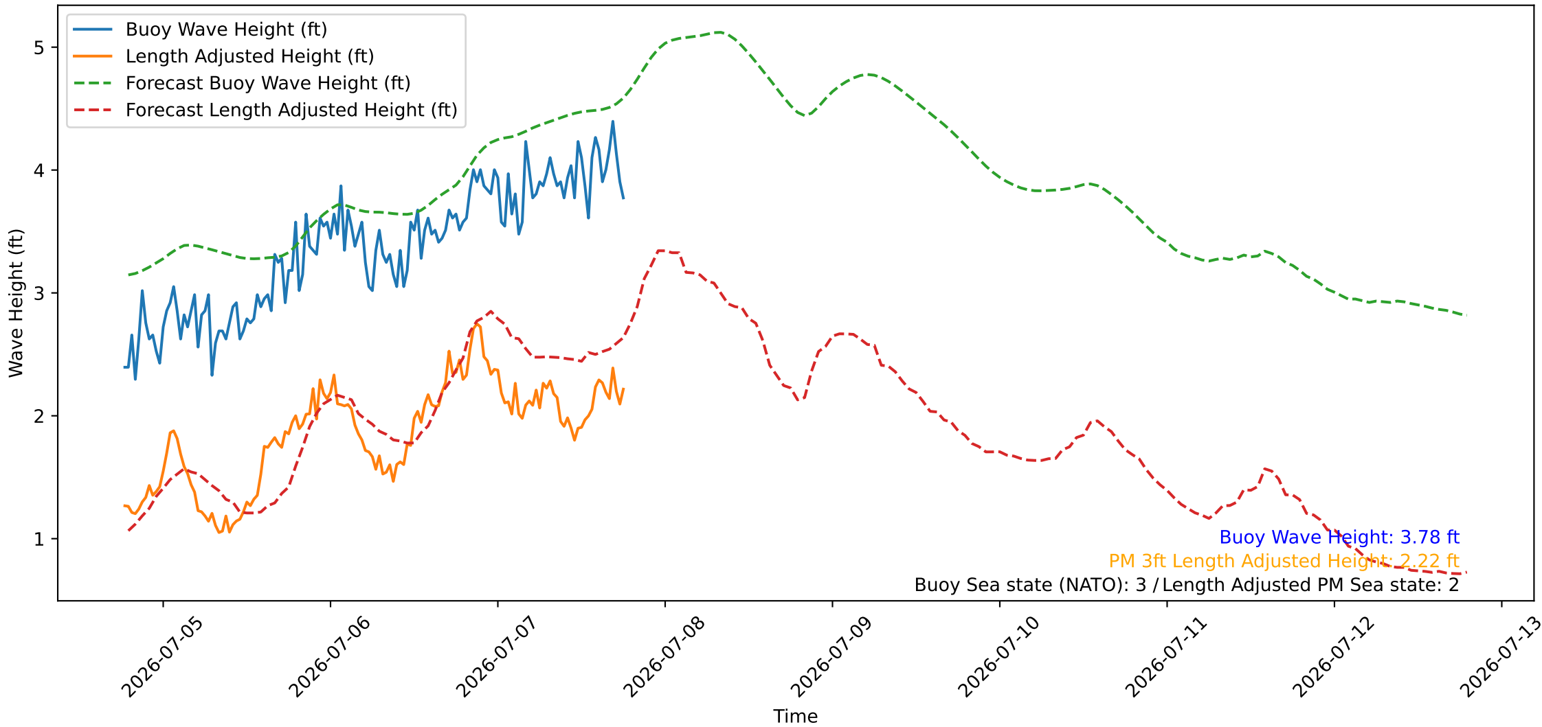
Wave Heights over Time for Oceanside Harbor at 2026-07-07 18:30:26
