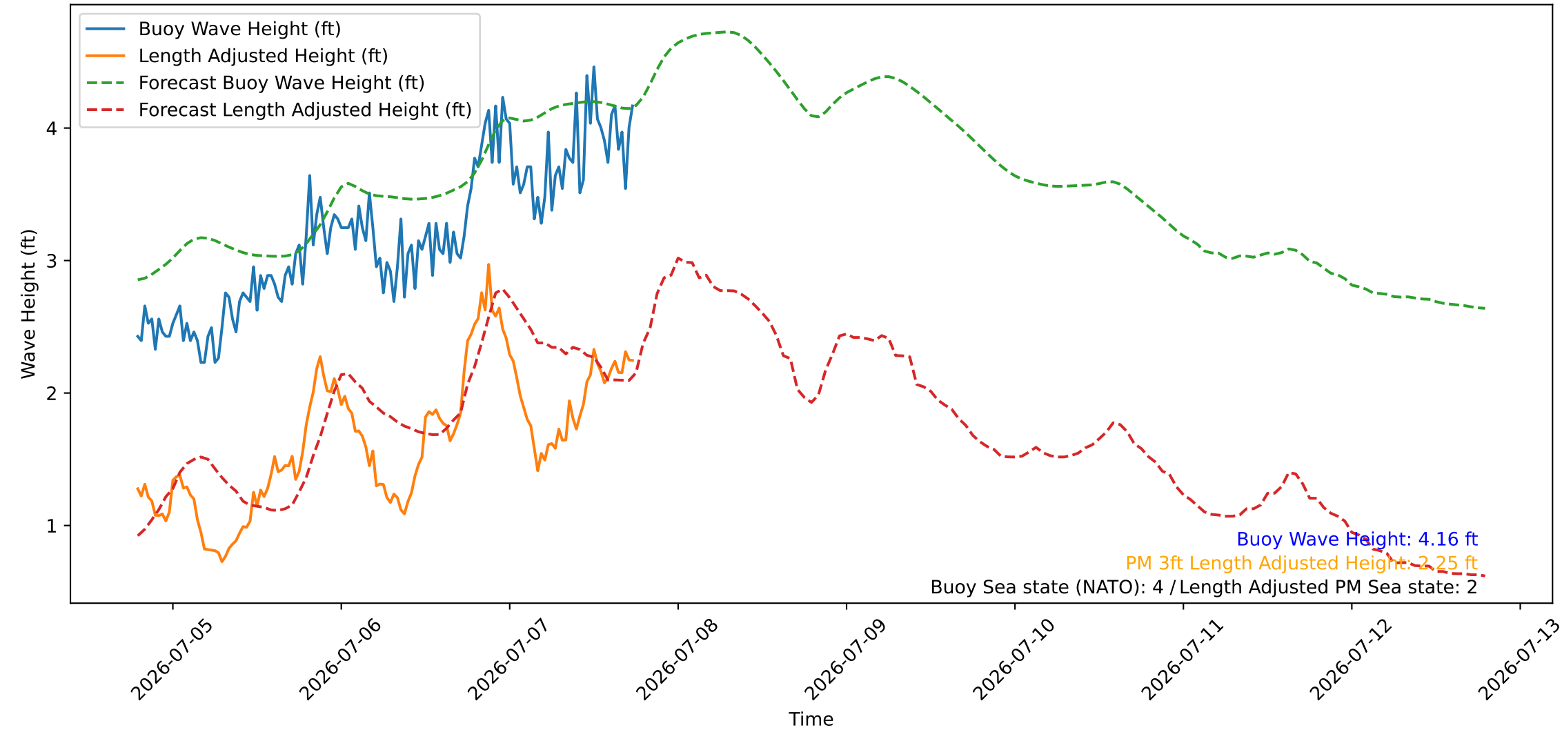
Wave Heights over Time for Red Beach at 2026-07-07 18:30:45
