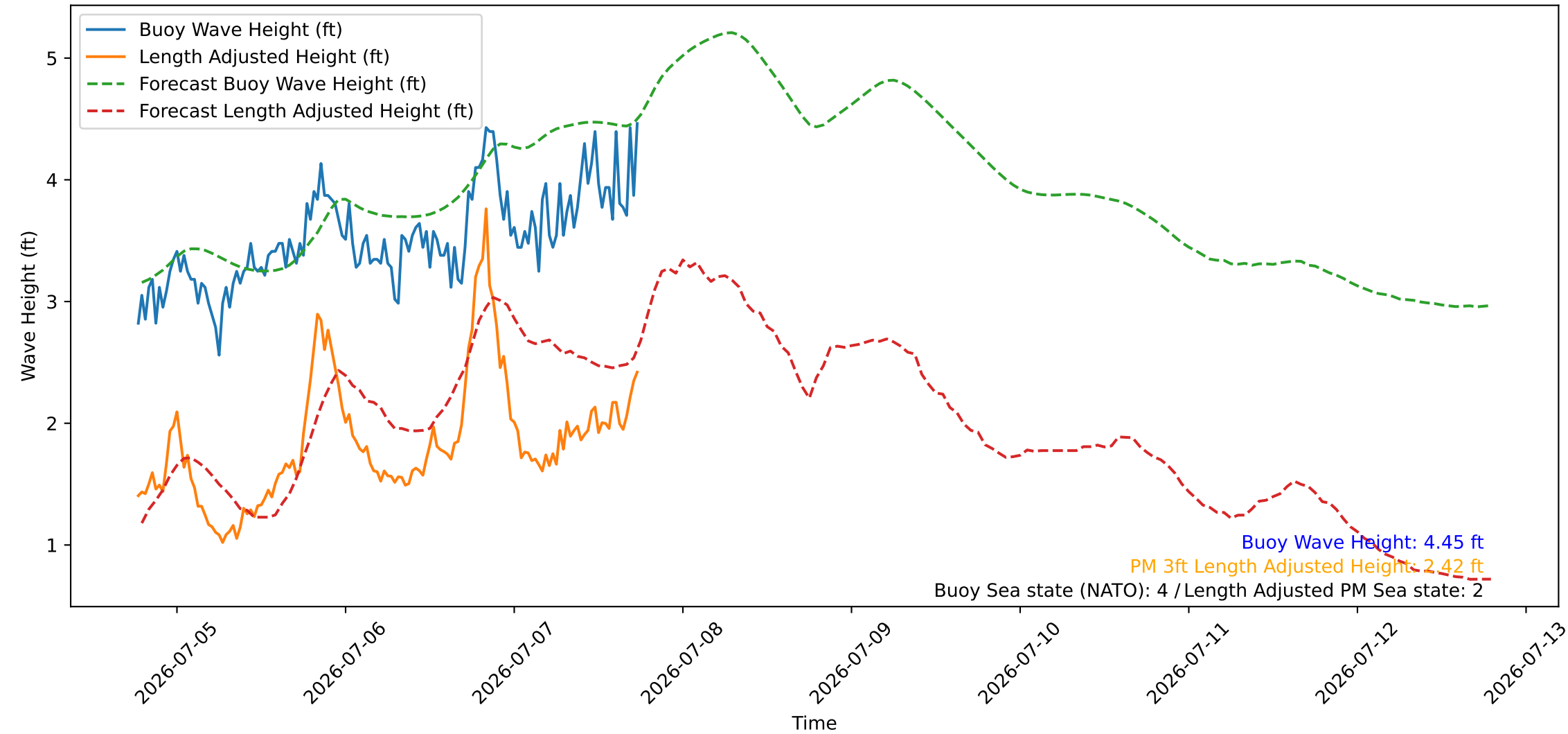
Wave Heights over Time for Green Beach at 2026-07-07 18:31:07
