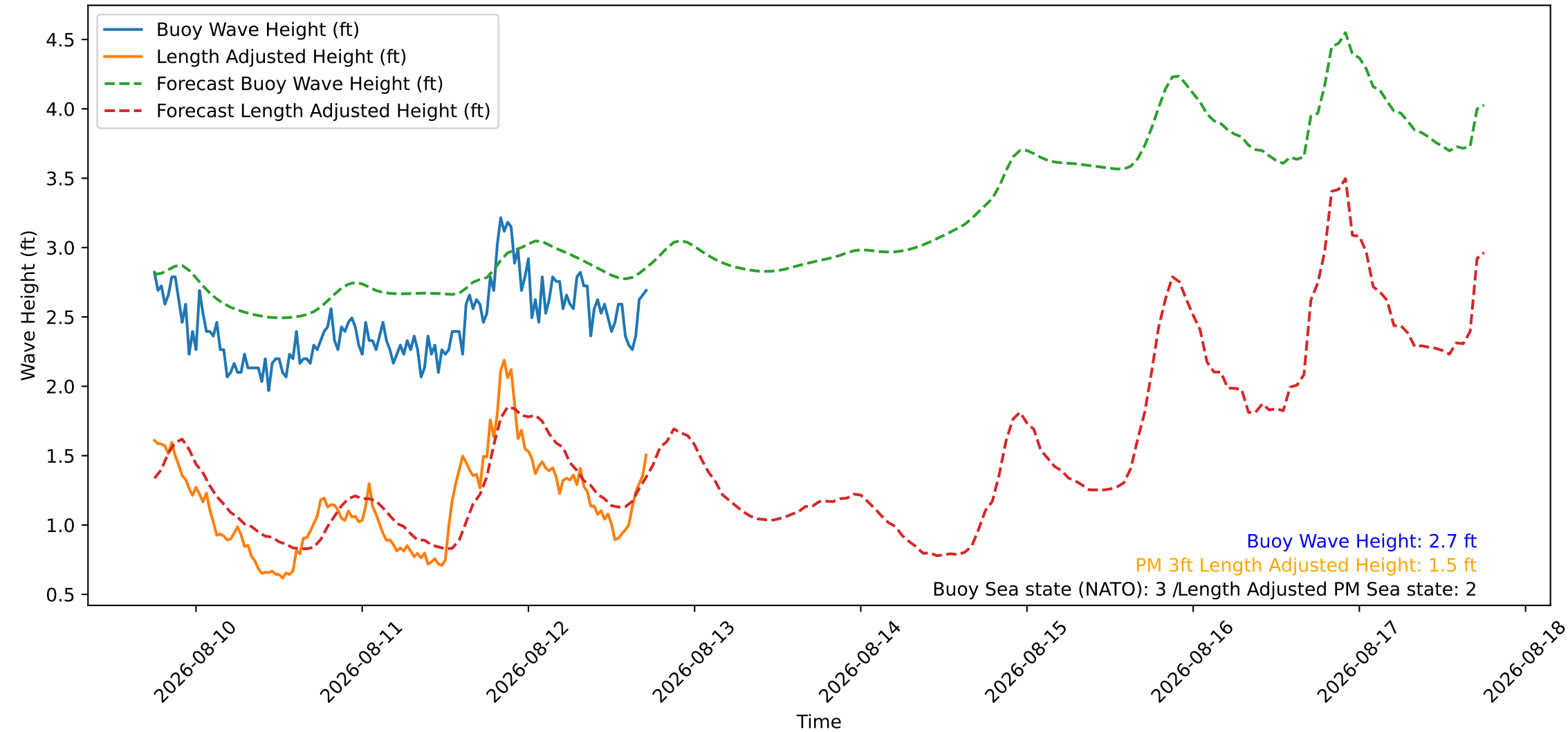
Wave Heights over Time for Green Beach at 2026-08-12 18:01:08
