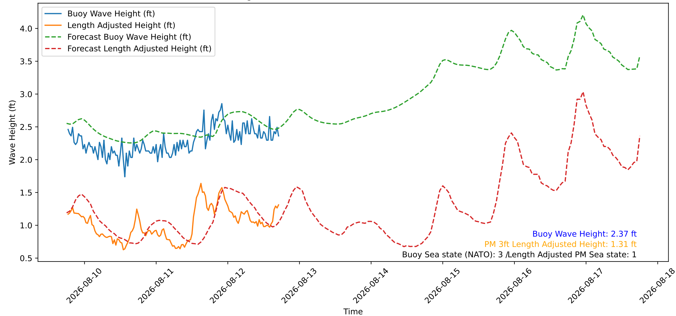
Wave Heights over Time for Red Beach at 2026-08-12 18:00:45
