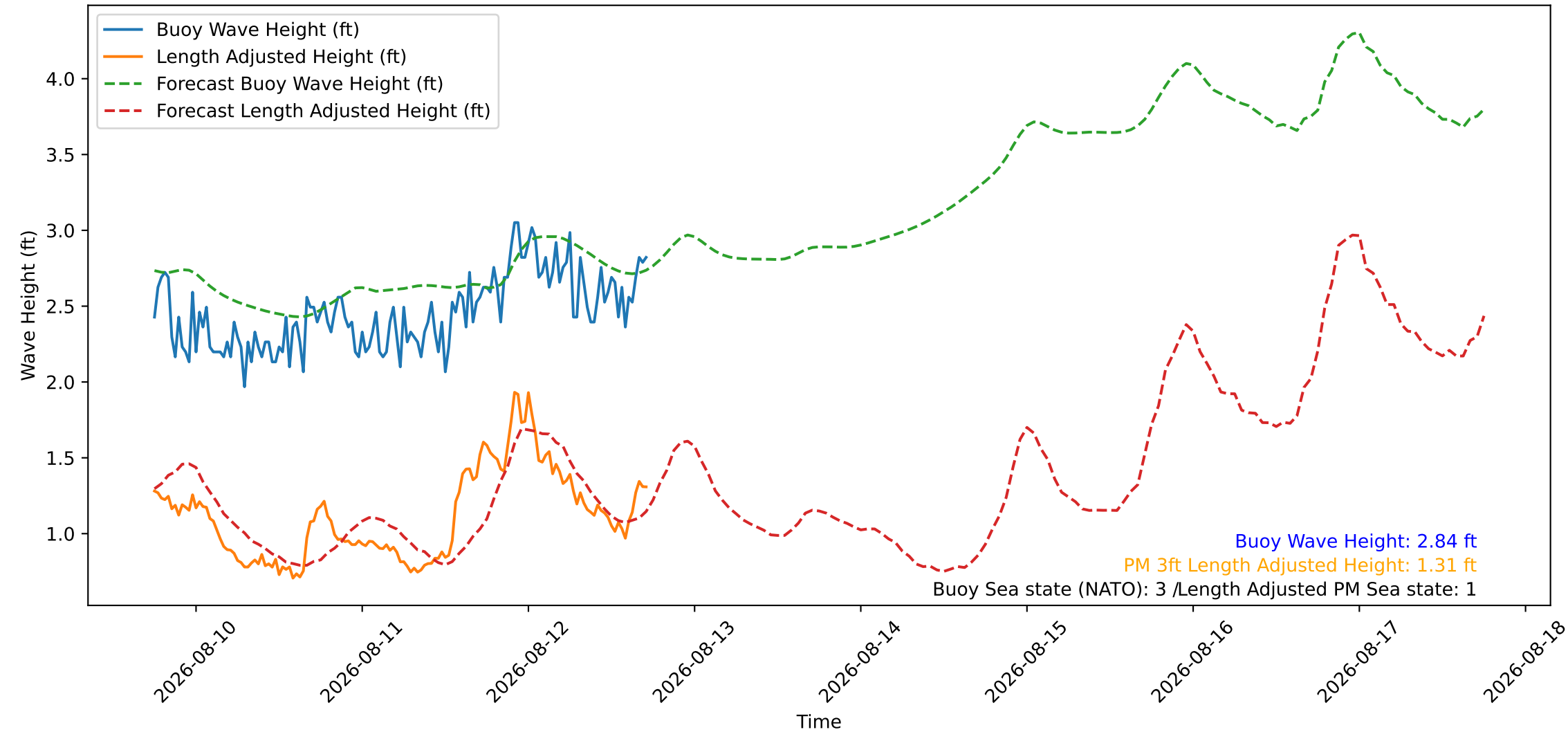
Wave Heights over Time for Oceanside Harbor at 2026-08-12 18:00:26
