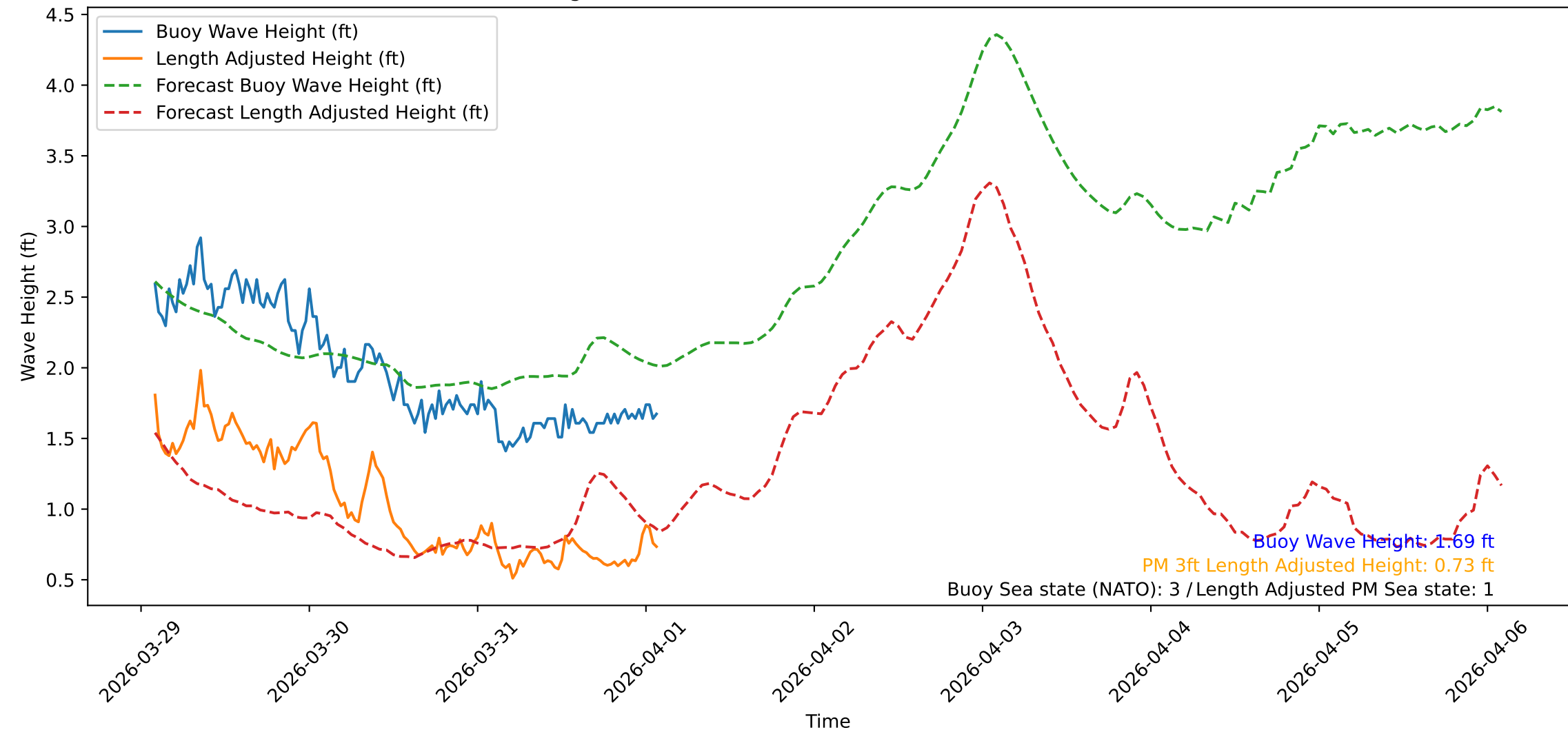
Wave Heights over Time for Green Beach at 2026-04-01 02:11:09
