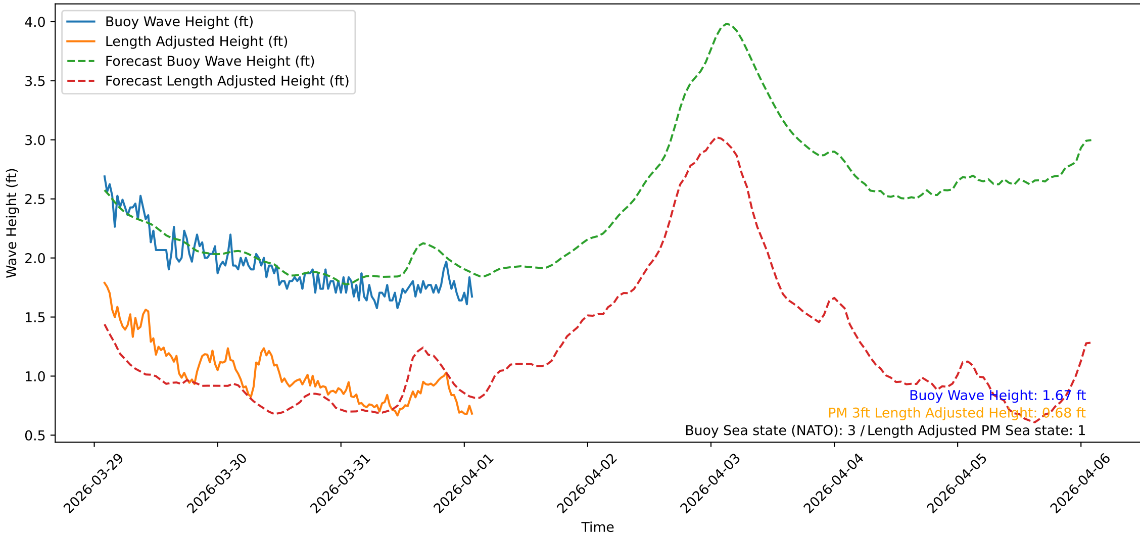
Wave Heights over Time for Oceanside Harbor at 2026-04-01 02:10:31
