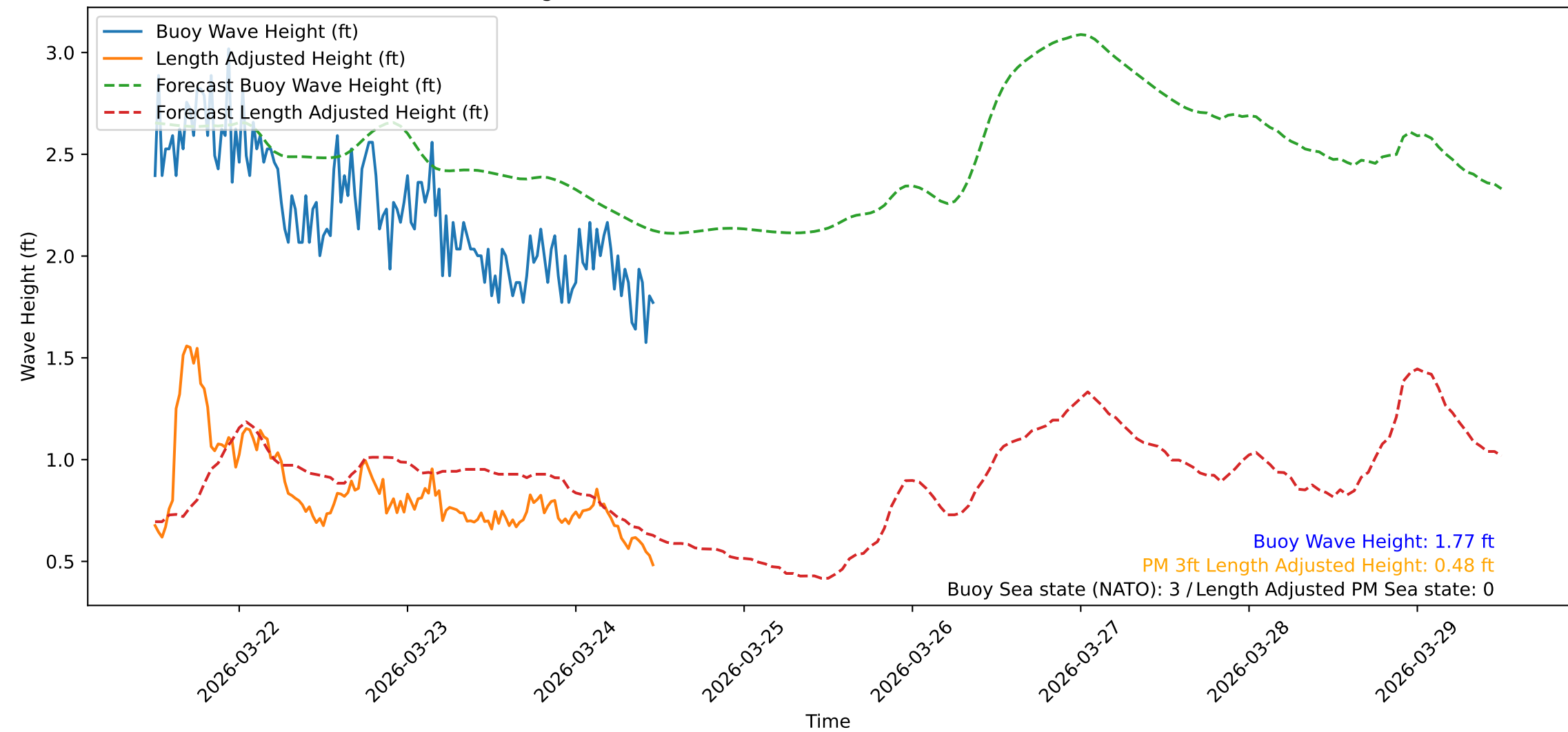
Wave Heights over Time for Oceanside Harbor at 2026-03-24 11:50:32
