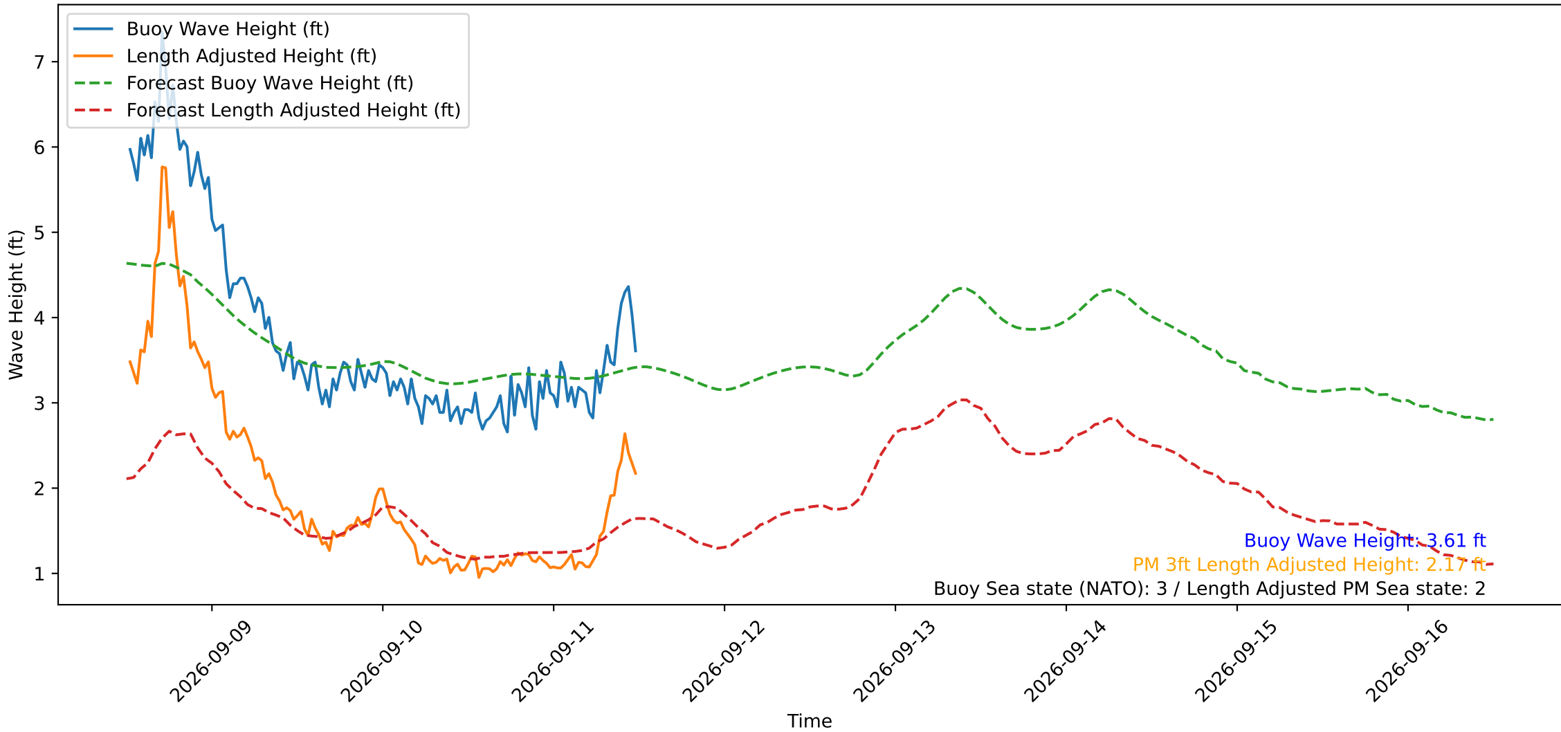
Wave Heights over Time for Oceanside Harbor at 2026-09-11 12:20:29
