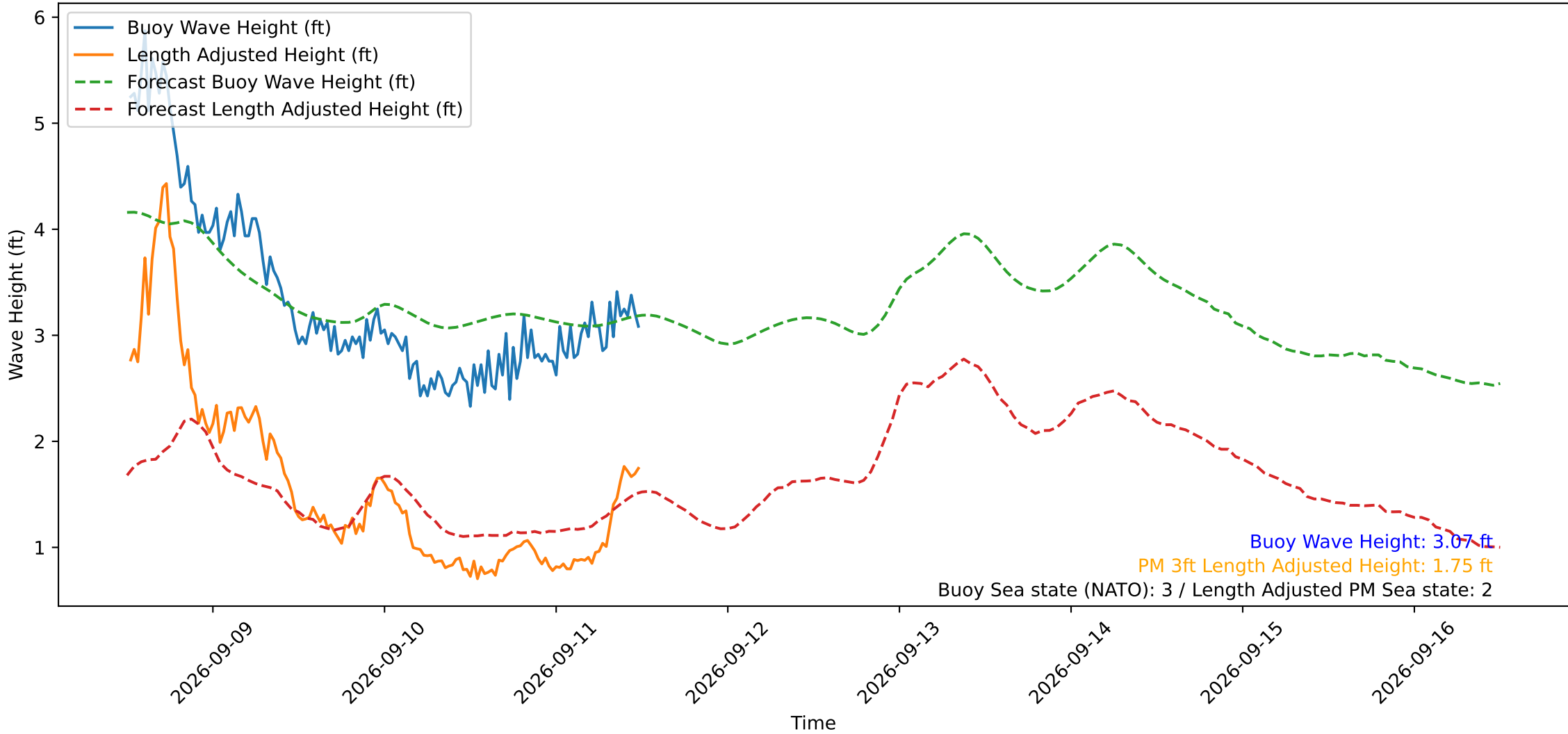
Wave Heights over Time for Red Beach at 2026-09-11 12:20:51
