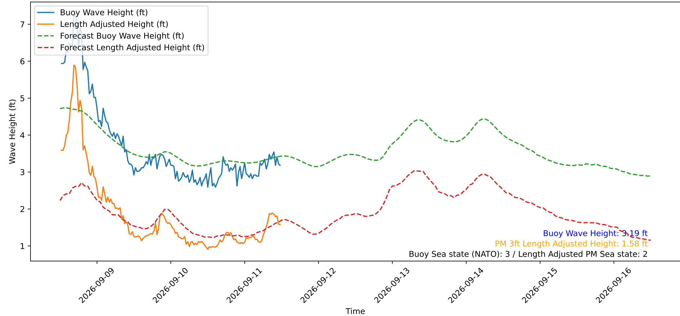
Wave Heights over Time for Green Beach at 2026-09-11 12:21:14
