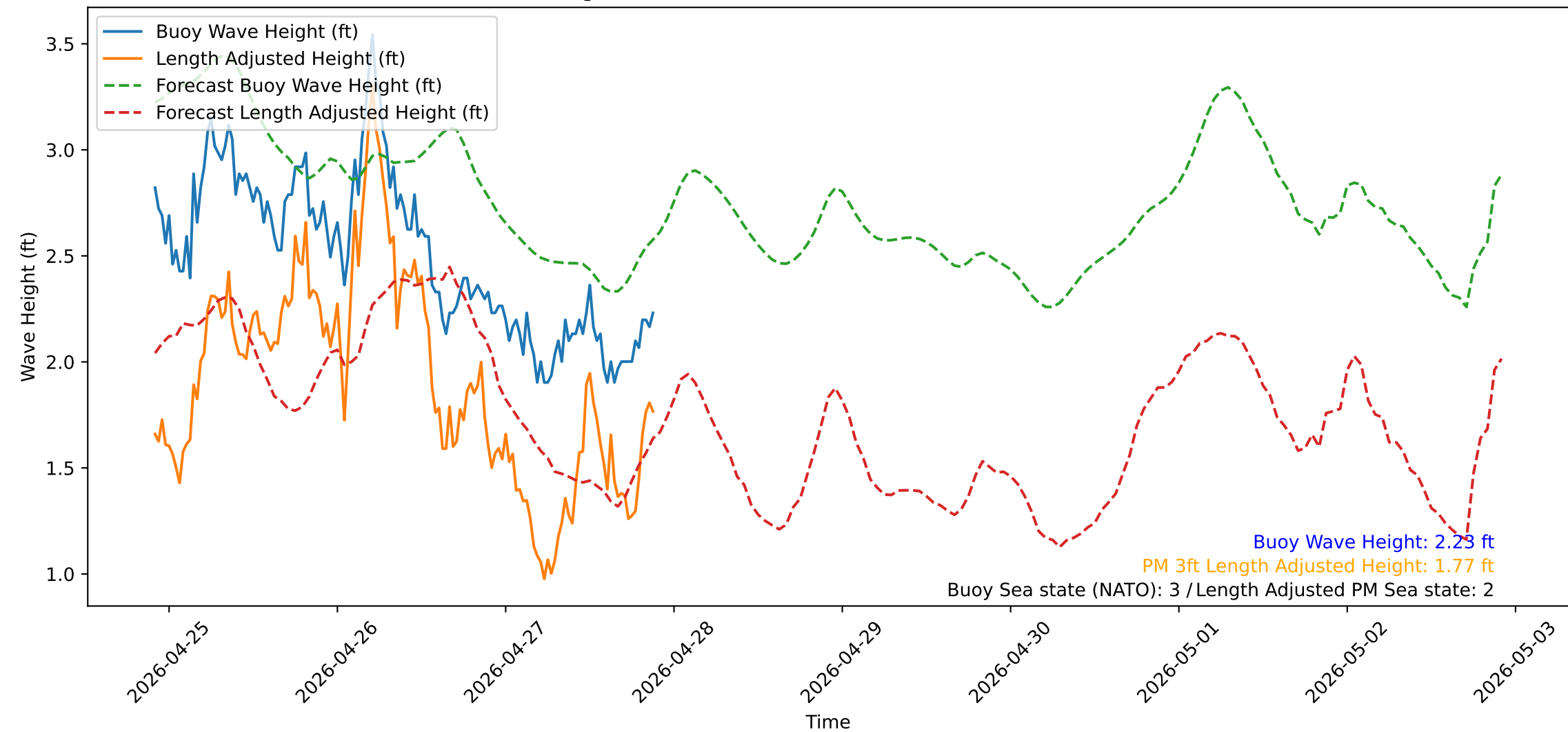
Wave Heights over Time for Red Beach at 2026-04-27 21:40:50
