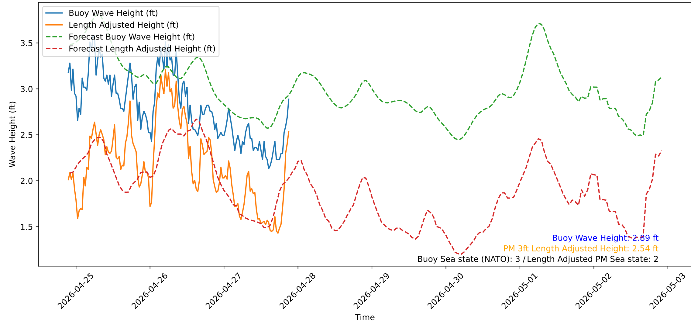
Wave Heights over Time for Green Beach at 2026-04-27 21:41:13
