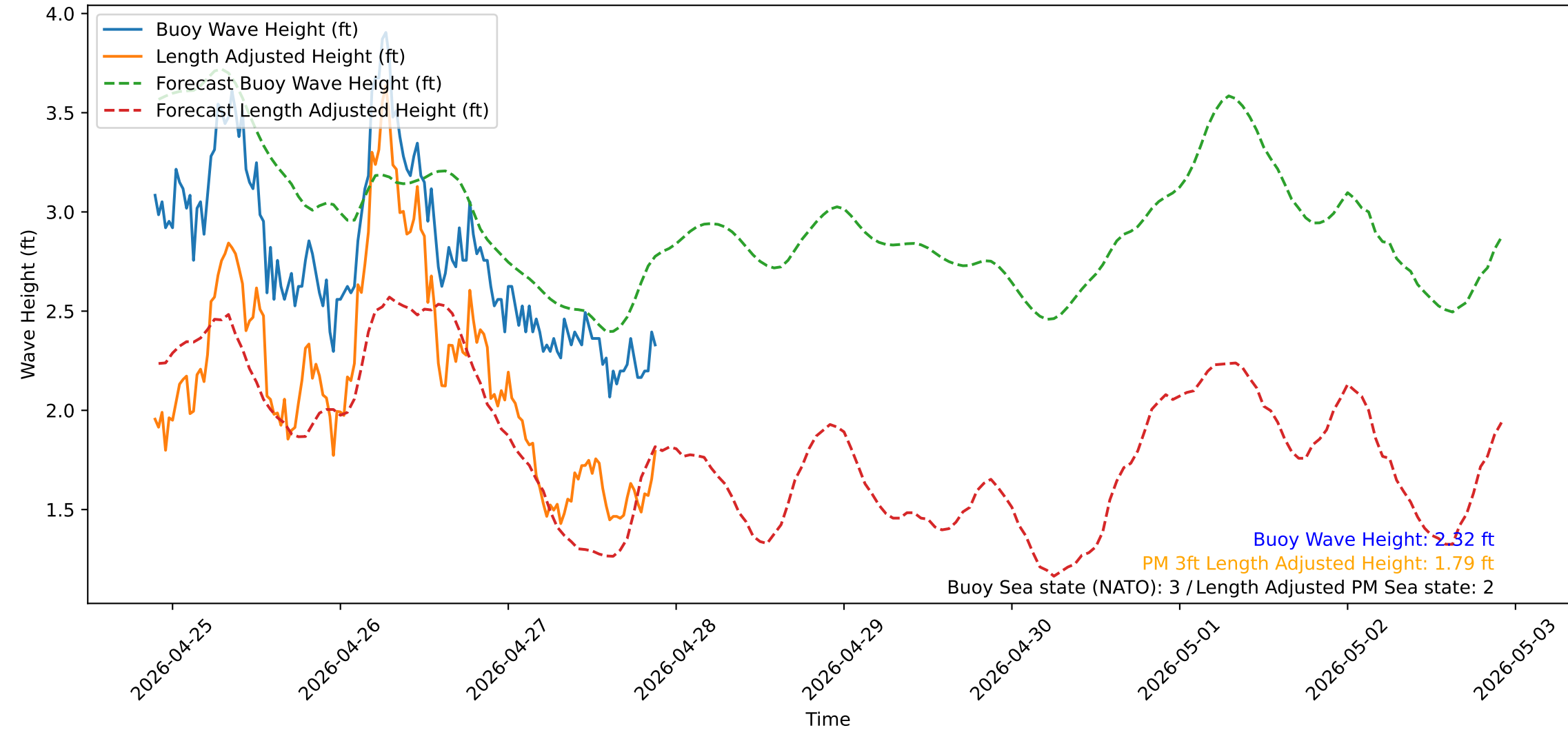
Wave Heights over Time for Oceanside Harbor at 2026-04-27 21:40:31
