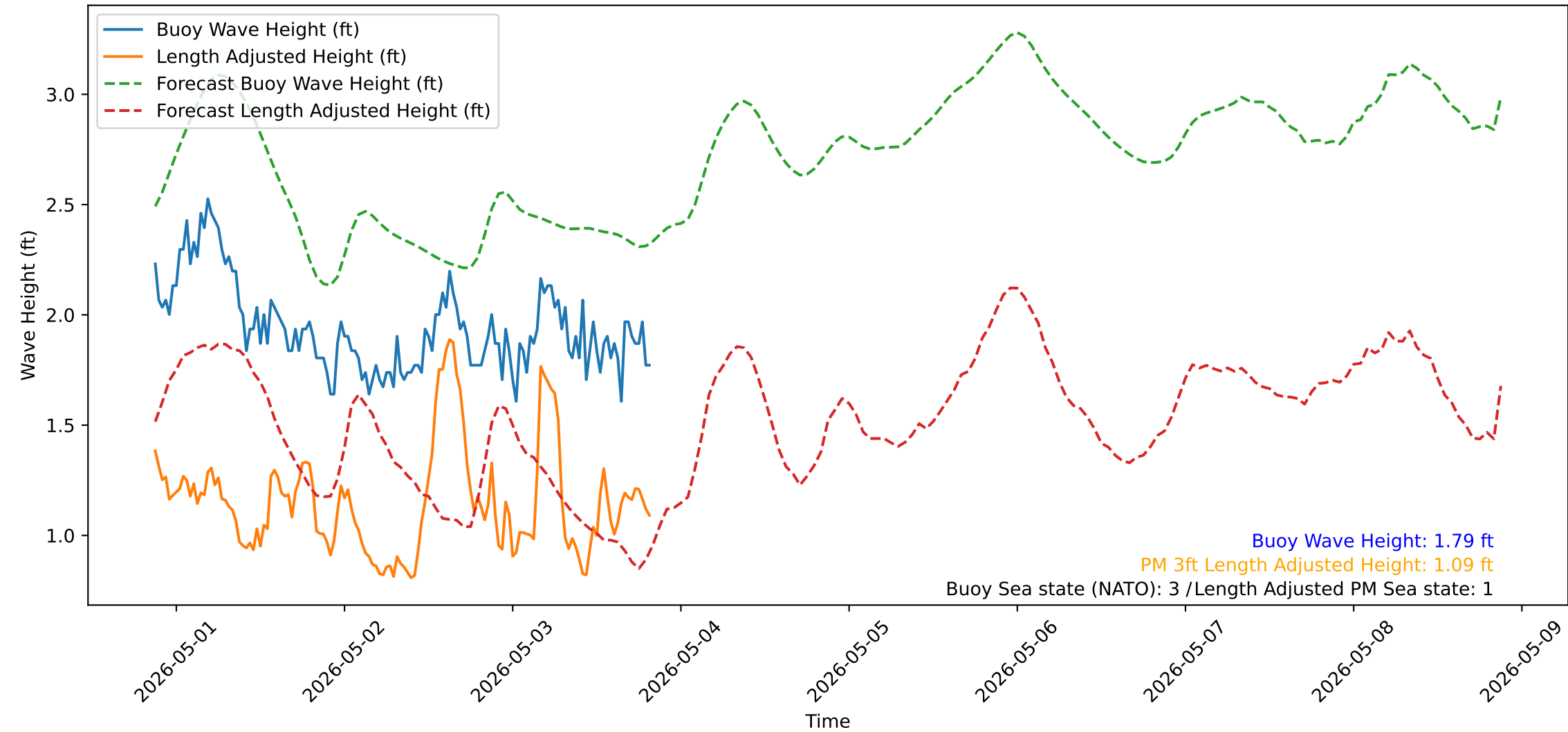
Wave Heights over Time for Red Beach at 2026-05-03 20:30:50
