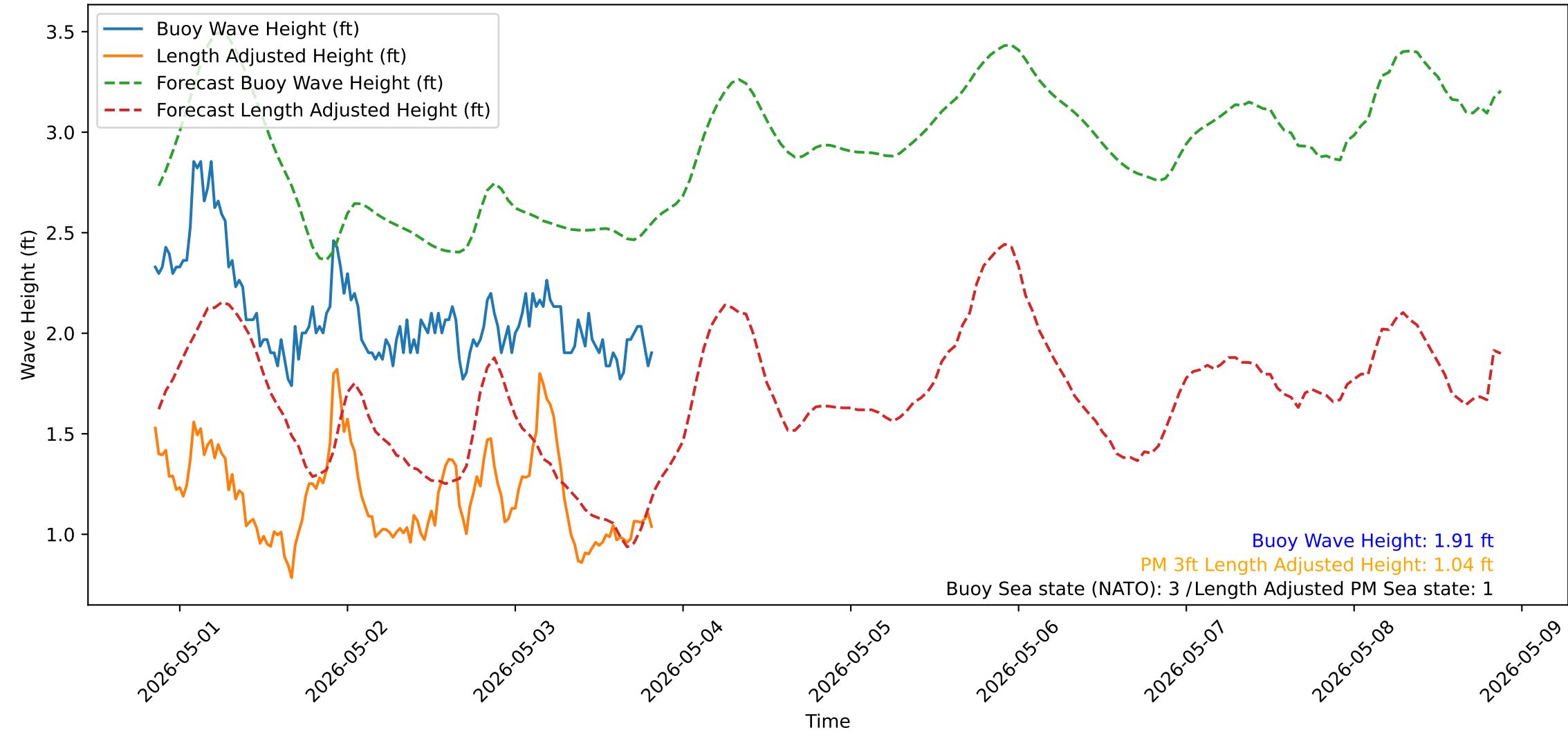
Wave Heights over Time for Green Beach at 2026-05-03 20:31:12
