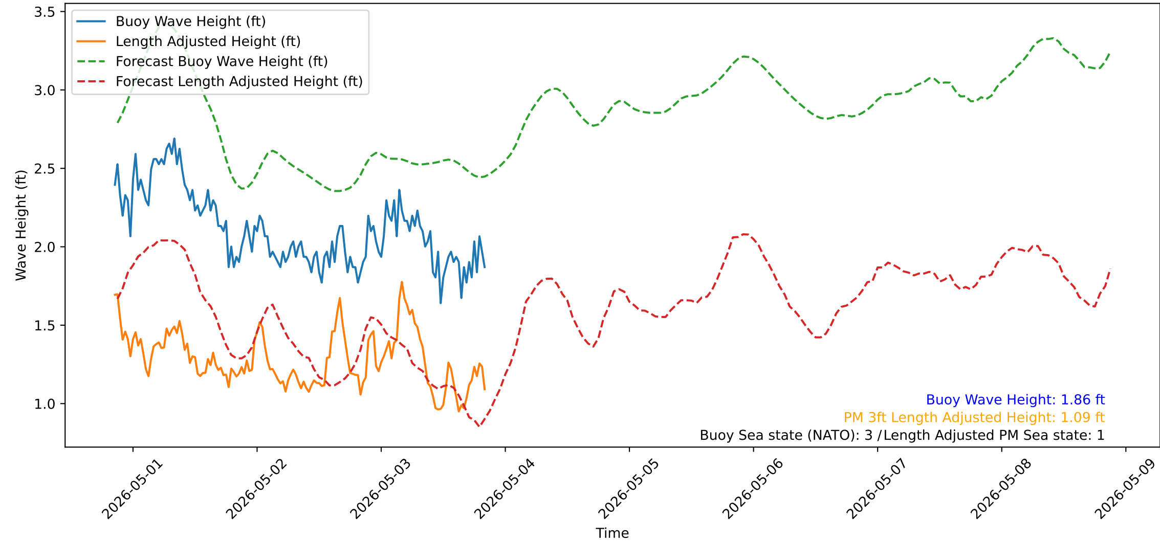
Wave Heights over Time for Oceanside Harbor at 2026-05-03 20:30:31
