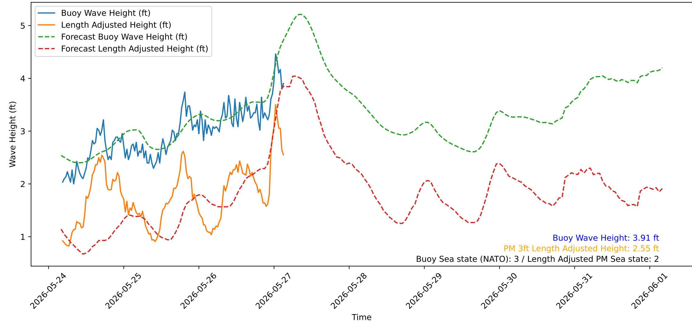
Wave Heights over Time for Red Beach at 2026-05-27 04:00:46
