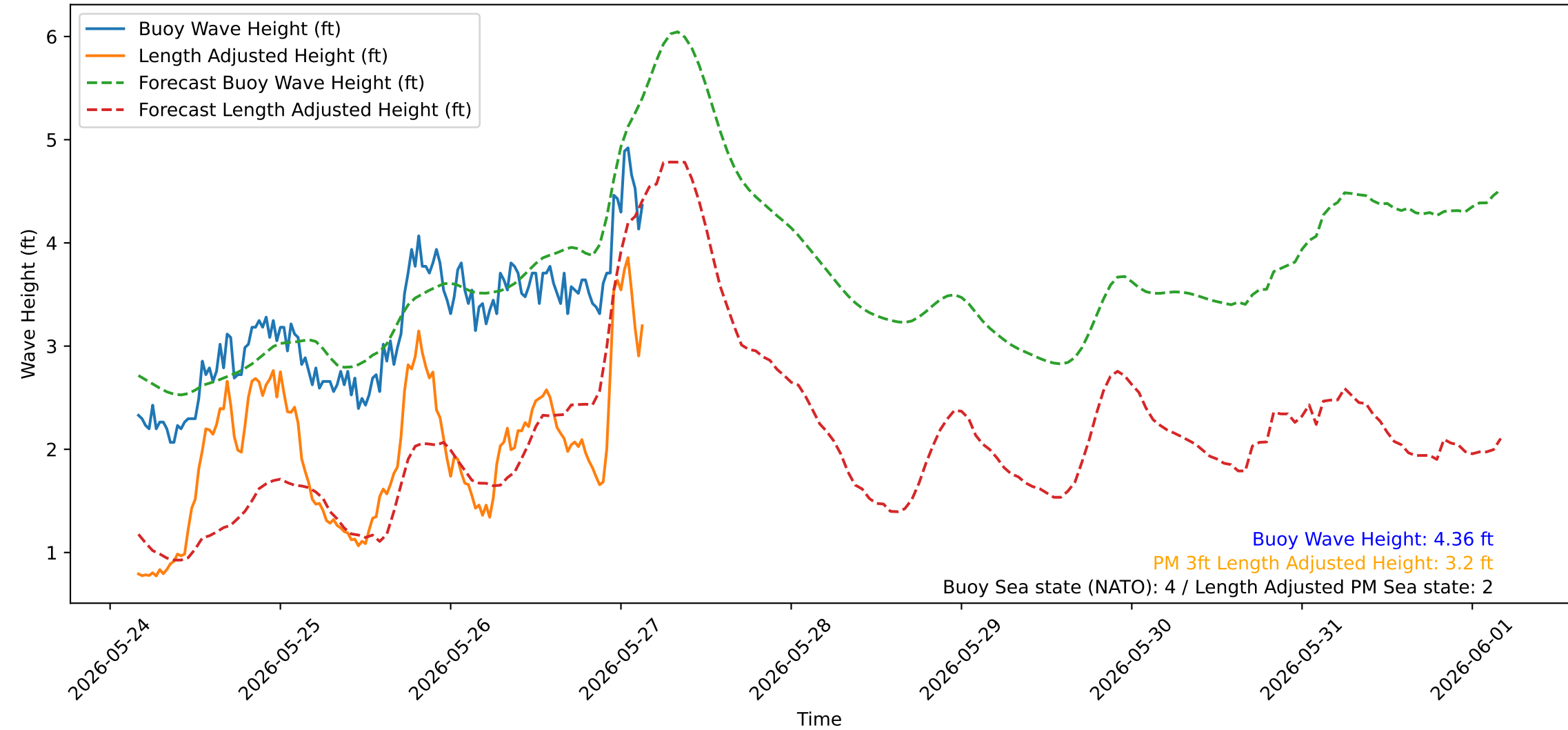
Wave Heights over Time for Green Beach at 2026-05-27 04:01:09
