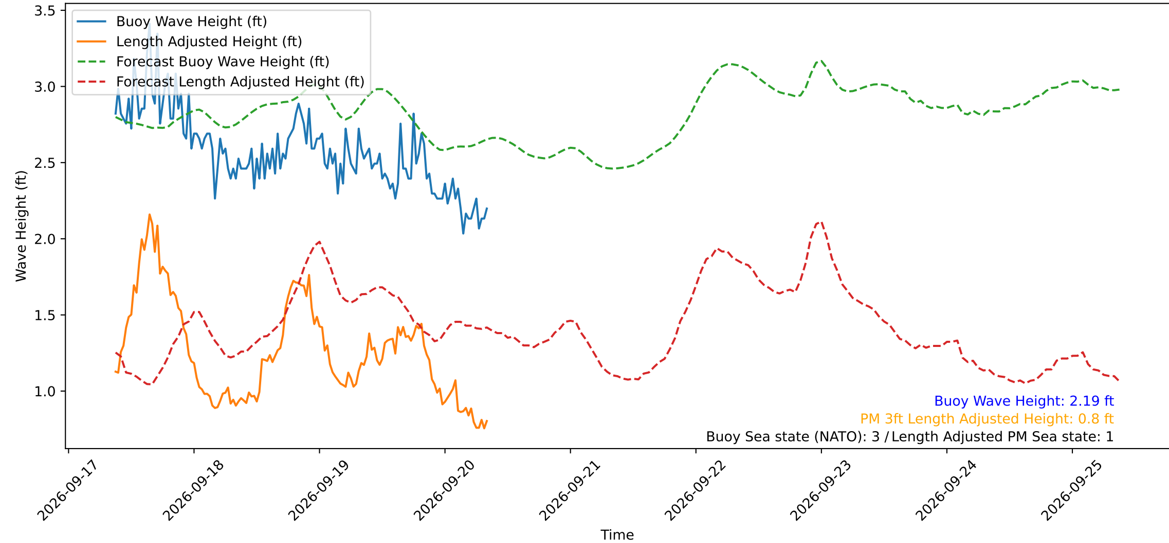
Wave Heights over Time for Red Beach at 2026-09-20 08:40:49
