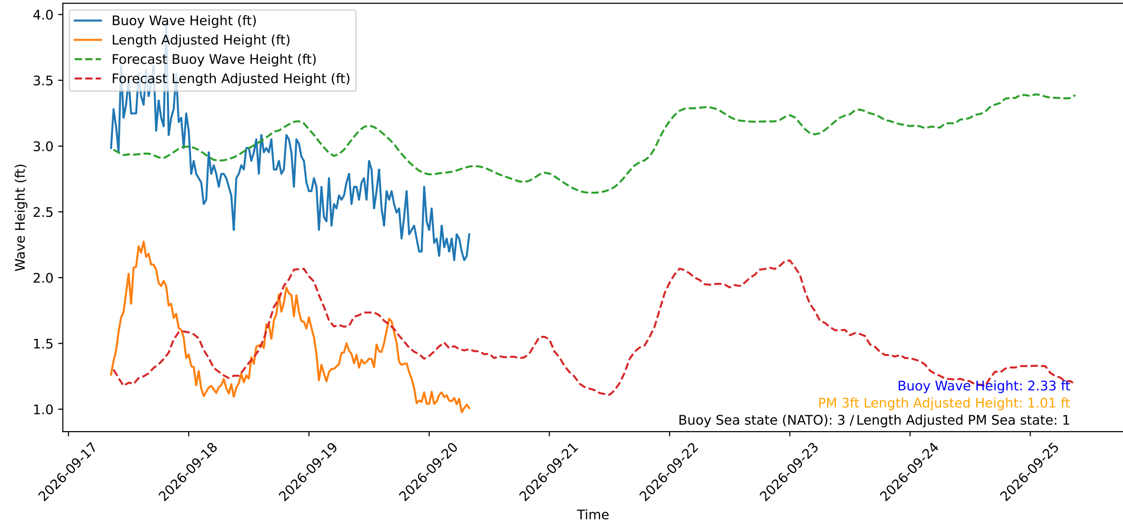
Wave Heights over Time for Oceanside Harbor at 2026-09-20 08:40:29
