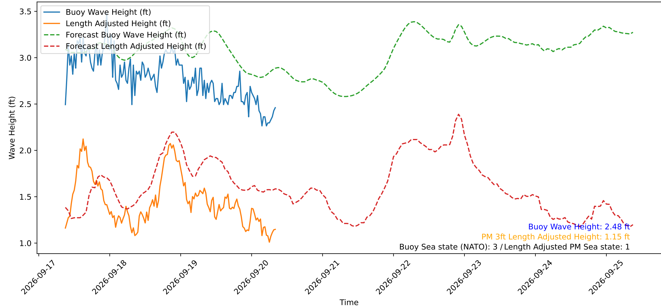
Wave Heights over Time for Green Beach at 2026-09-20 08:41:12
