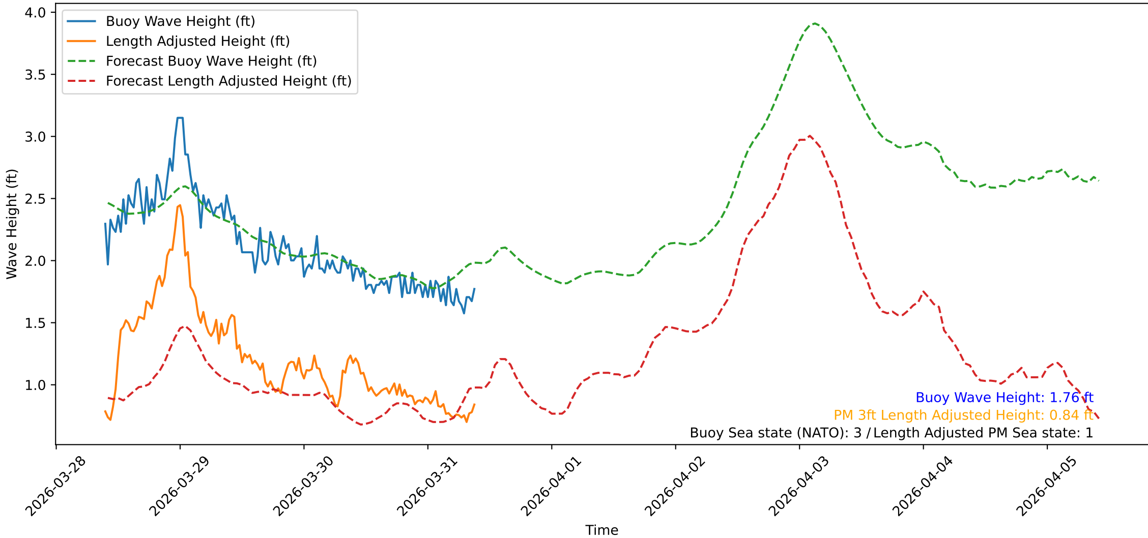
Wave Heights over Time for Oceanside Harbor at 2026-03-31 09:40:31
