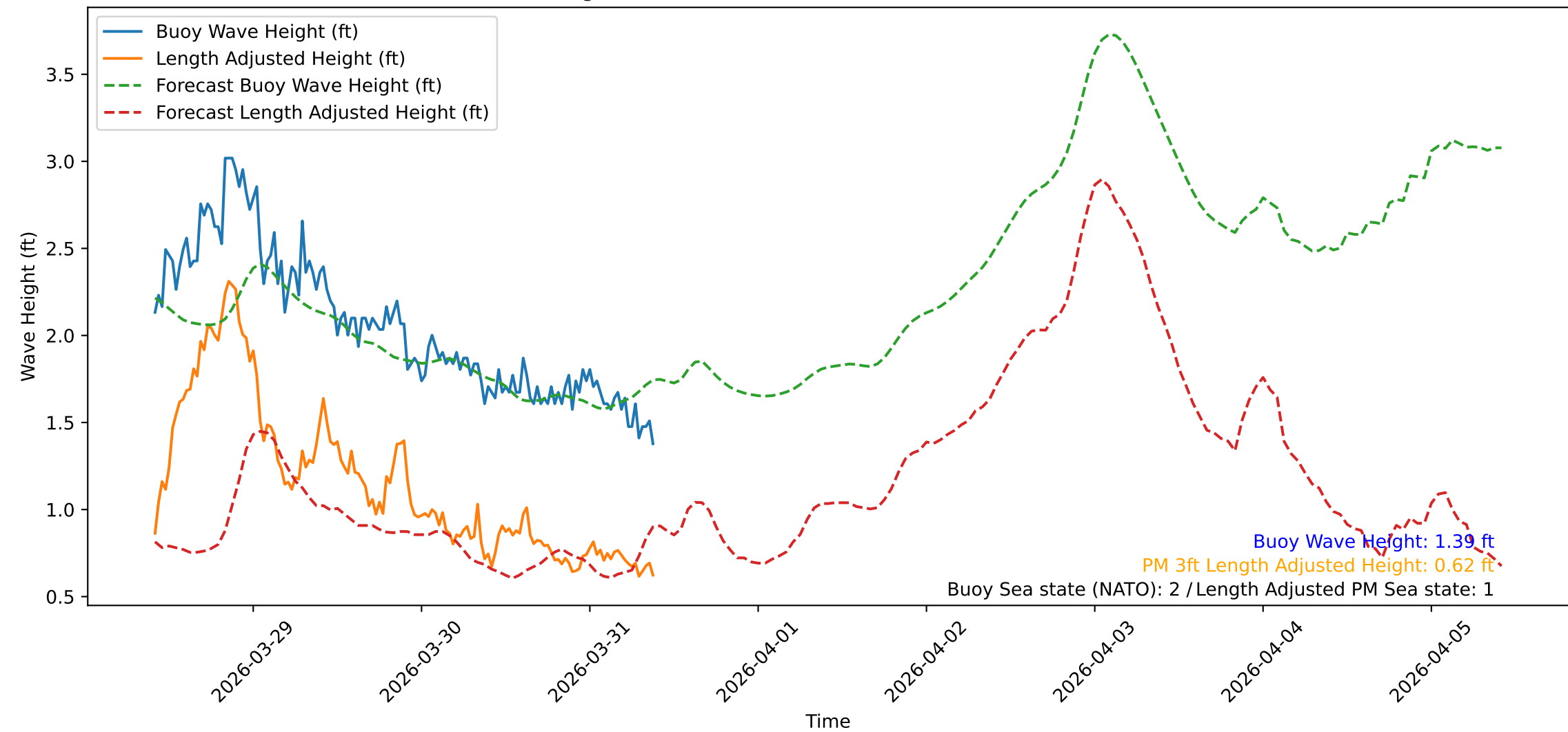
Wave Heights over Time for Red Beach at 2026-03-31 09:40:48
