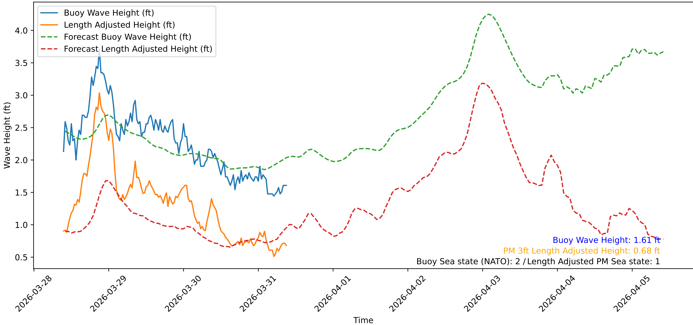
Wave Heights over Time for Green Beach at 2026-03-31 09:41:10
