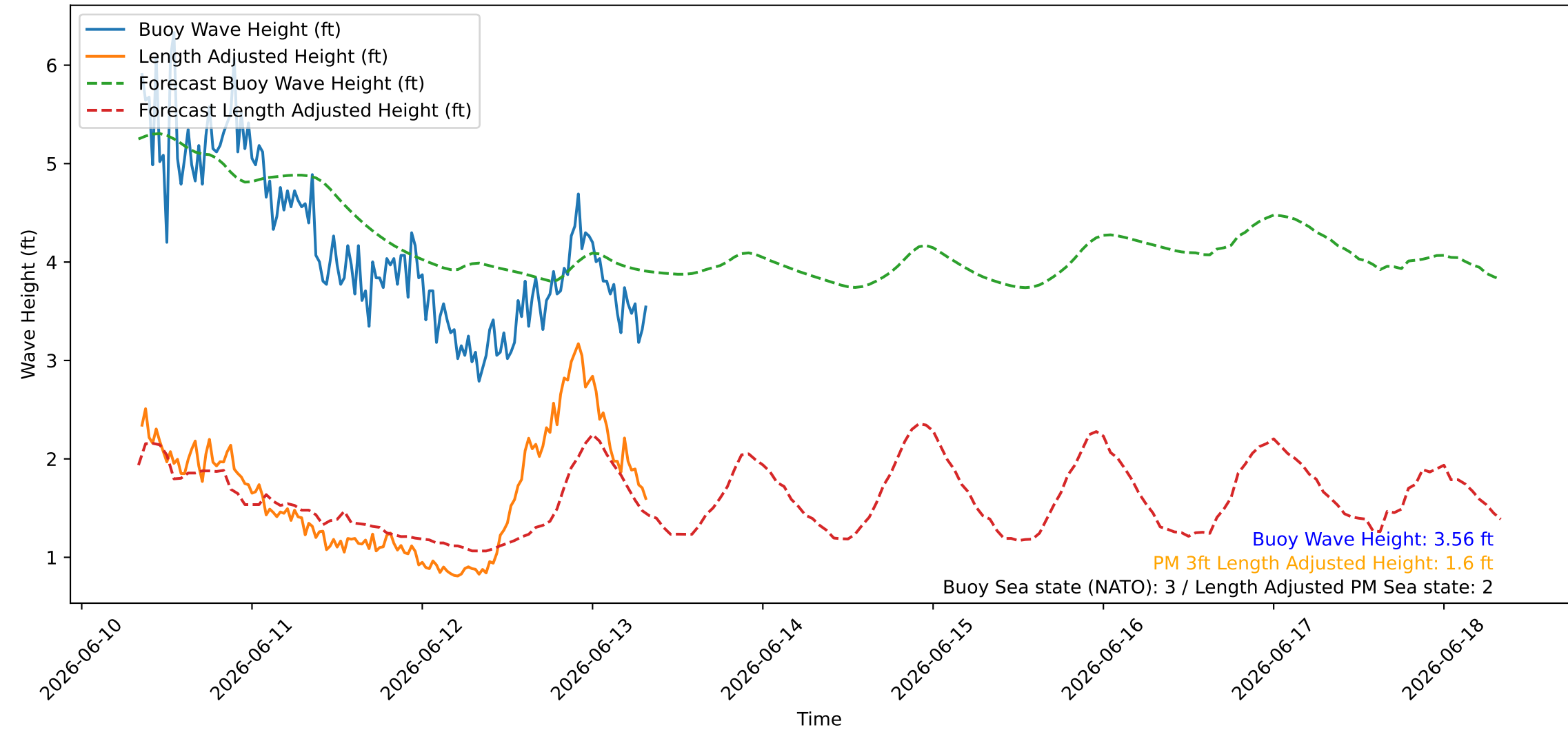
Wave Heights over Time for Oceanside Harbor at 2026-06-13 08:20:26
