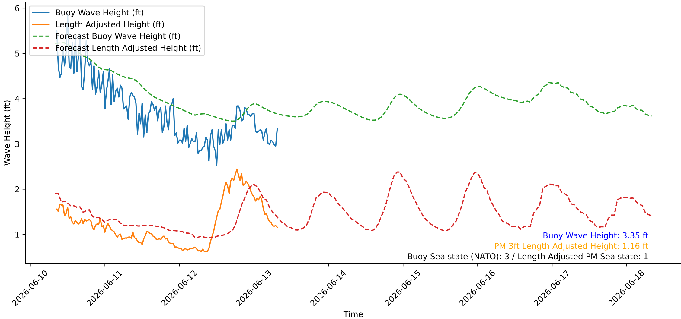
Wave Heights over Time for Red Beach at 2026-06-13 08:20:47
