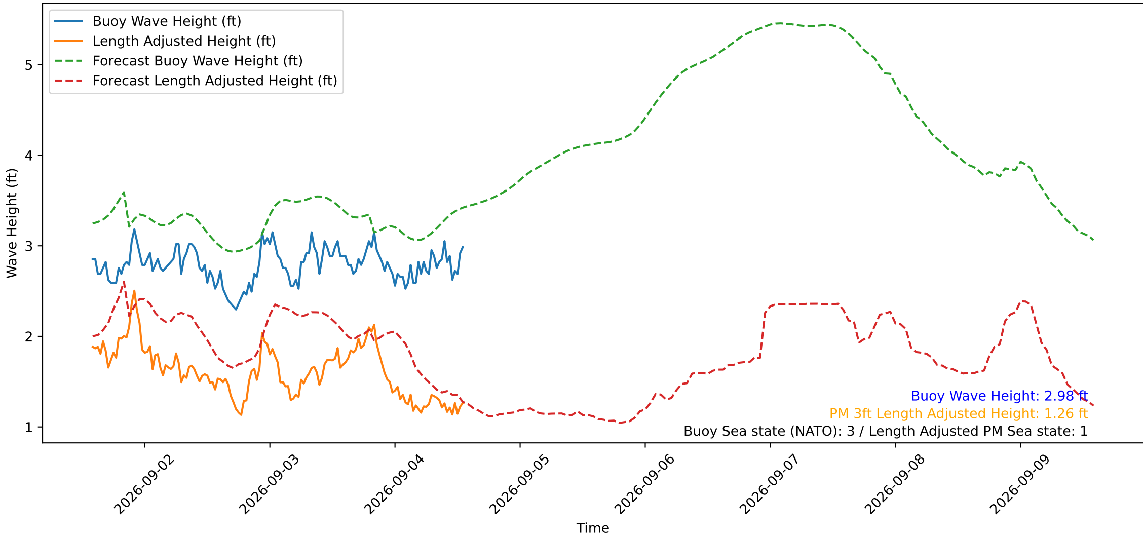
Wave Heights over Time for Red Beach at 2026-09-04 13:40:50
