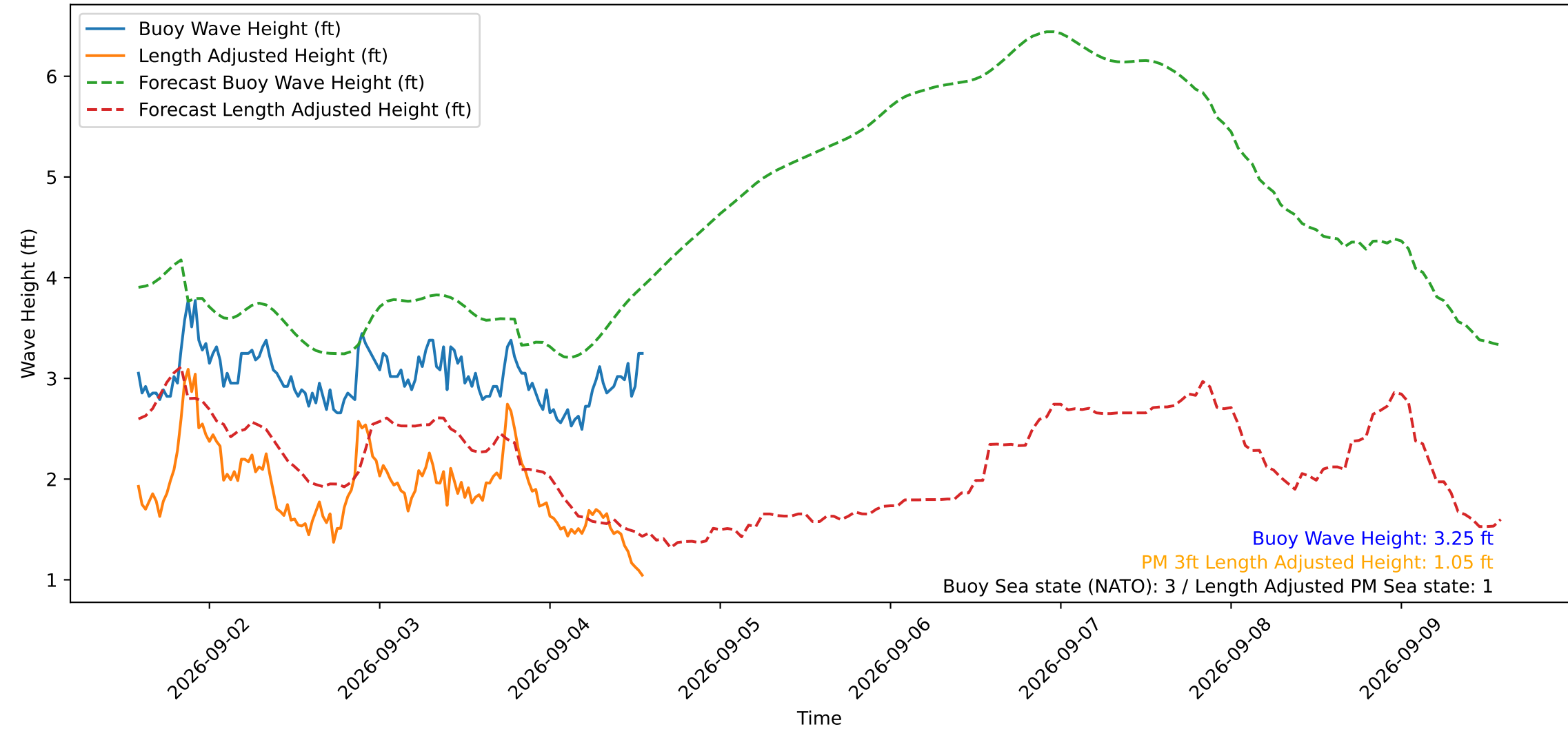
Wave Heights over Time for Green Beach at 2026-09-04 13:41:13
