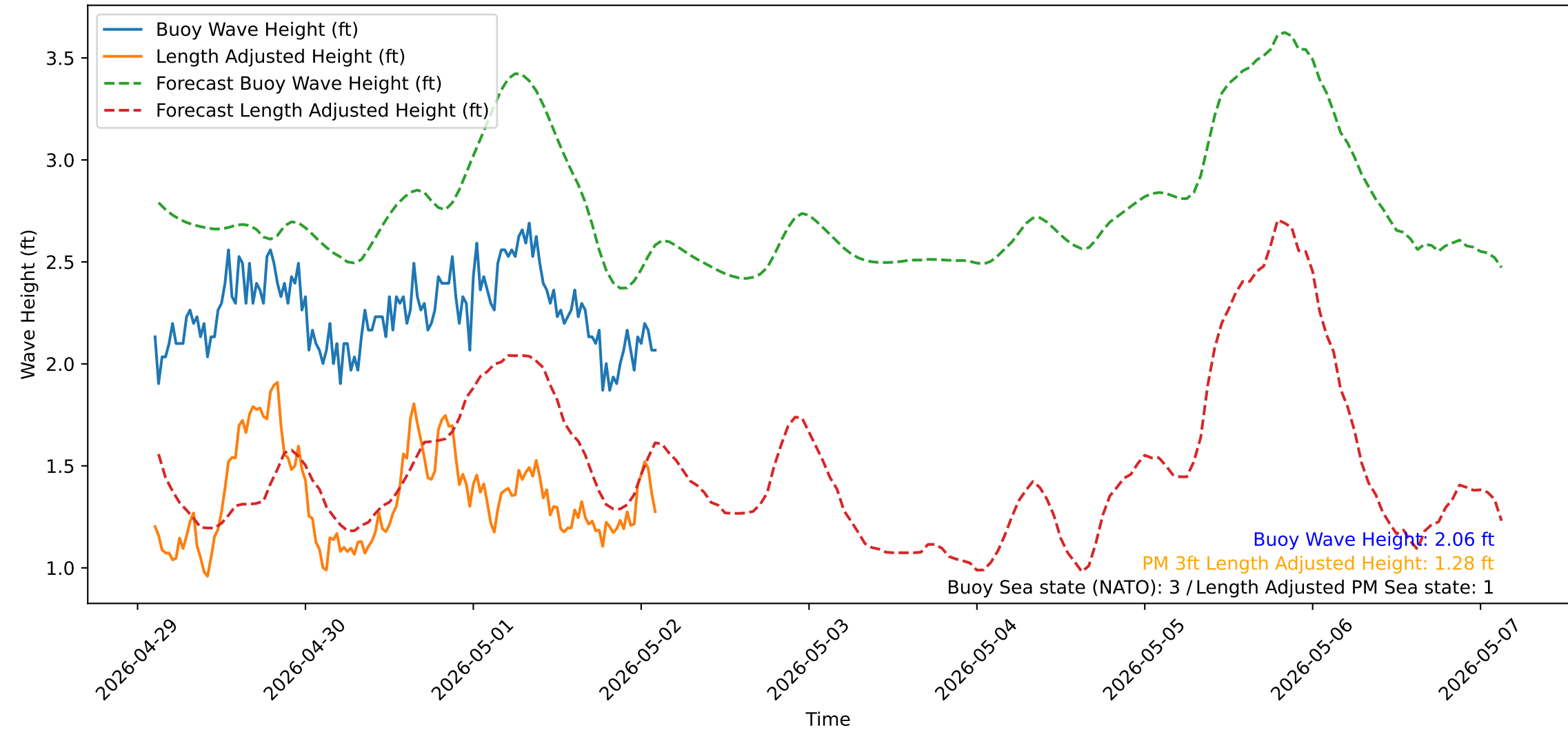
Wave Heights over Time for Oceanside Harbor at 2026-05-02 02:40:31
