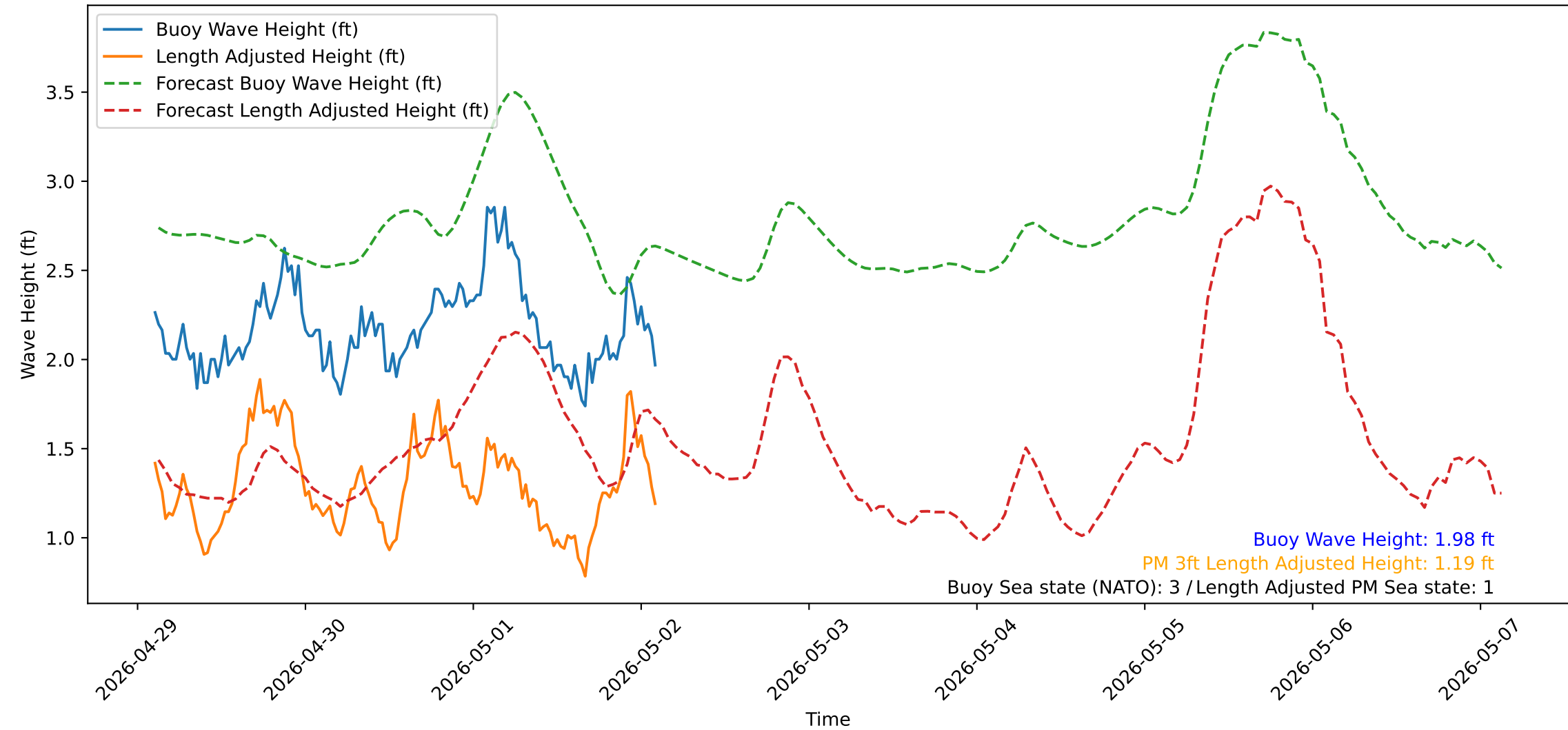
Wave Heights over Time for Green Beach at 2026-05-02 02:41:14
