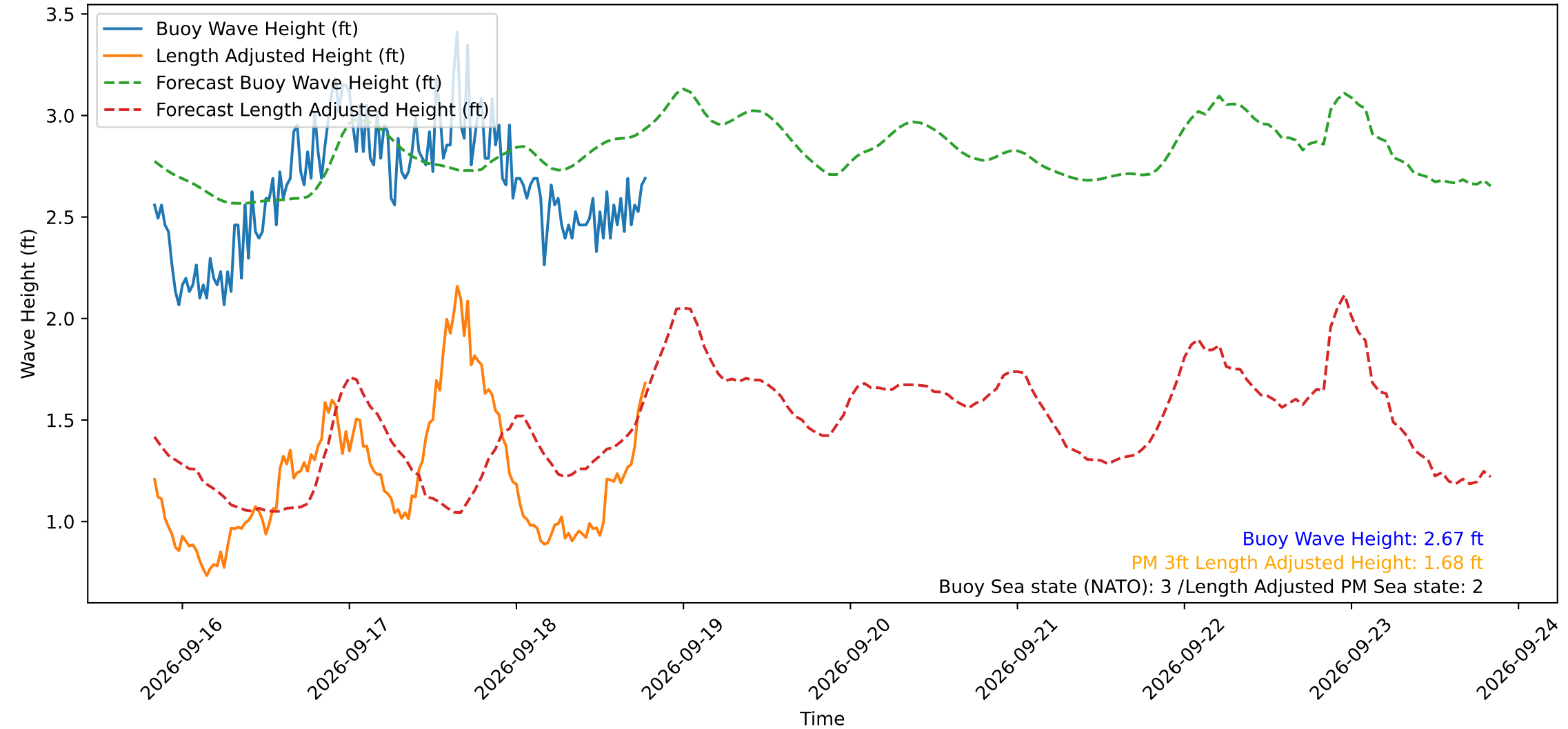
Wave Heights over Time for Red Beach at 2026-09-18 19:30:48
