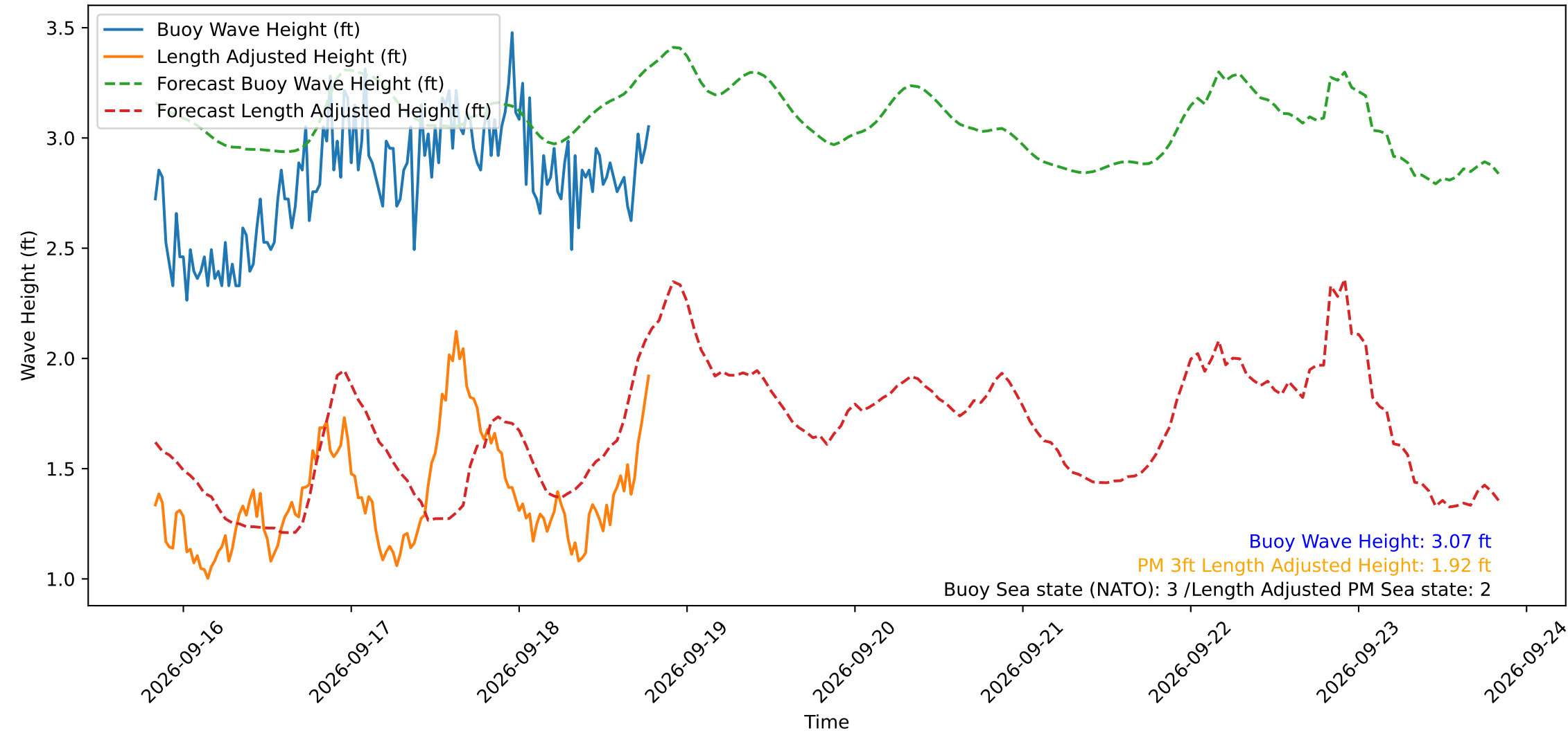
Wave Heights over Time for Green Beach at 2026-09-18 19:31:11
