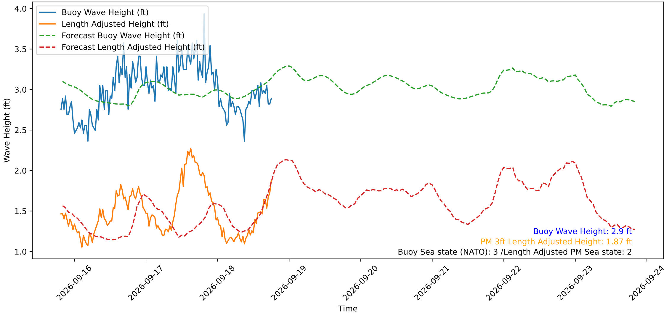
Wave Heights over Time for Oceanside Harbor at 2026-09-18 19:30:29
