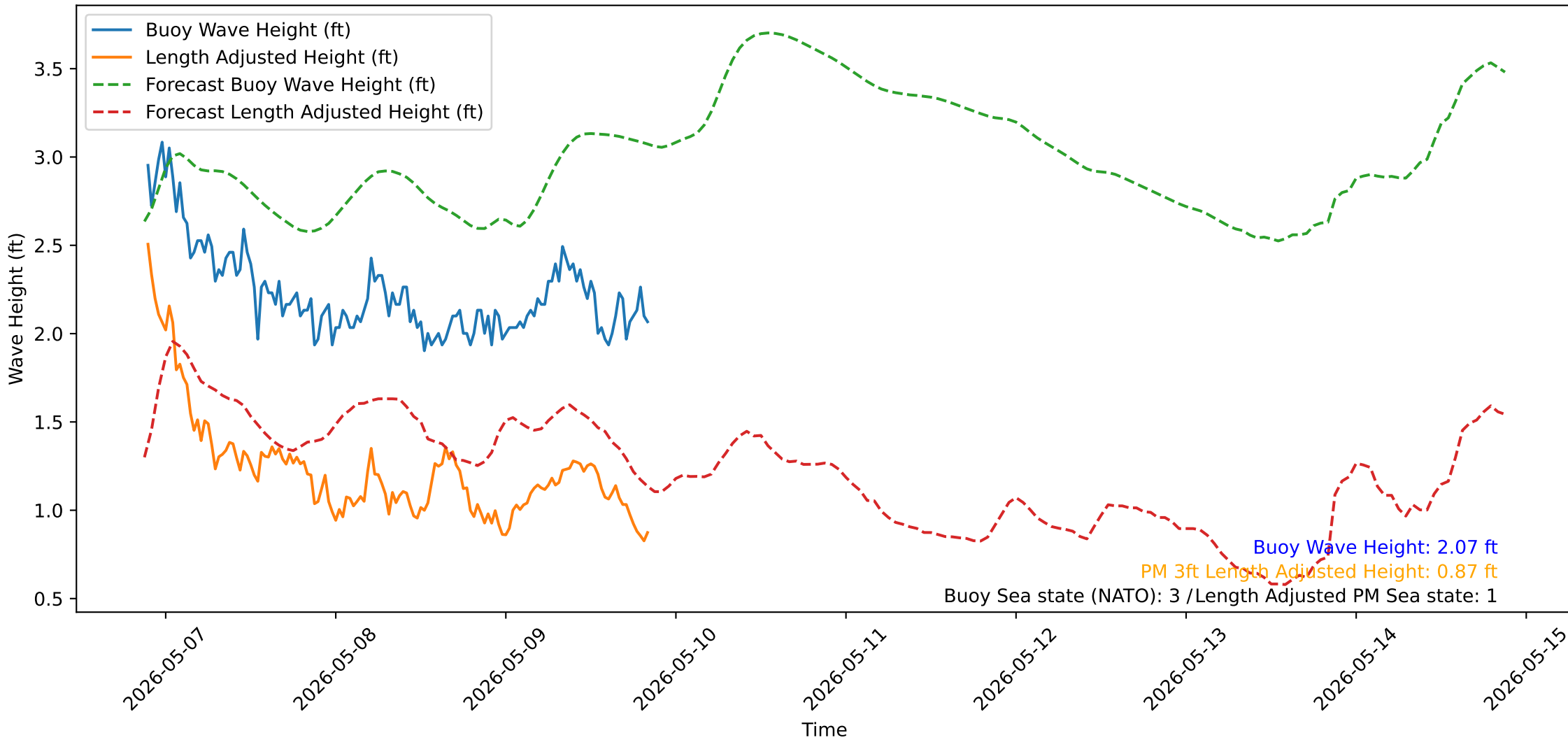
Wave Heights over Time for Red Beach at 2026-05-09 21:00:50
