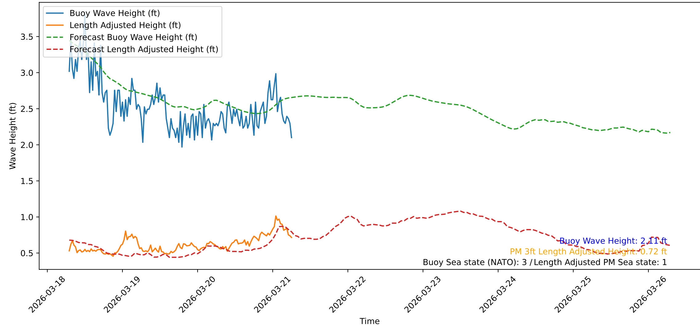
Wave Heights over Time for Oceanside Harbor at 2026-03-21 07:10:32
