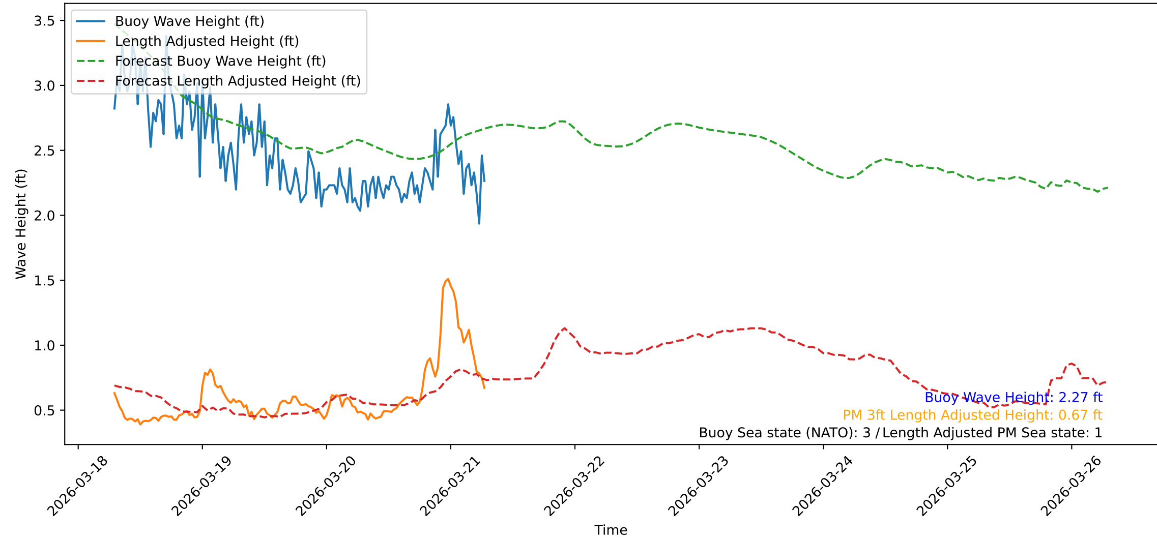
Wave Heights over Time for Green Beach at 2026-03-21 07:11:10
