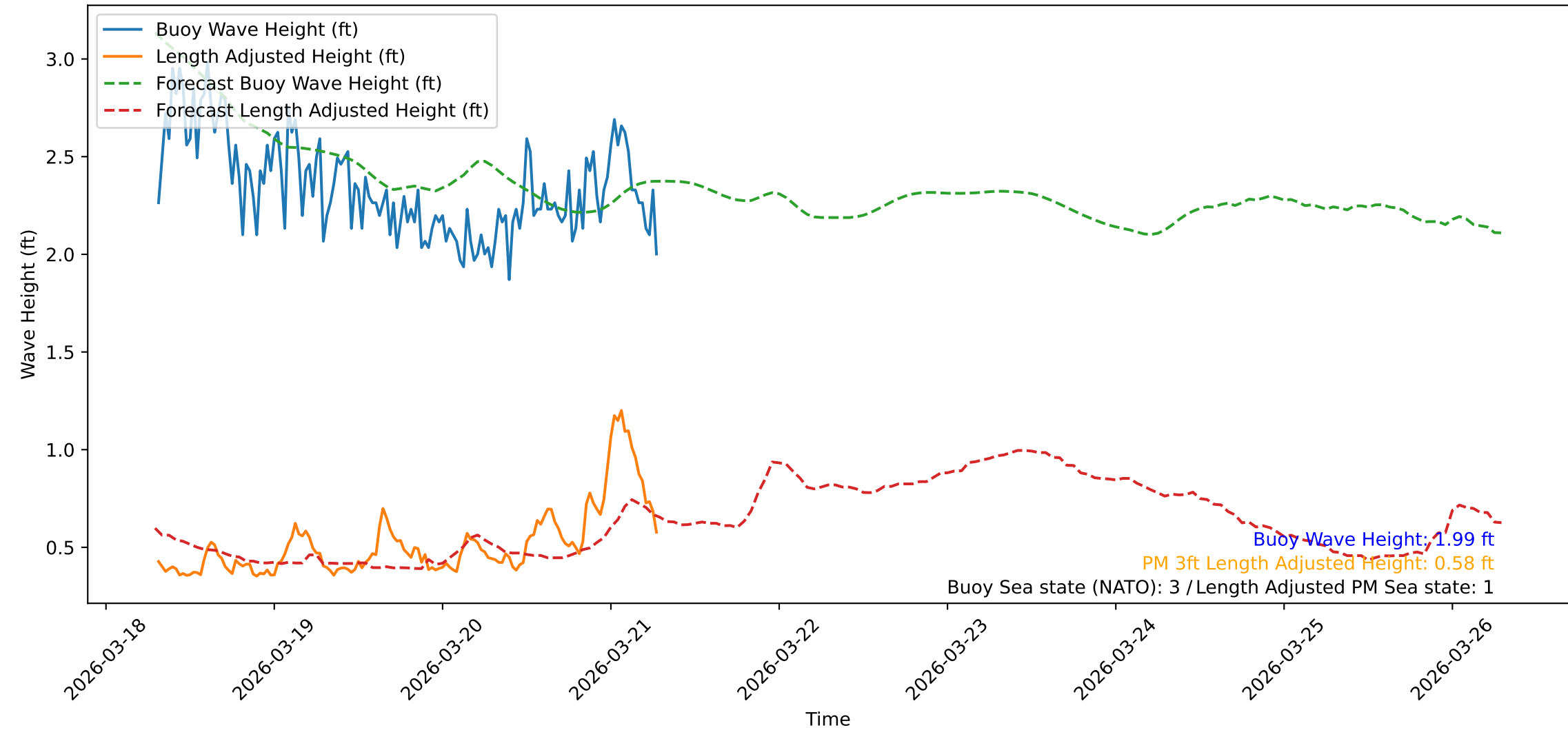
Wave Heights over Time for Red Beach at 2026-03-21 07:10:48
