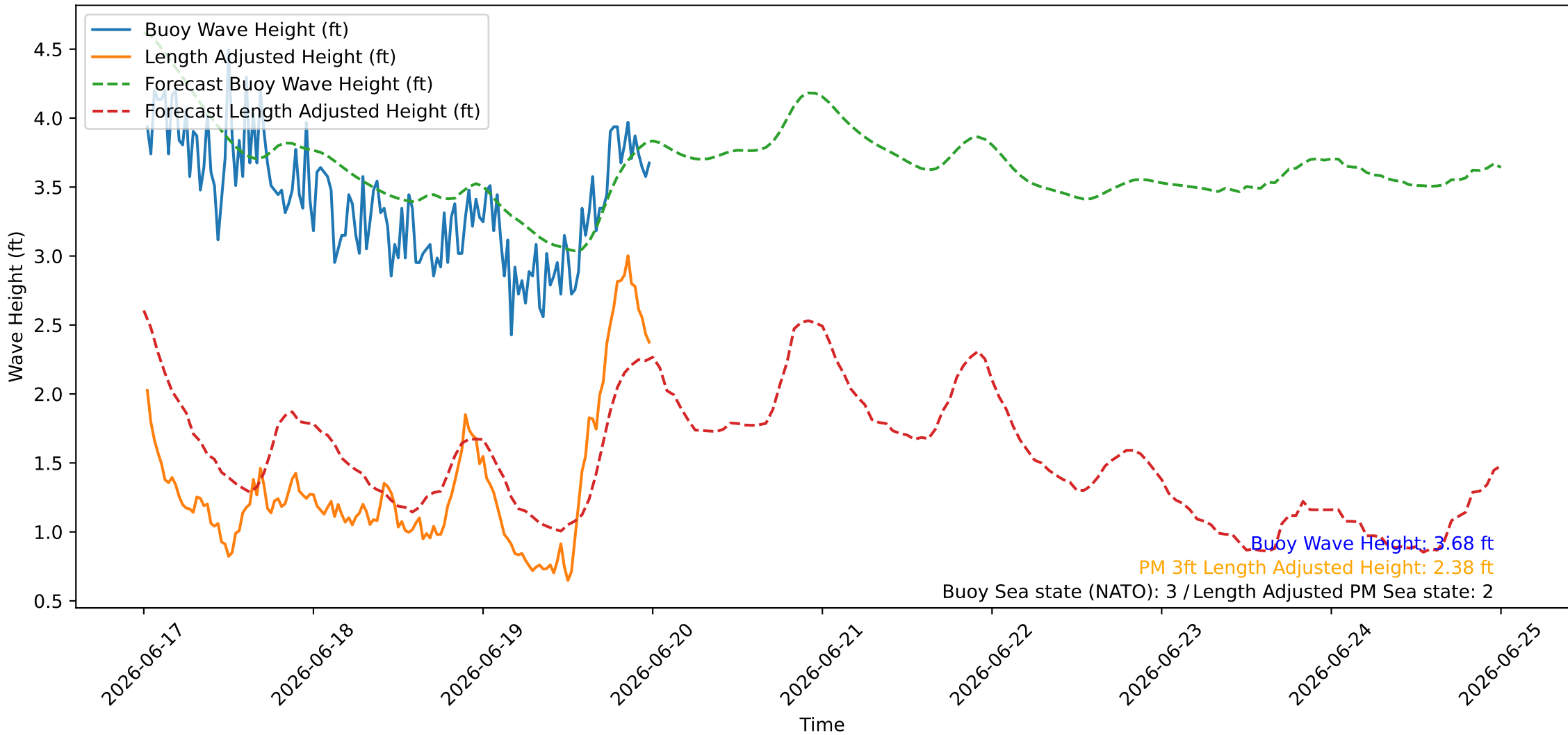
Wave Heights over Time for Green Beach at 2026-06-20 00:21:08
