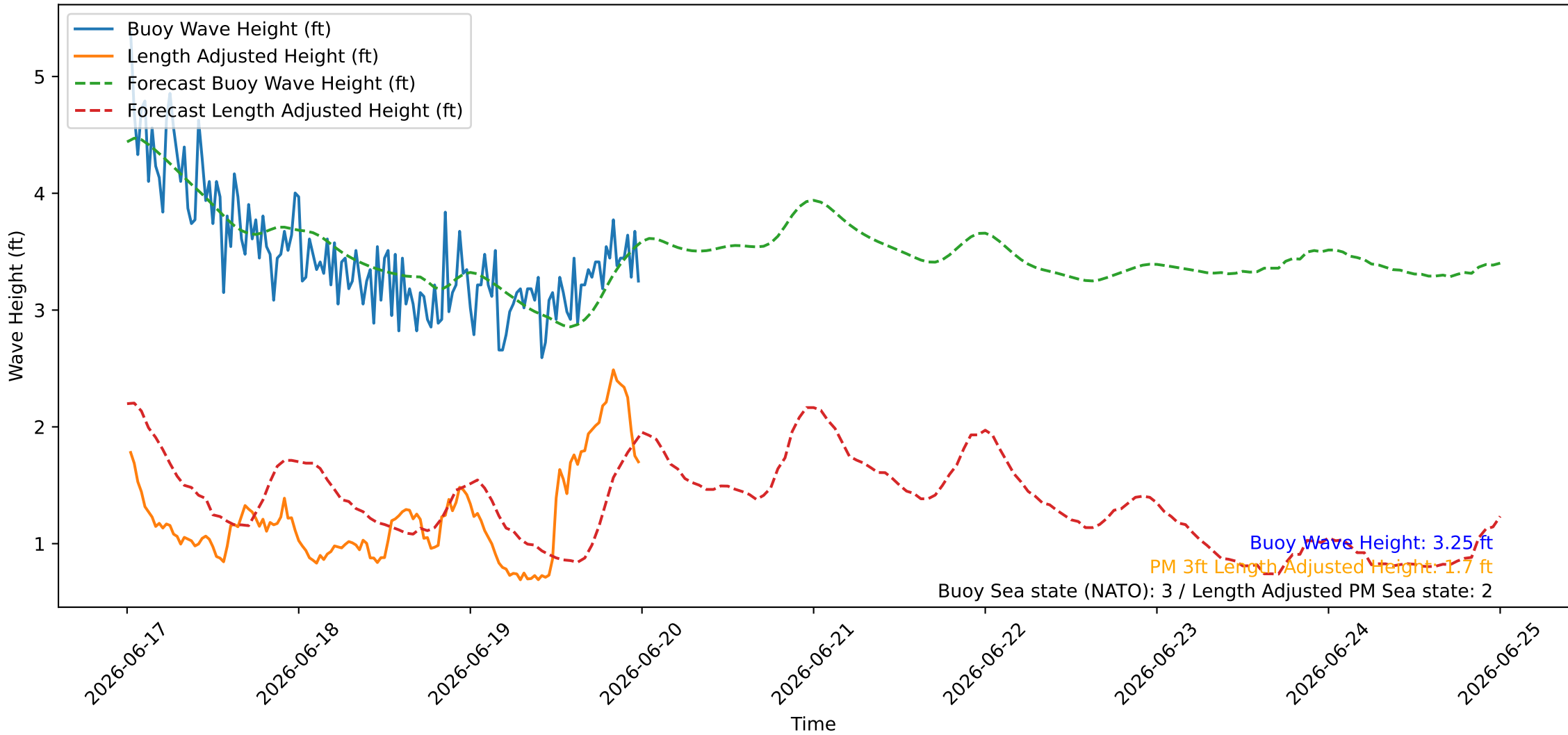
Wave Heights over Time for Red Beach at 2026-06-20 00:20:46
