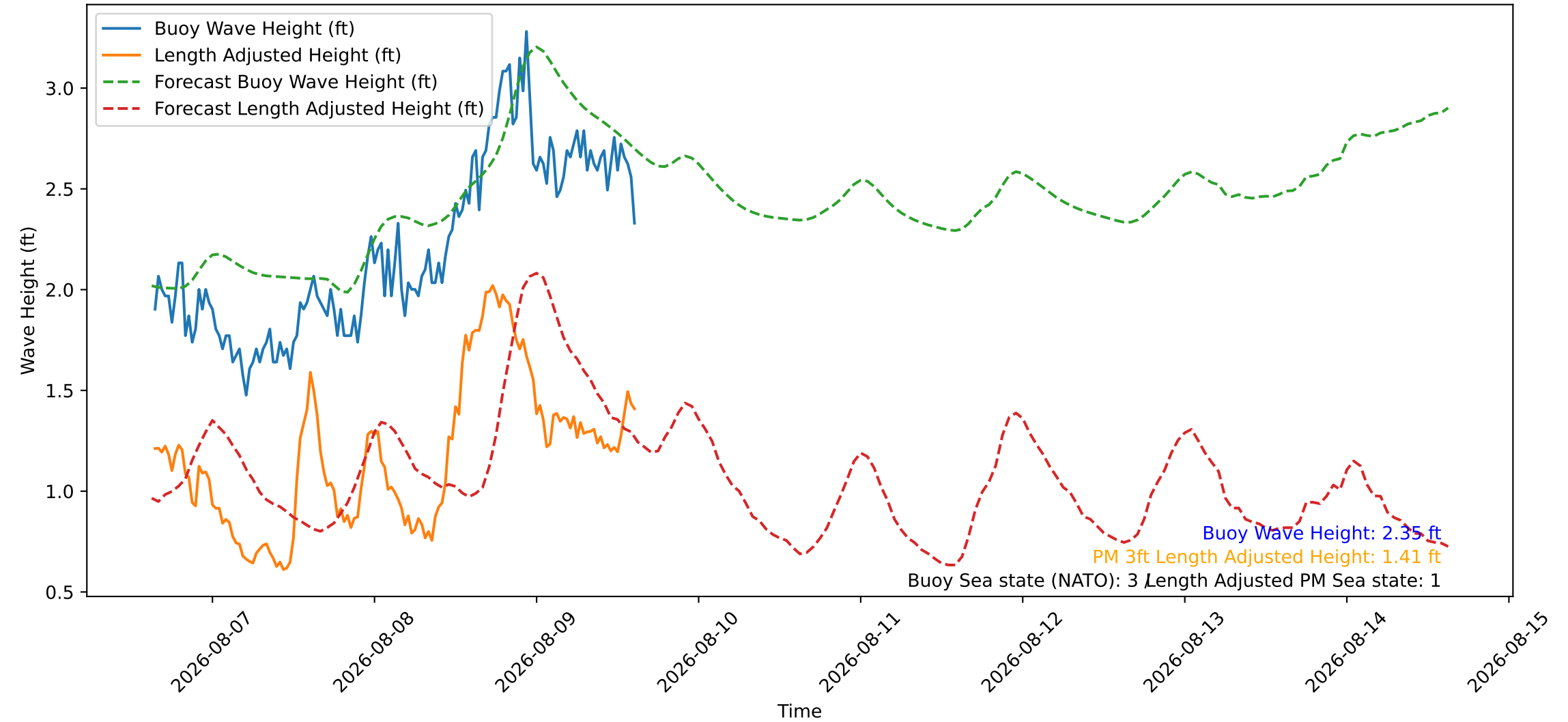
Wave Heights over Time for Red Beach at 2026-08-09 15:20:47
