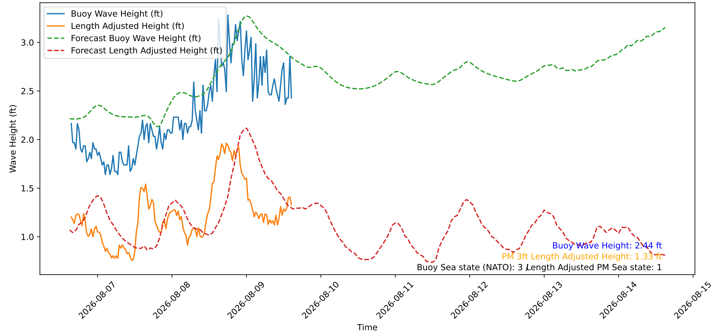
Wave Heights over Time for Oceanside Harbor at 2026-08-09 15:20:26
