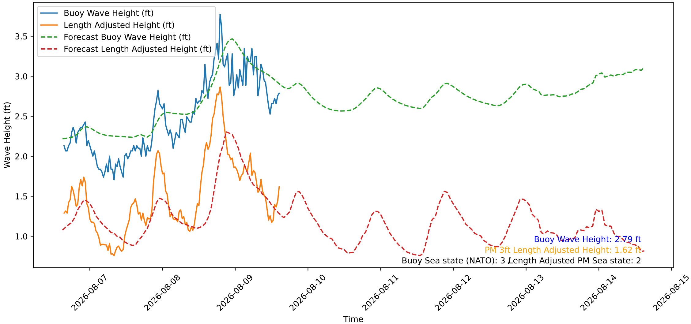
Wave Heights over Time for Green Beach at 2026-08-09 15:21:09
