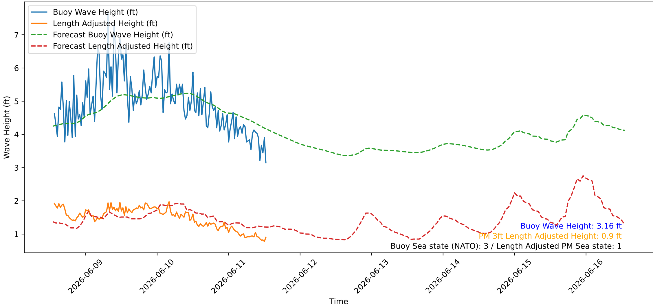
Wave Heights over Time for Red Beach at 2026-06-11 13:10:45
