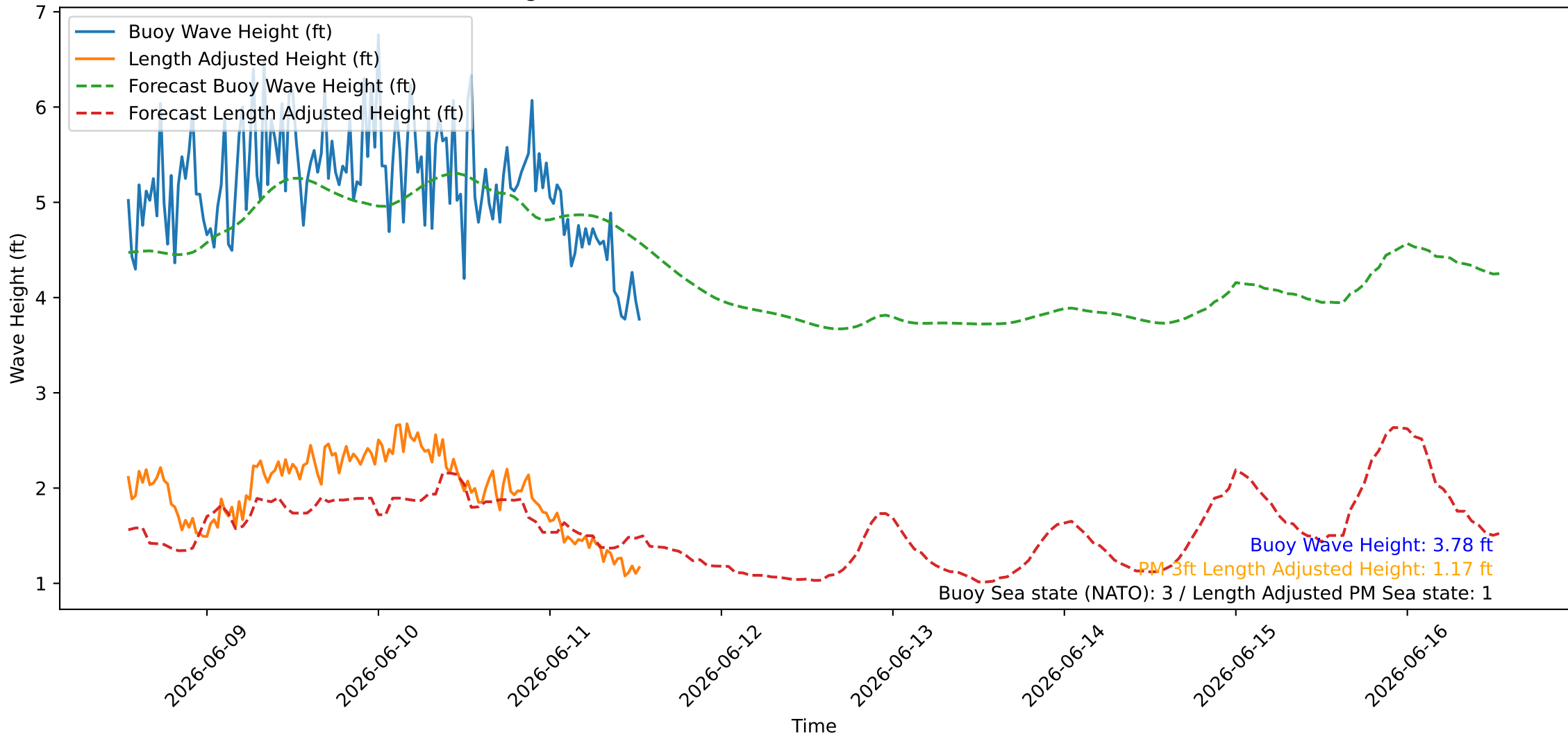
Wave Heights over Time for Oceanside Harbor at 2026-06-11 13:10:26
