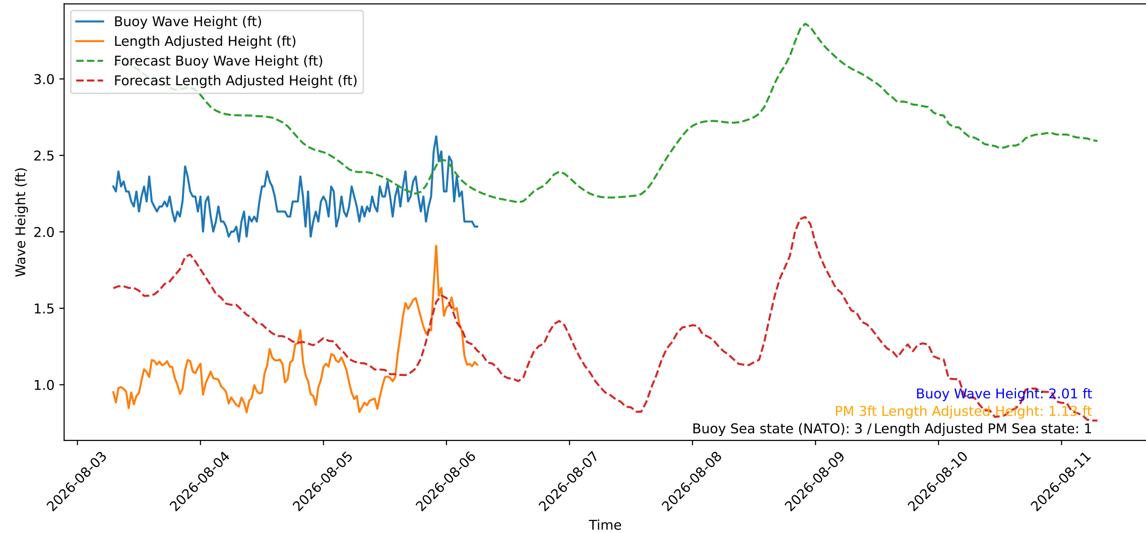
Wave Heights over Time for Green Beach at 2026-08-06 07:01:07
