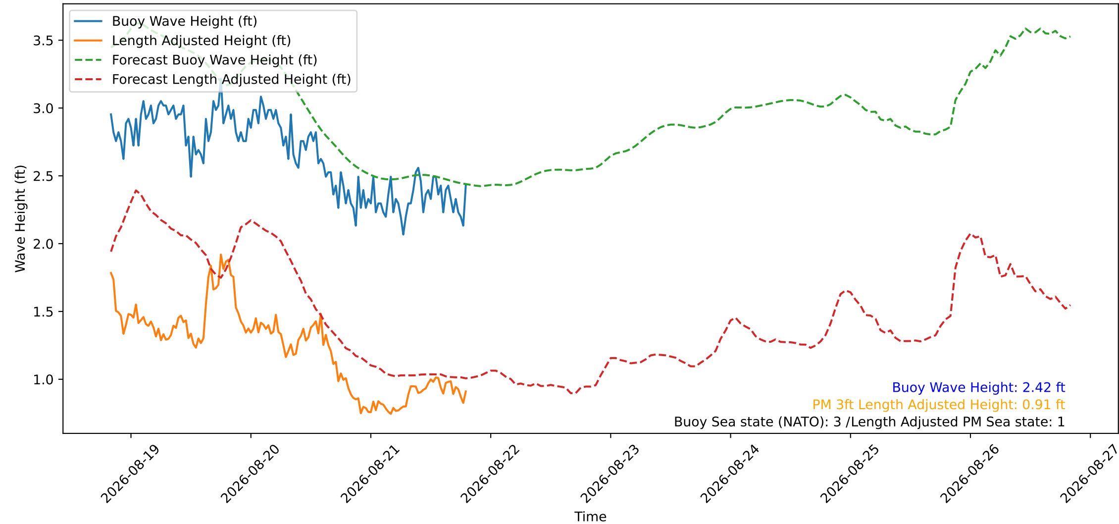
Wave Heights over Time for Red Beach at 2026-08-21 19:50:46
