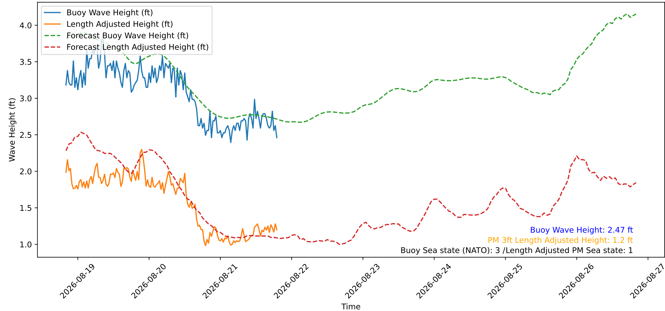
Wave Heights over Time for Oceanside Harbor at 2026-08-21 19:50:26
