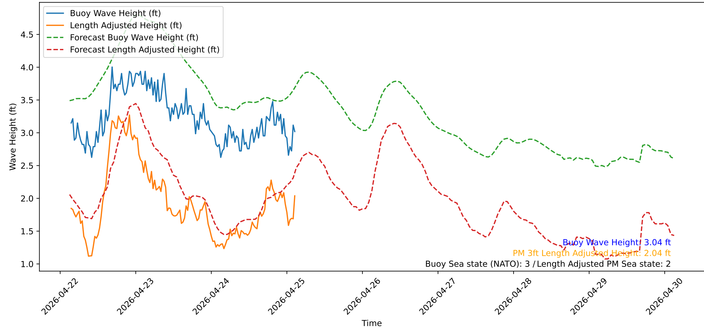
Wave Heights over Time for Green Beach at 2026-04-25 03:21:13
