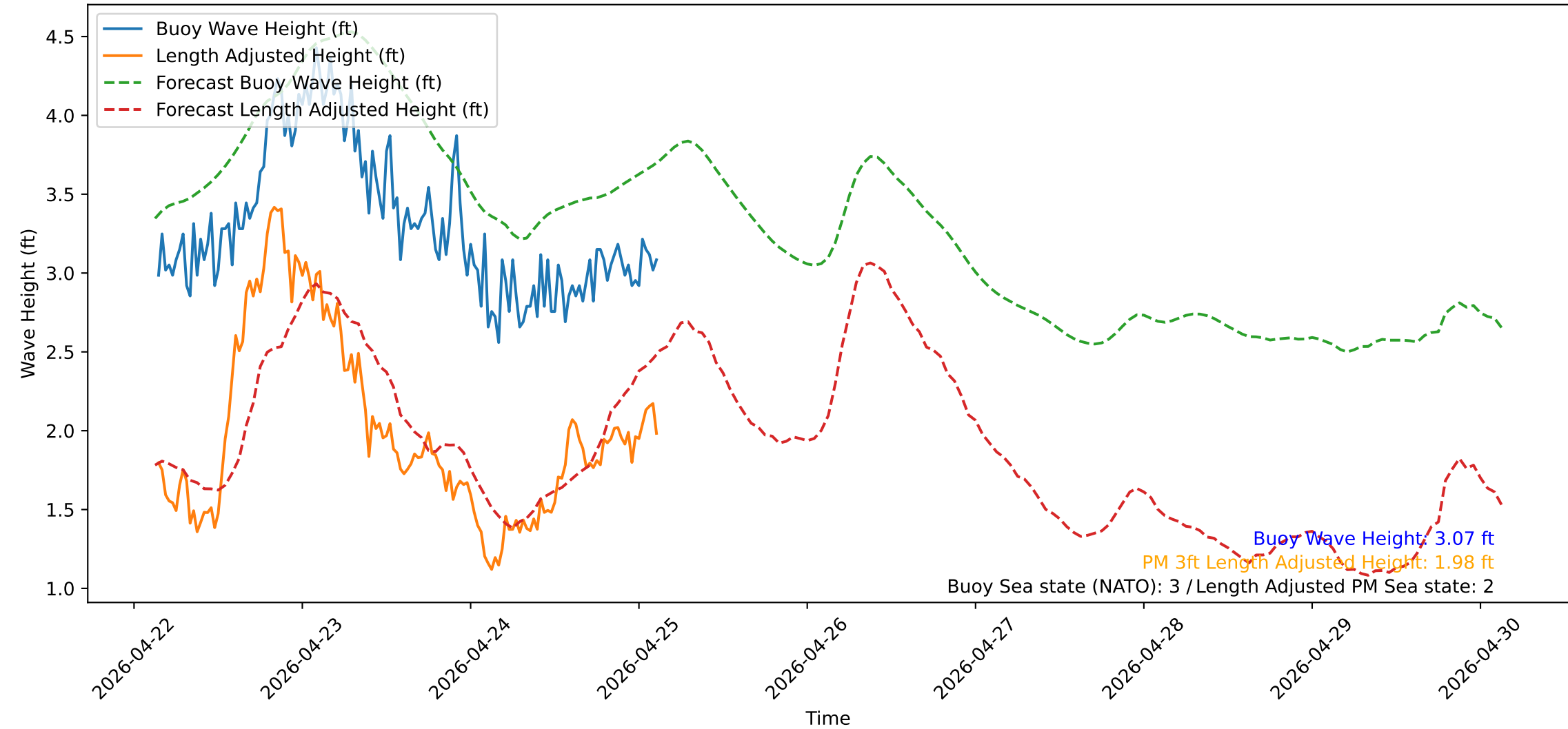
Wave Heights over Time for Oceanside Harbor at 2026-04-25 03:20:30
