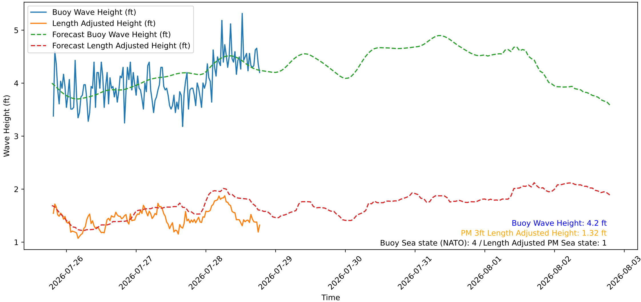
Wave Heights over Time for Oceanside Harbor at 2026-07-28 19:20:26
