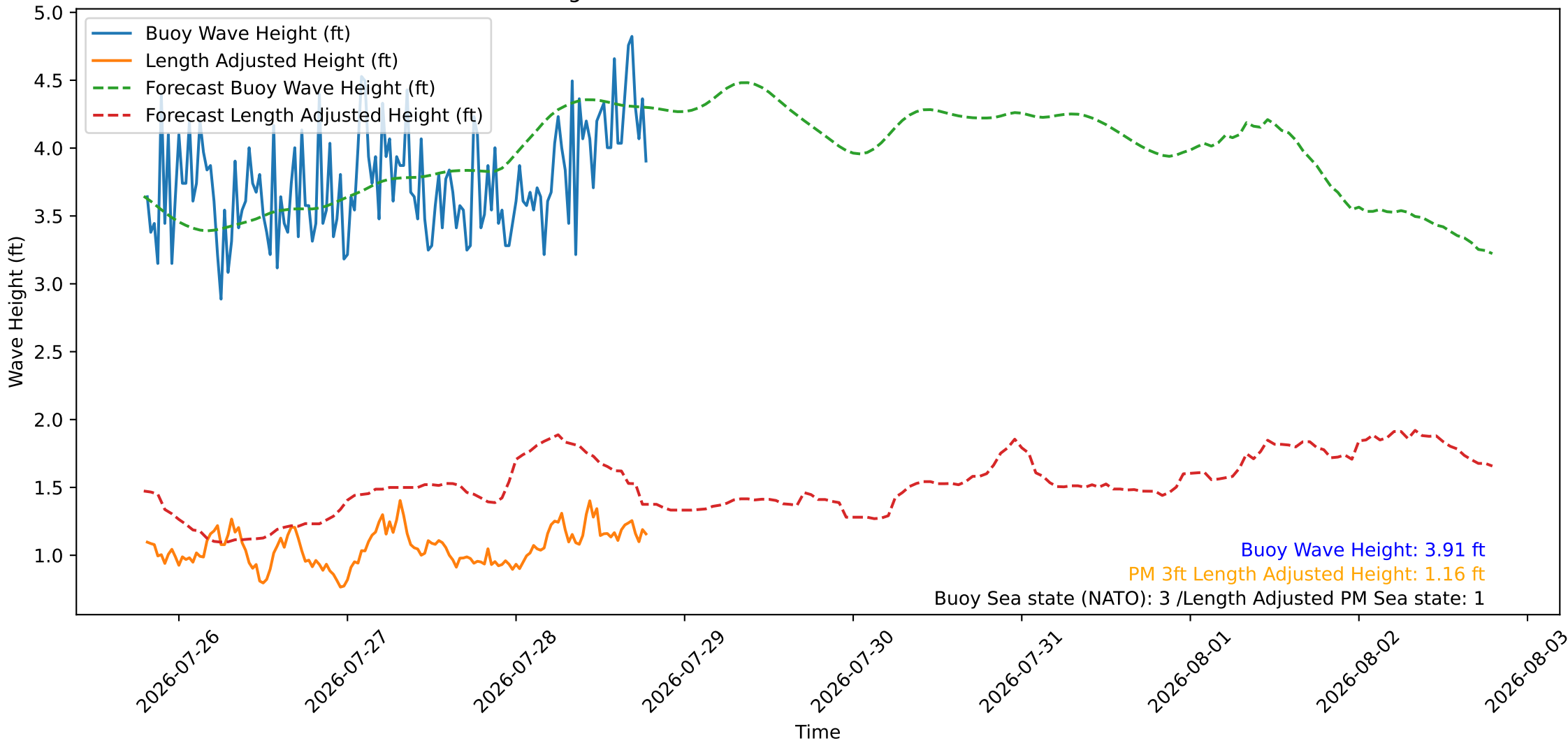
Wave Heights over Time for Red Beach at 2026-07-28 19:20:47
