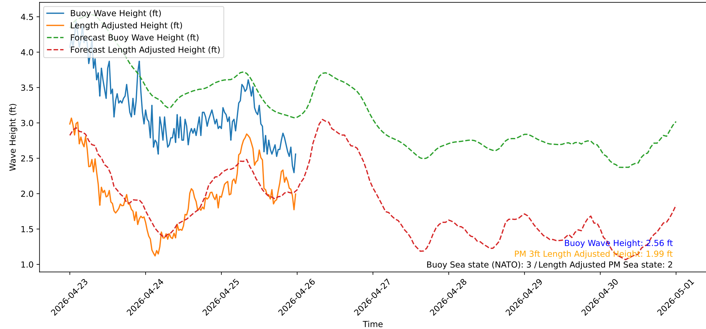
Wave Heights over Time for Oceanside Harbor at 2026-04-26 00:10:31
