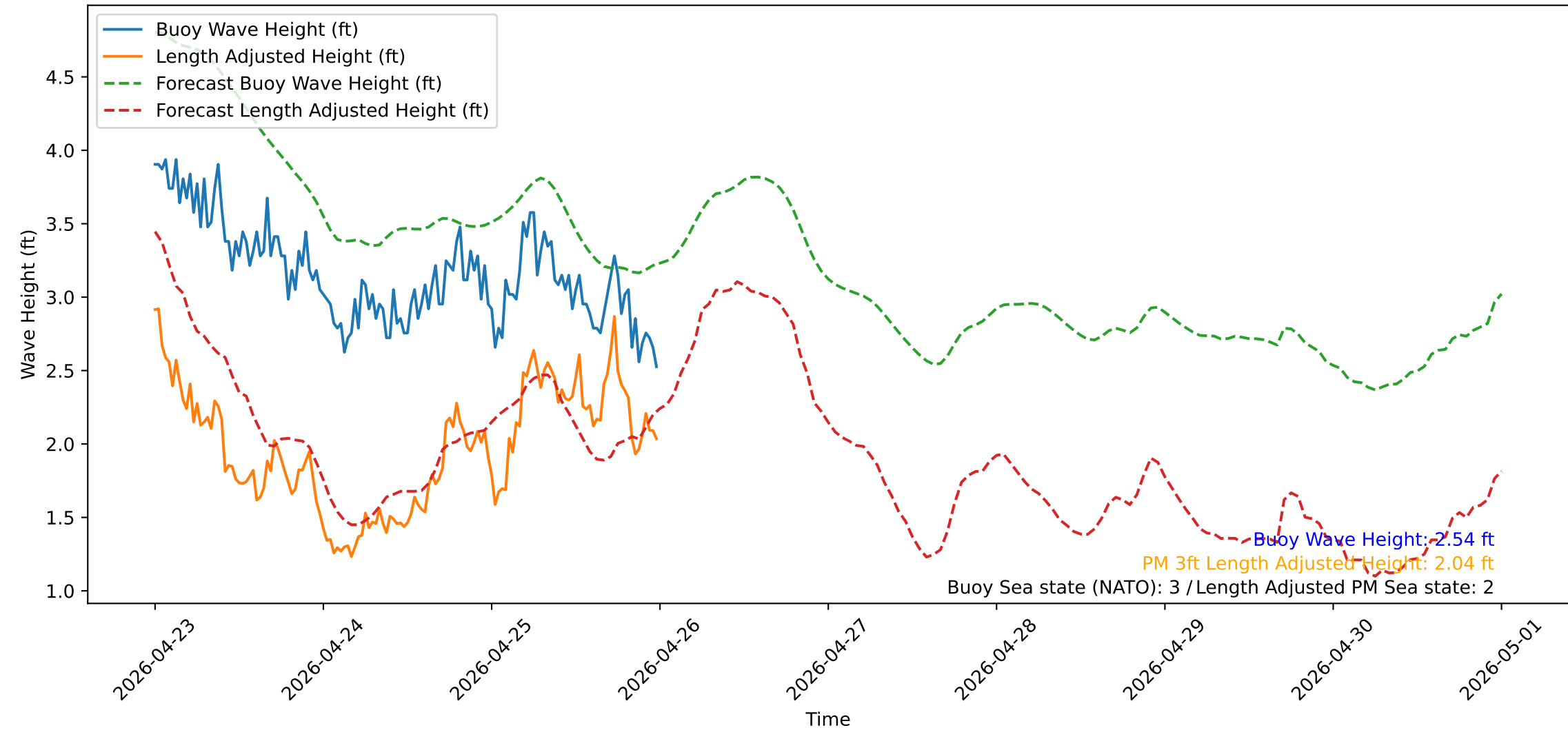
Wave Heights over Time for Green Beach at 2026-04-26 00:11:12
