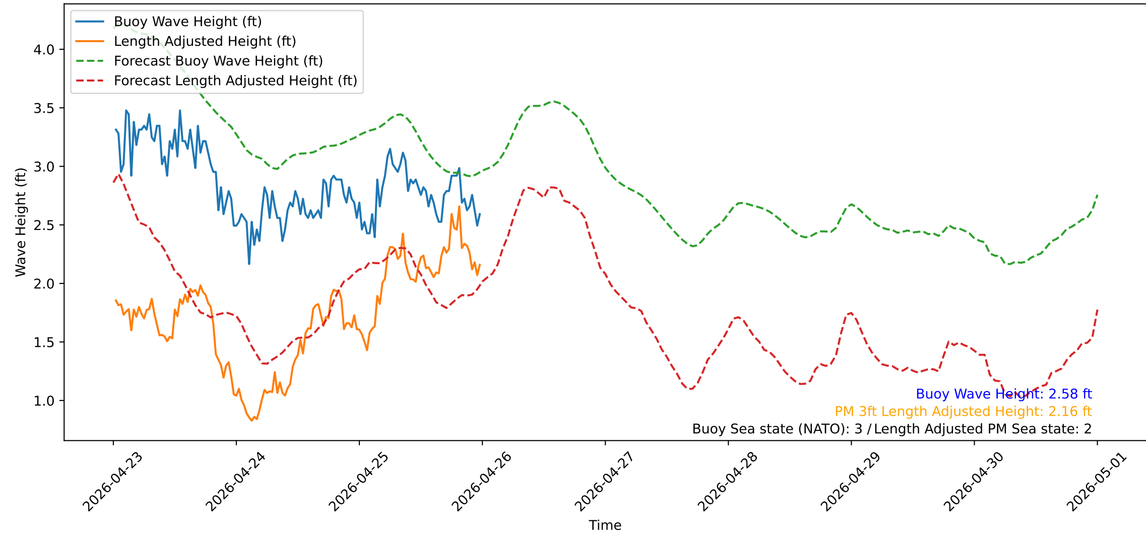
Wave Heights over Time for Red Beach at 2026-04-26 00:10:50
