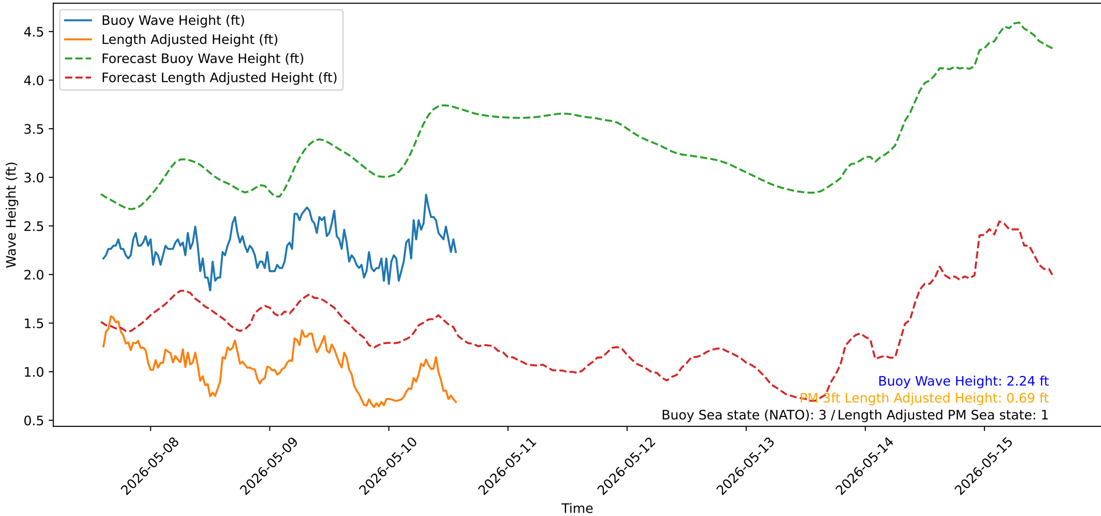
Wave Heights over Time for Green Beach at 2026-05-10 14:21:16
