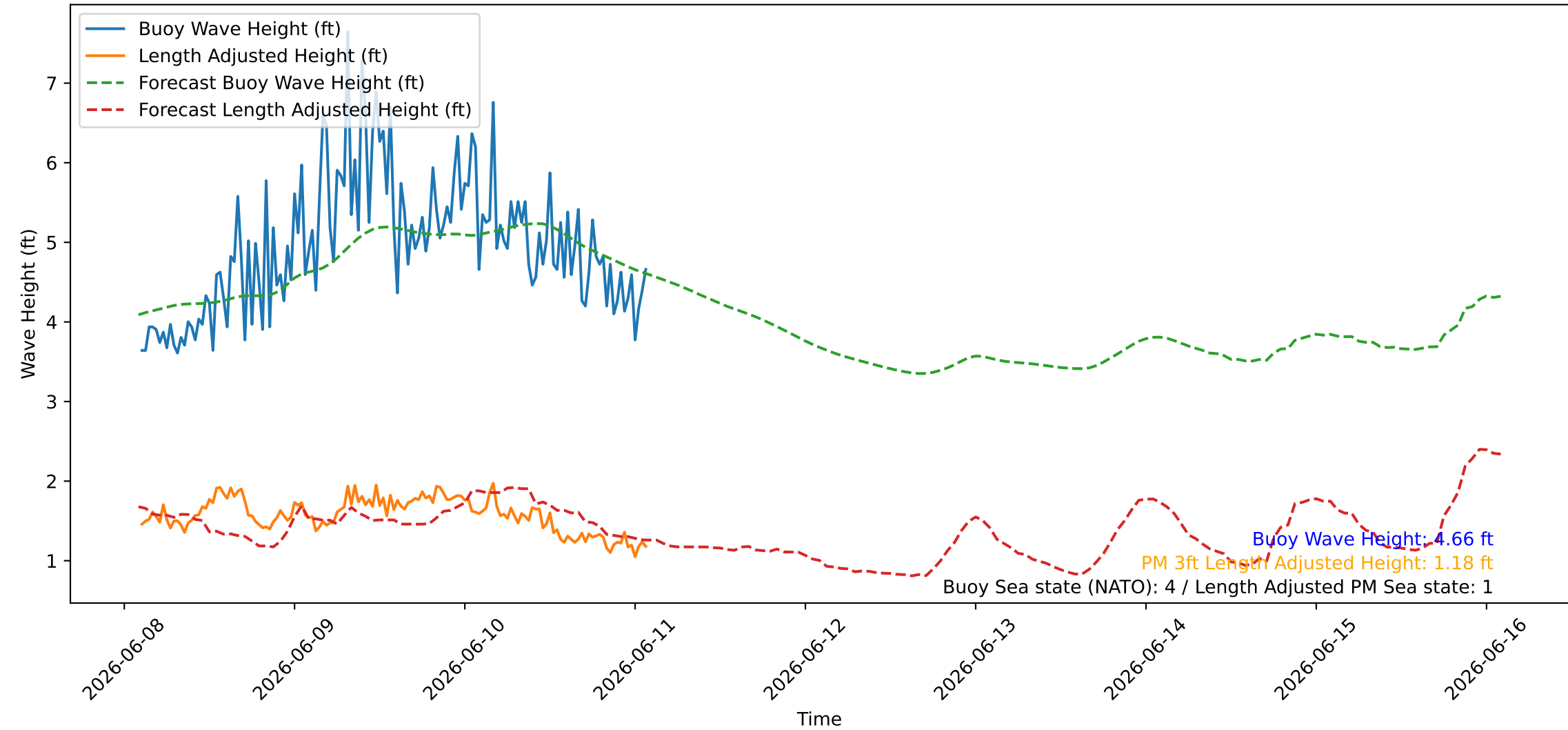
Wave Heights over Time for Red Beach at 2026-06-11 02:10:47
