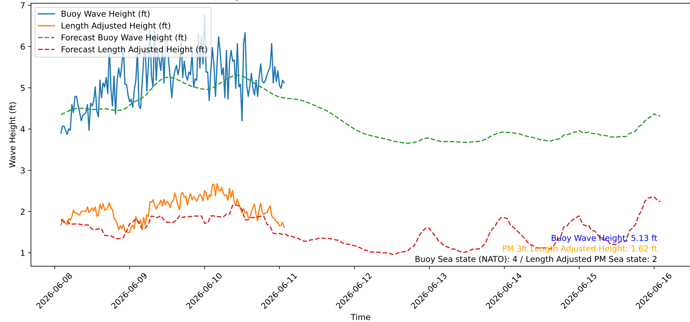
Wave Heights over Time for Oceanside Harbor at 2026-06-11 02:10:27
