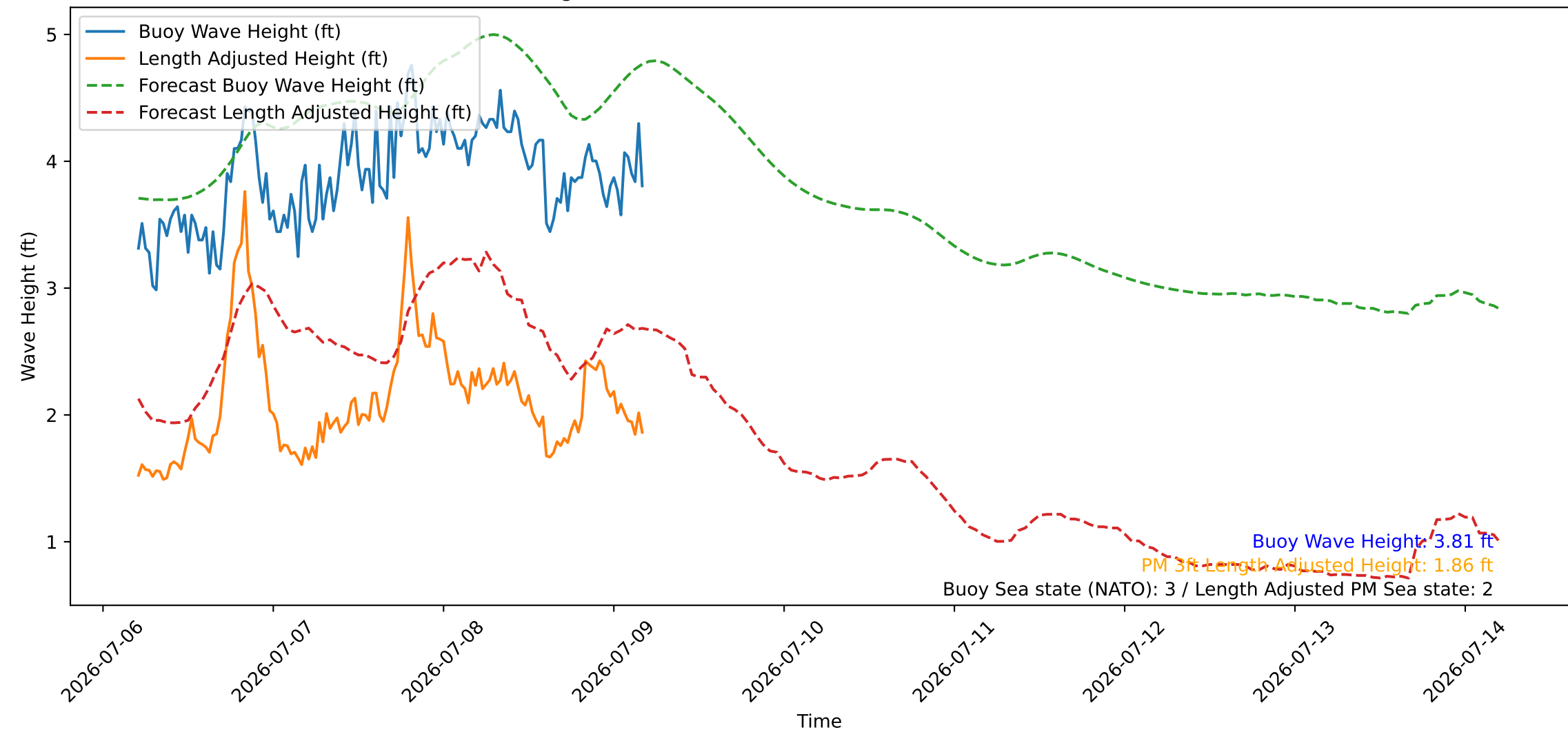
Wave Heights over Time for Green Beach at 2026-07-09 05:01:09
