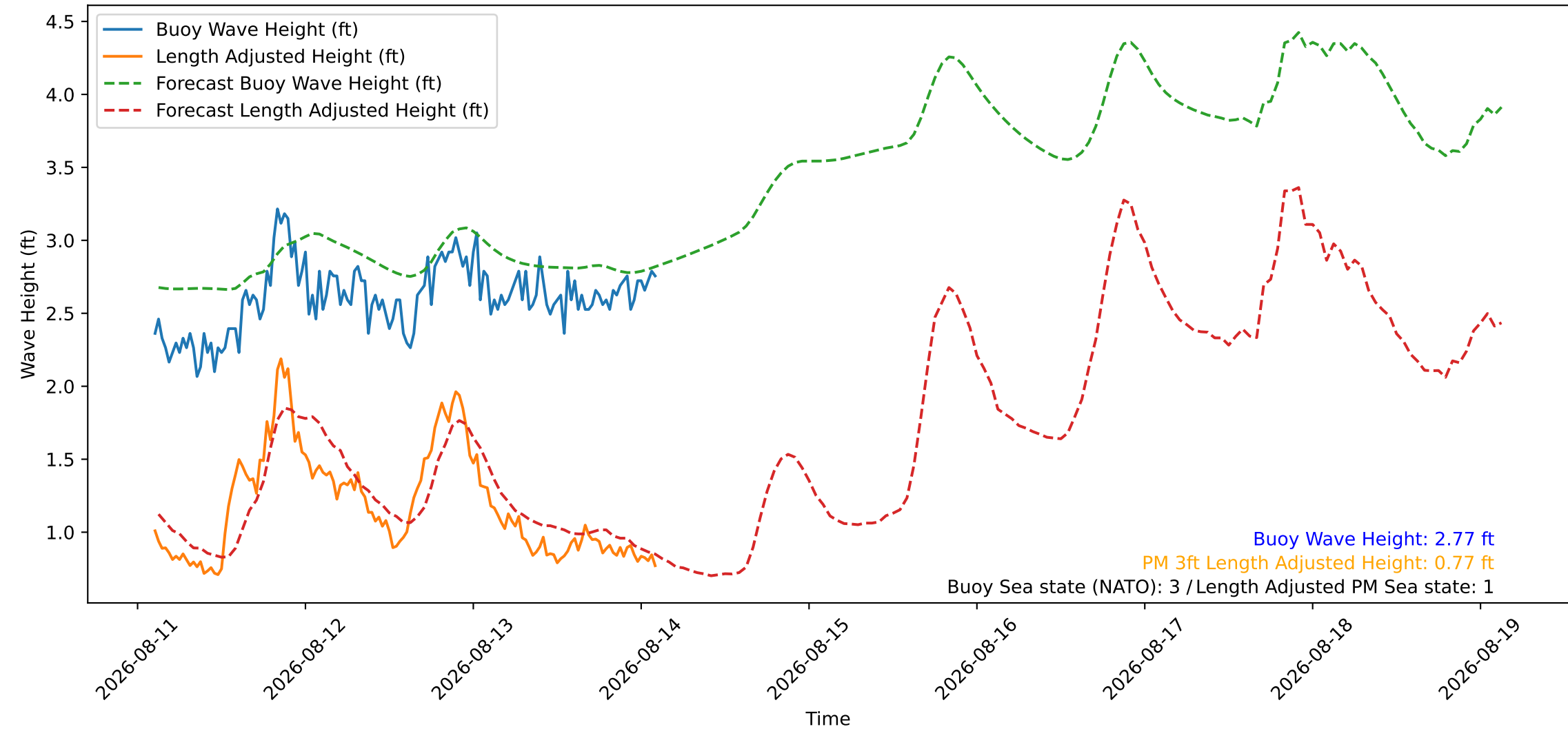
Wave Heights over Time for Green Beach at 2026-08-14 02:41:08
