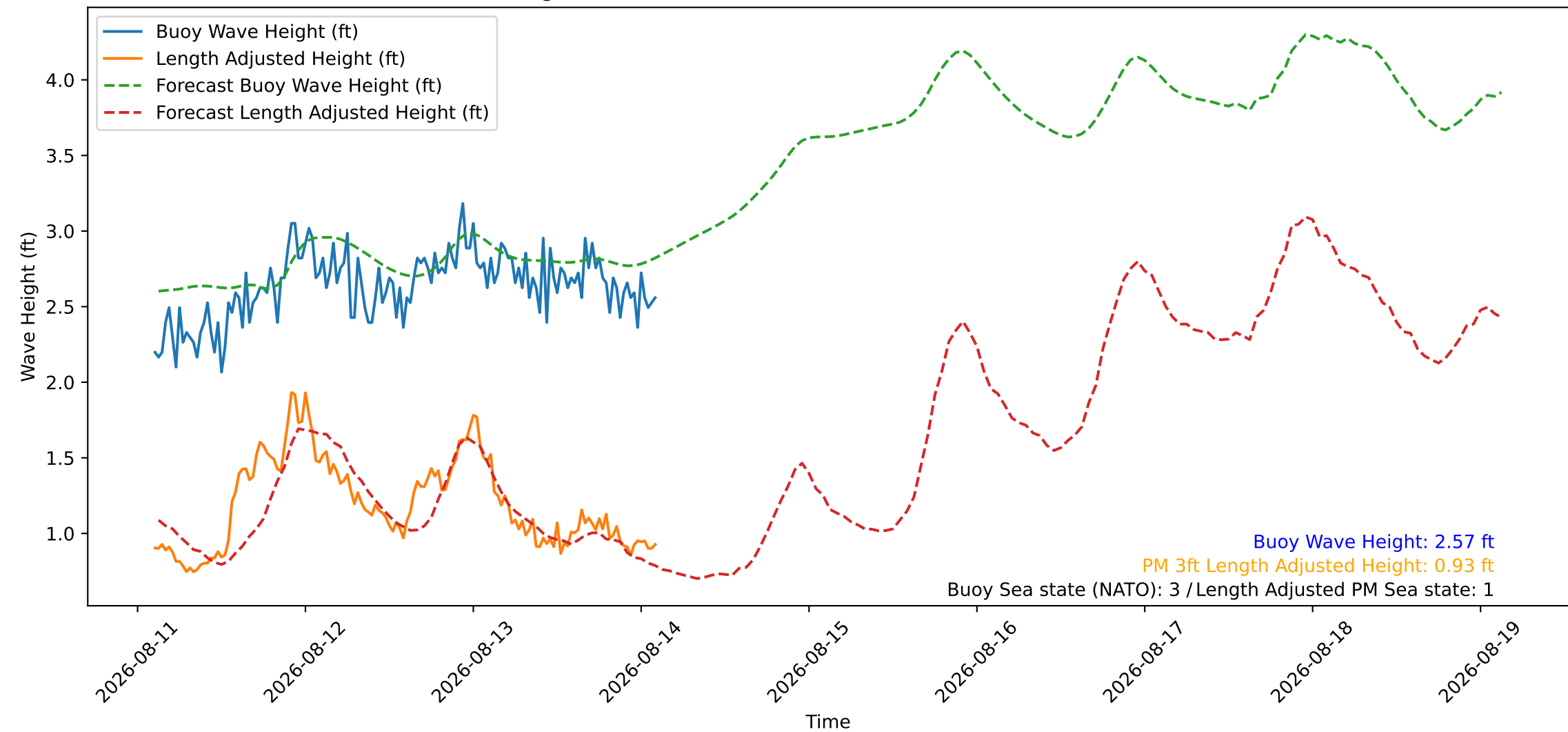
Wave Heights over Time for Oceanside Harbor at 2026-08-14 02:40:26
