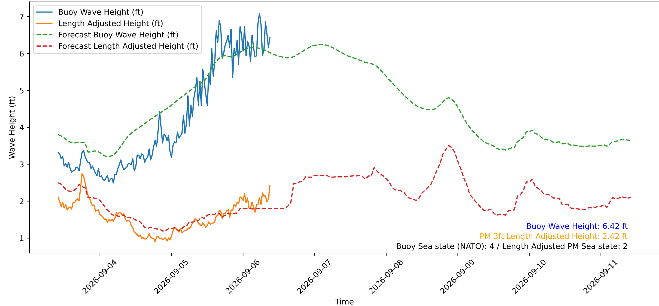
Wave Heights over Time for Green Beach at 2026-09-06 09:41:13
