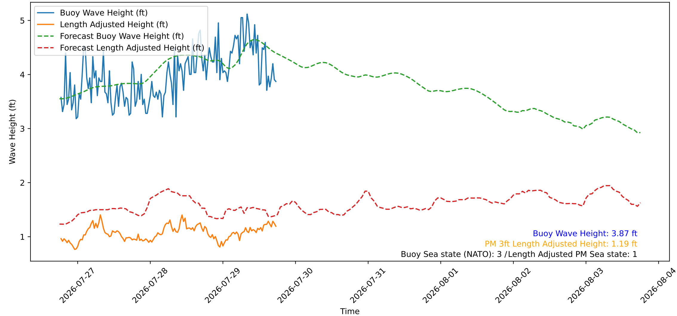
Wave Heights over Time for Red Beach at 2026-07-29 18:10:45
