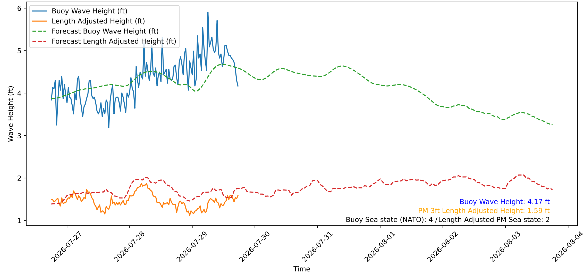
Wave Heights over Time for Oceanside Harbor at 2026-07-29 18:10:26
