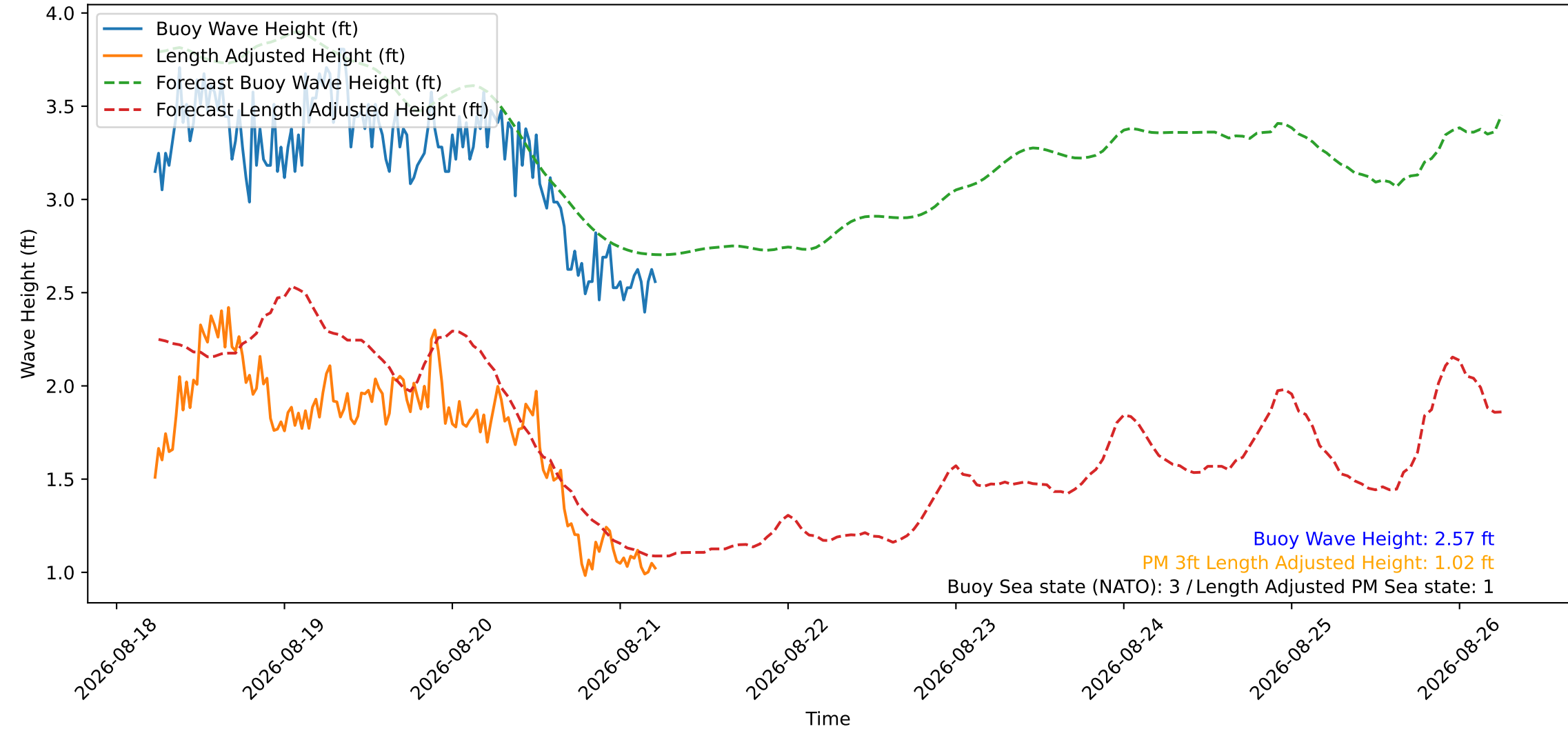
Wave Heights over Time for Oceanside Harbor at 2026-08-21 05:40:26
