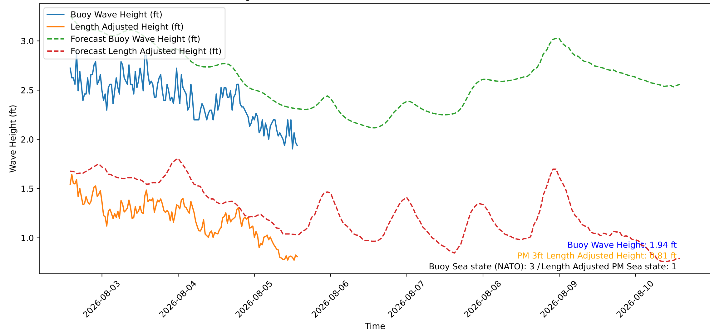
Wave Heights over Time for Oceanside Harbor at 2026-08-05 14:10:26
