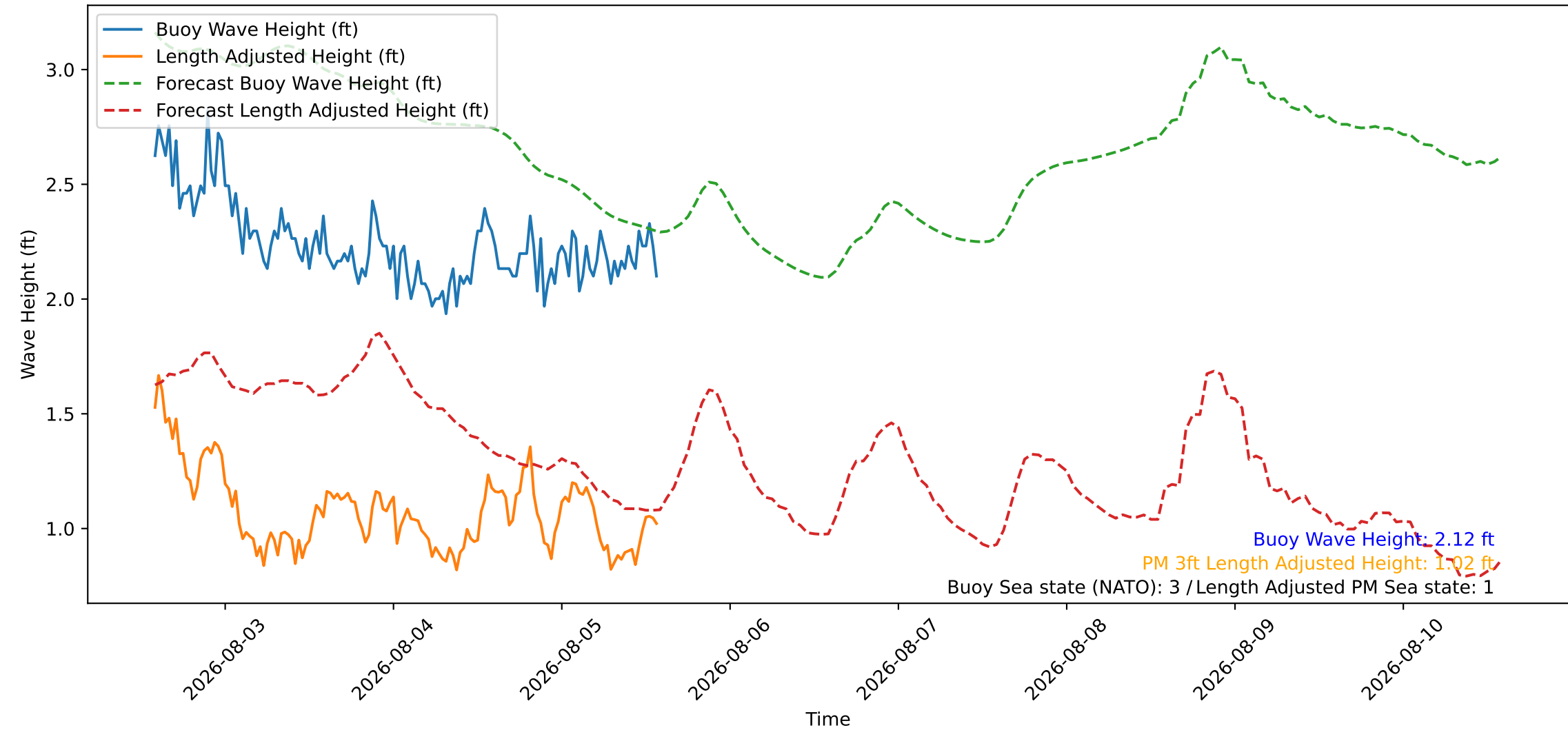
Wave Heights over Time for Green Beach at 2026-08-05 14:11:08
