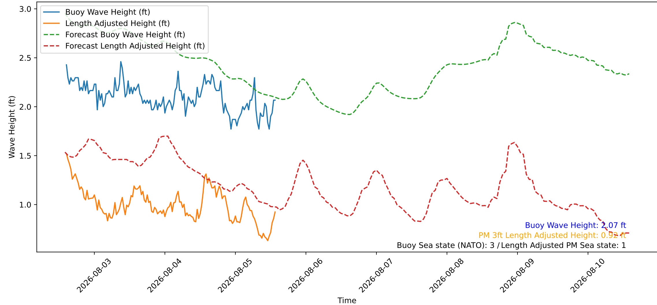
Wave Heights over Time for Red Beach at 2026-08-05 14:10:46
