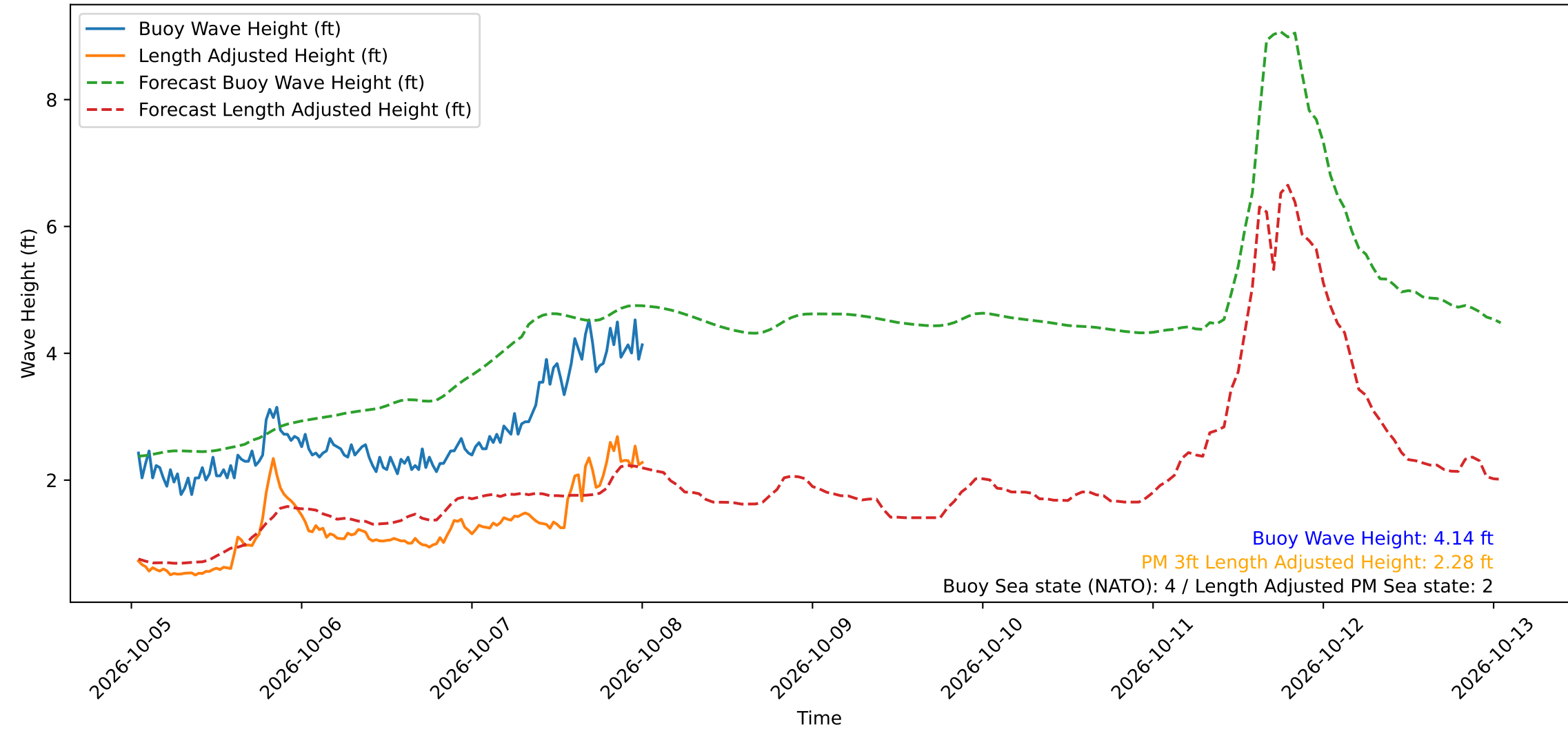
Wave Heights over Time for Green Beach at 2026-10-08 00:51:13
