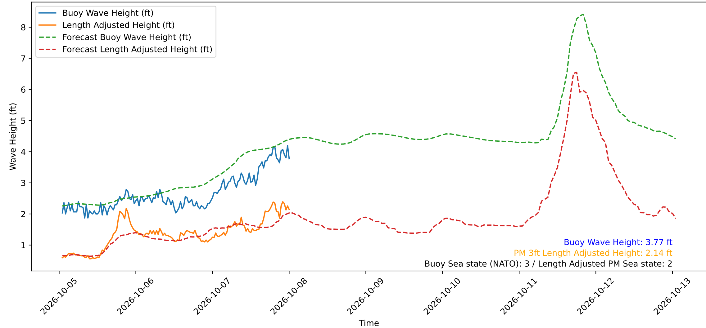
Wave Heights over Time for Oceanside Harbor at 2026-10-08 00:50:29
