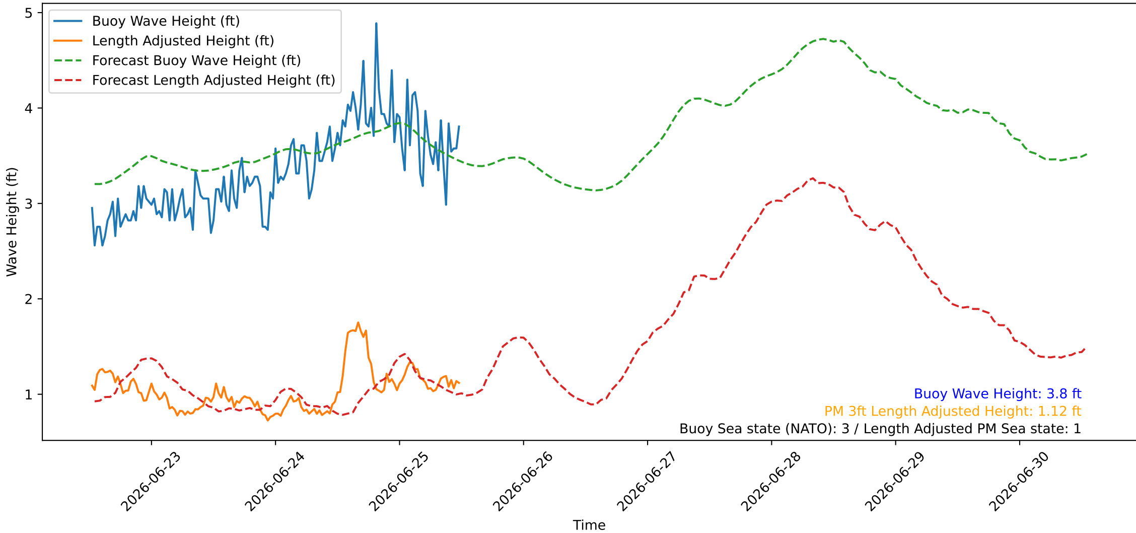
Wave Heights over Time for Oceanside Harbor at 2026-06-25 12:40:25
