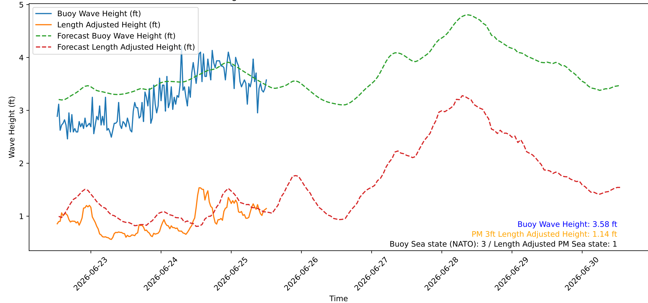
Wave Heights over Time for Green Beach at 2026-06-25 12:41:07
