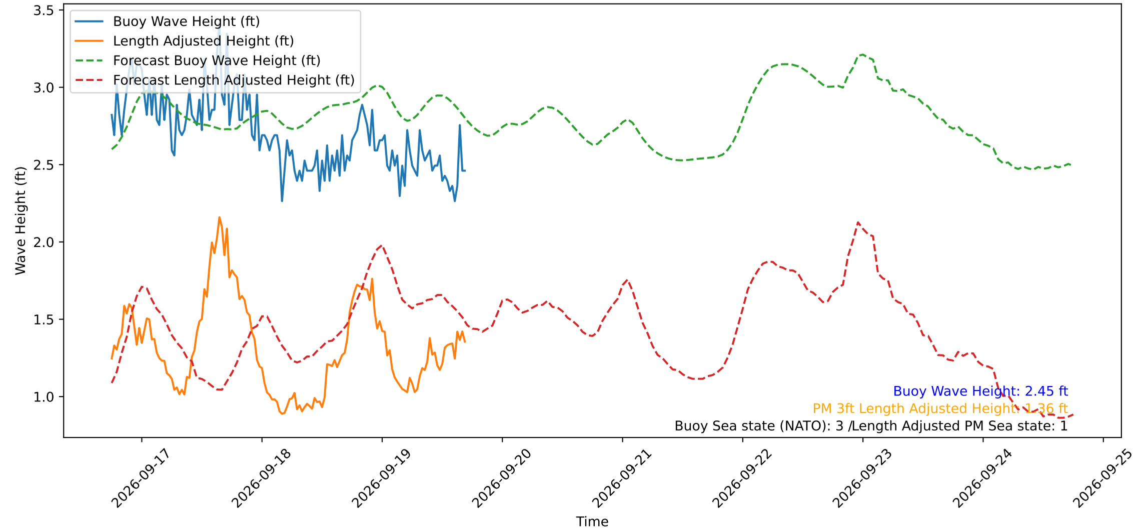
Wave Heights over Time for Red Beach at 2026-09-19 17:30:49
