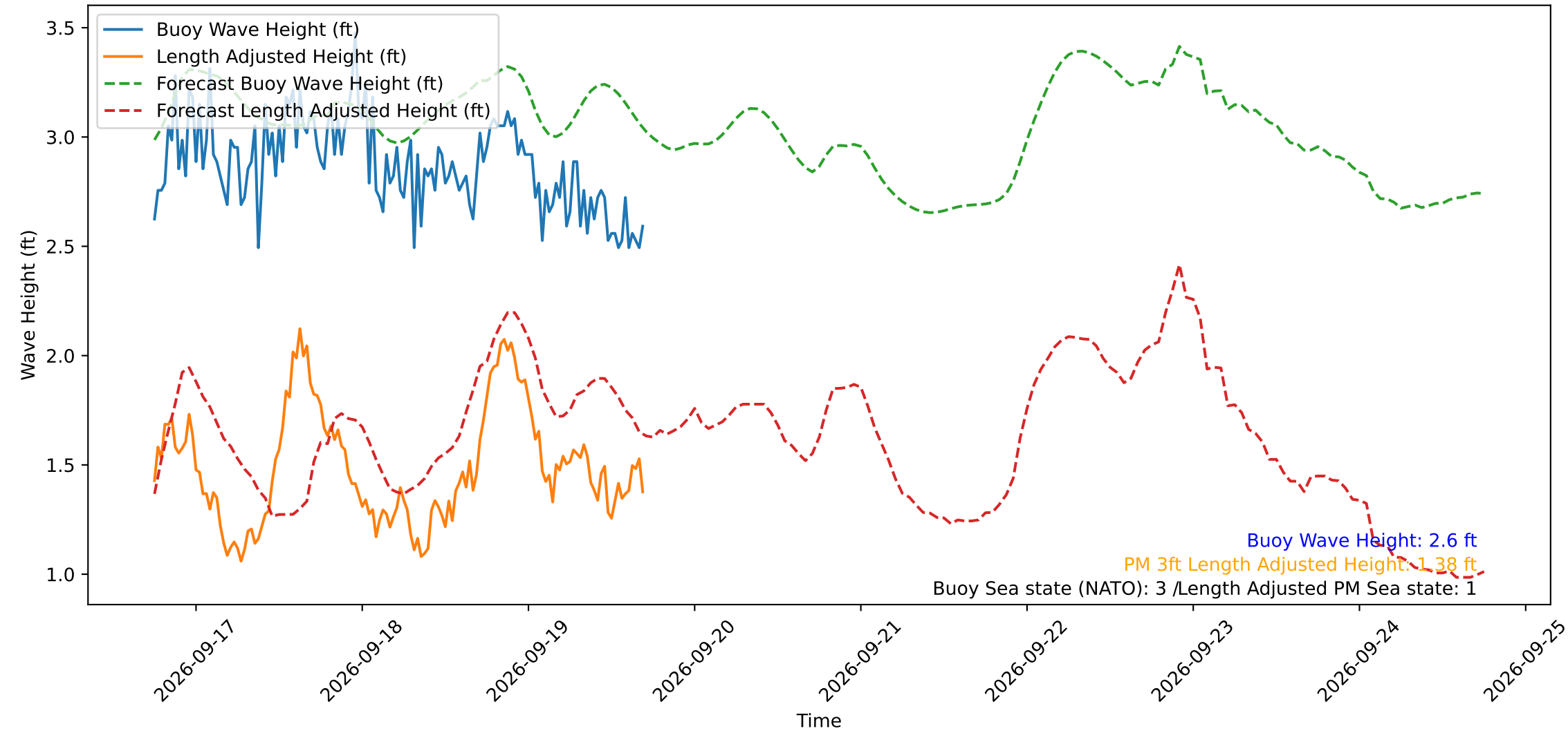
Wave Heights over Time for Green Beach at 2026-09-19 17:31:11
