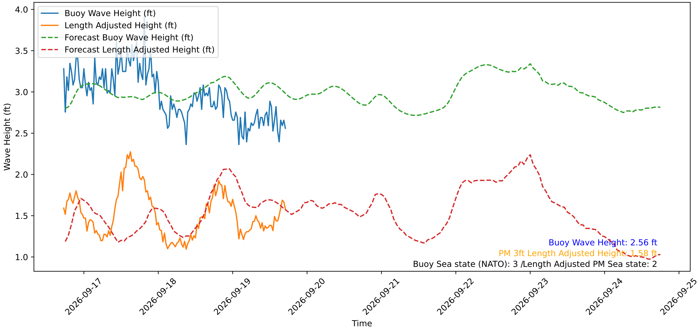
Wave Heights over Time for Oceanside Harbor at 2026-09-19 17:30:29
