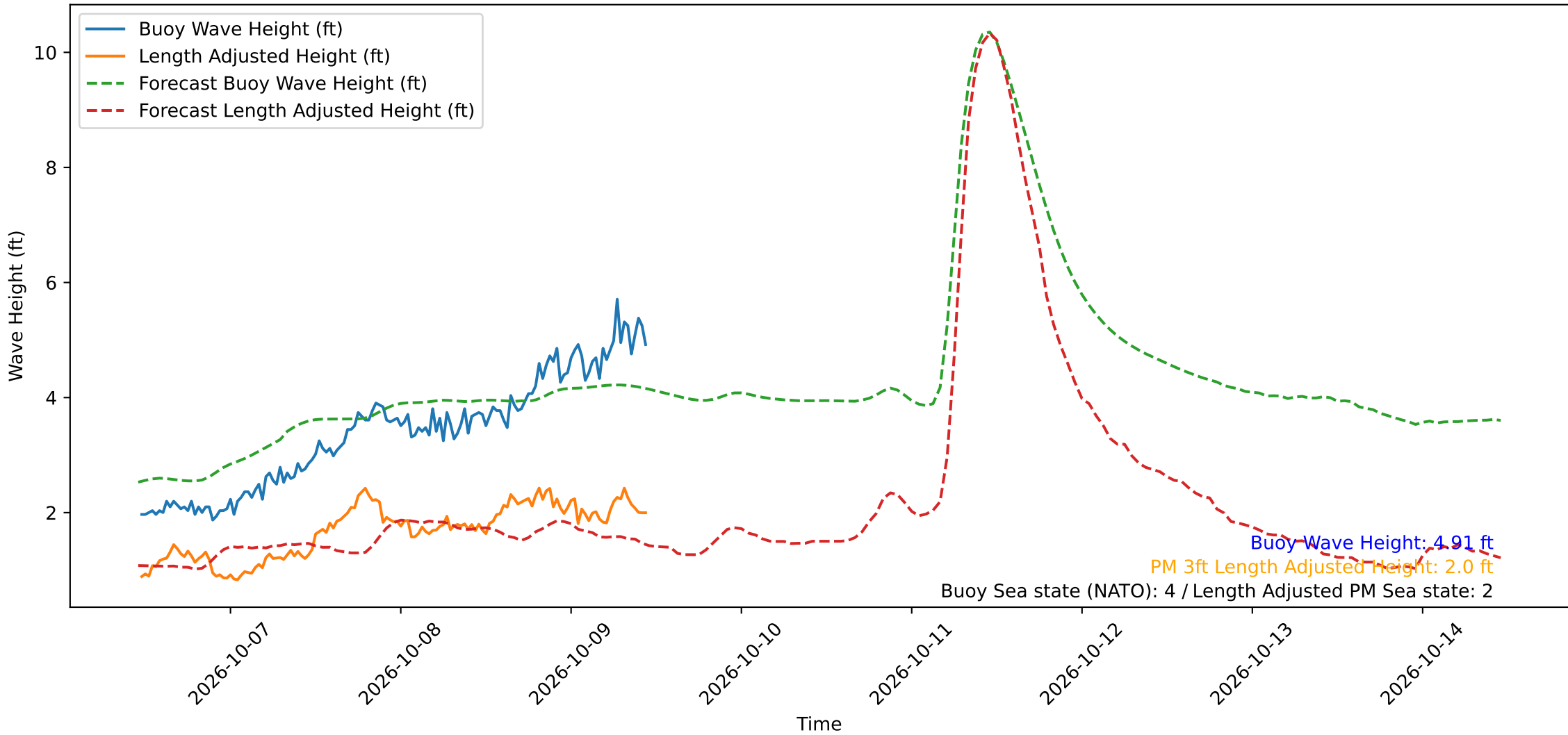
Wave Heights over Time for Red Beach at 2026-10-09 11:20:50
