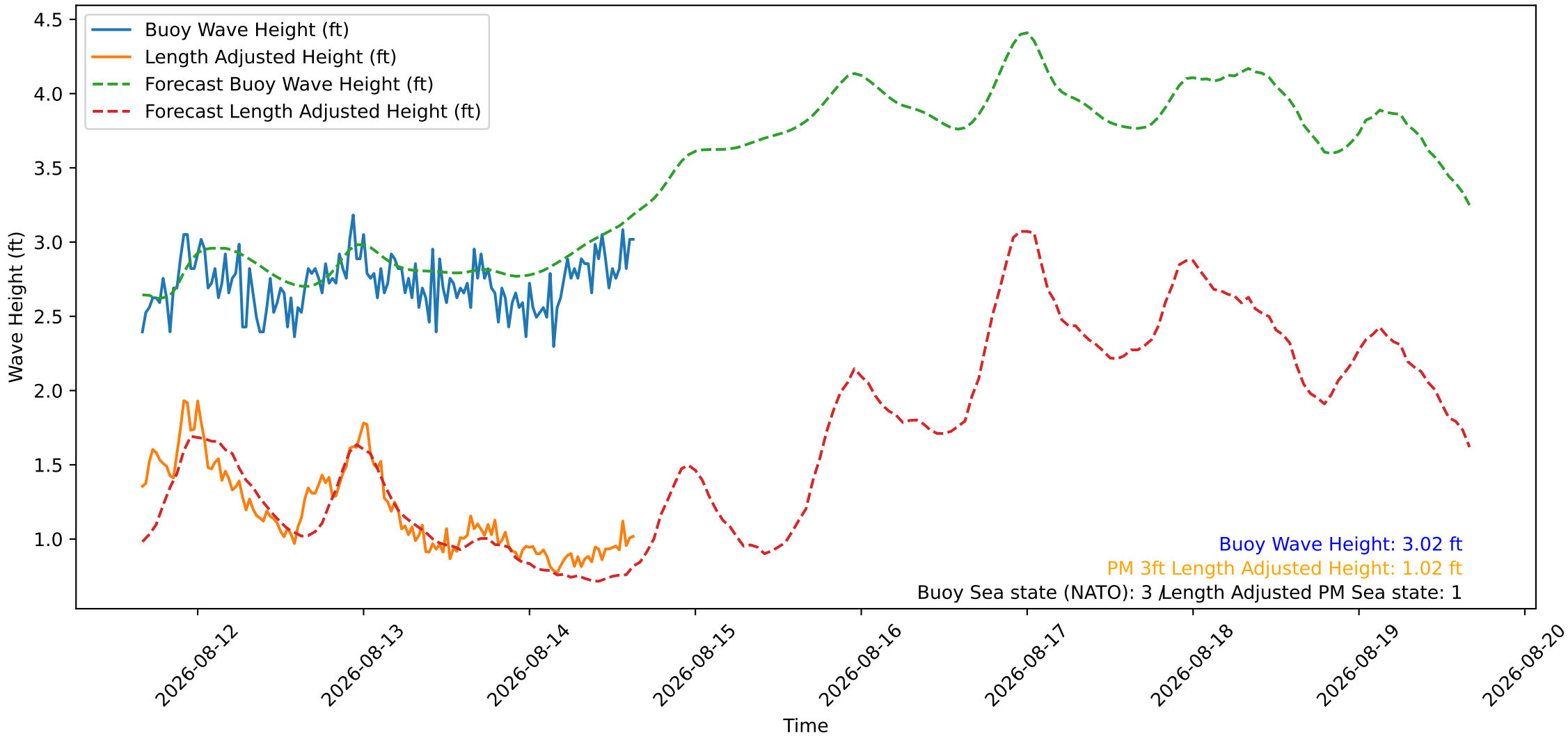
Wave Heights over Time for Oceanside Harbor at 2026-08-14 15:50:26
