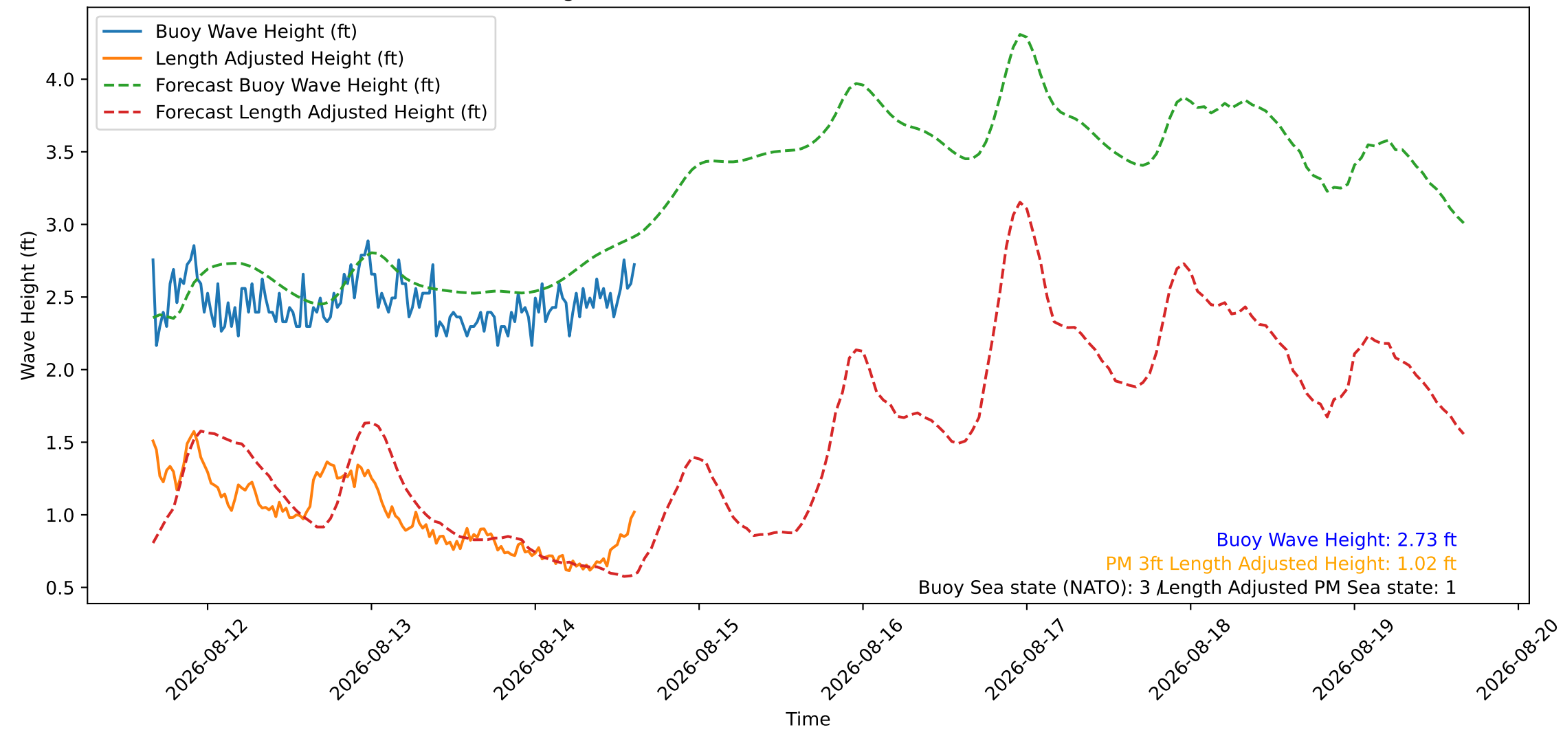
Wave Heights over Time for Red Beach at 2026-08-14 15:50:47
