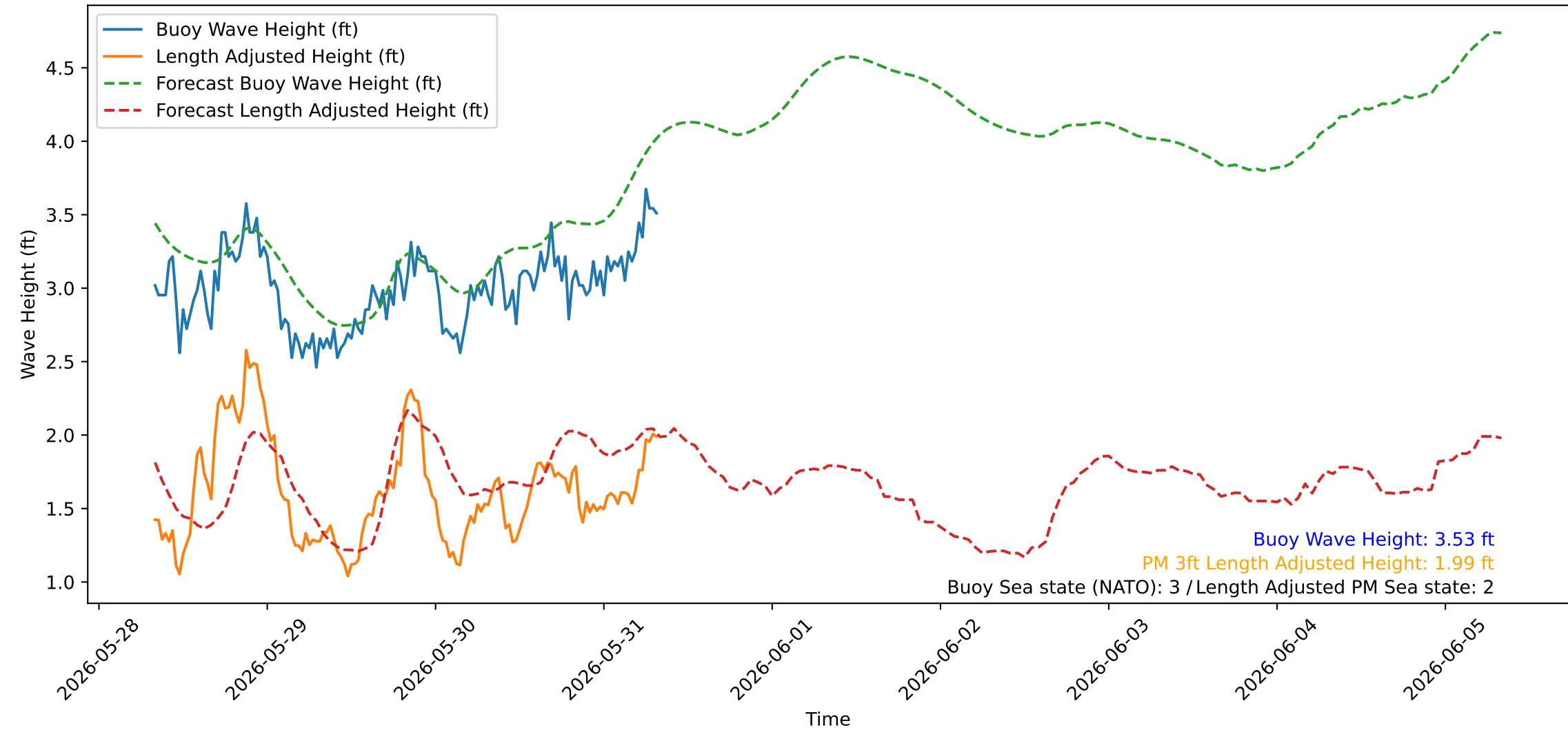
Wave Heights over Time for Green Beach at 2026-05-31 08:11:07
