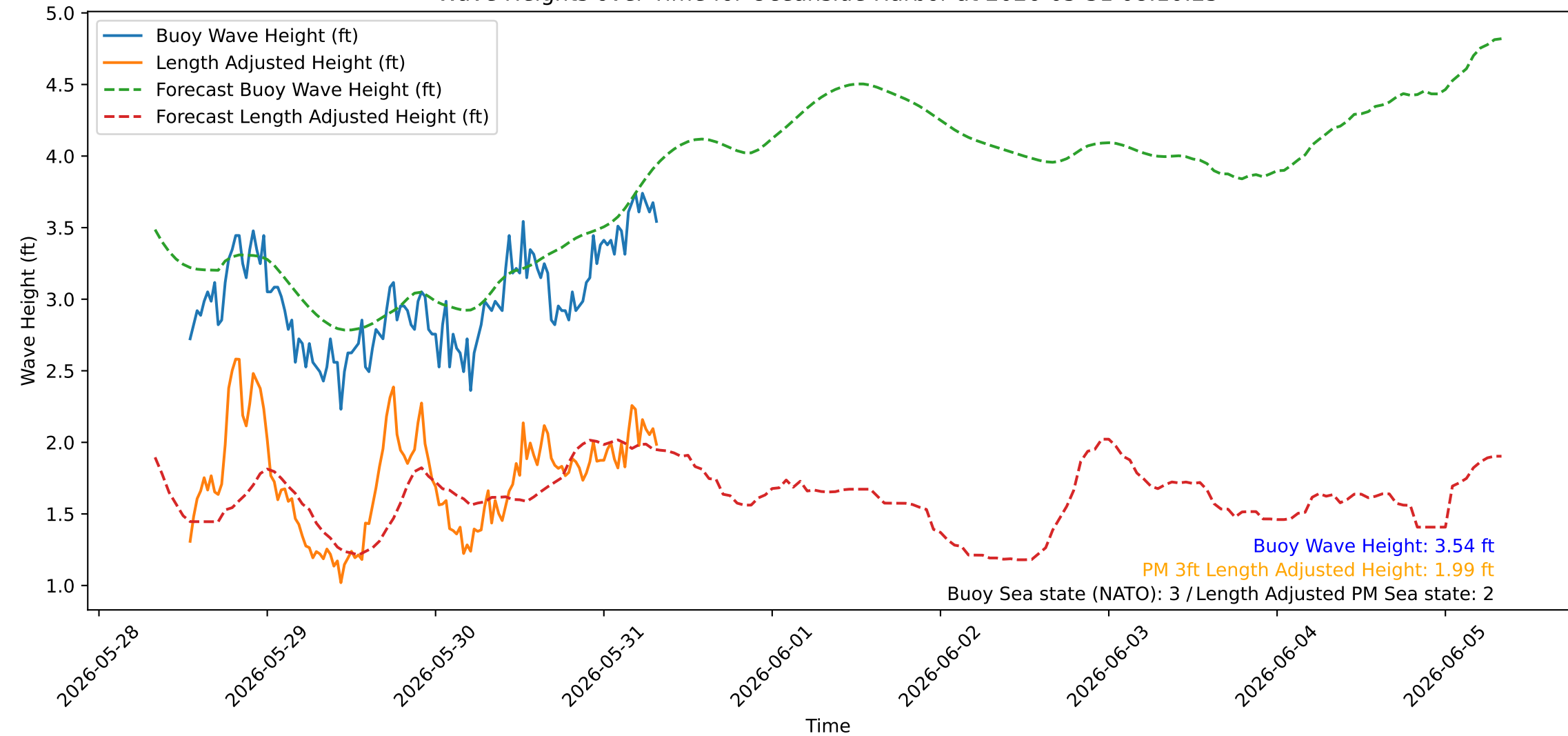
Wave Heights over Time for Oceanside Harbor at 2026-05-31 08:10:25
