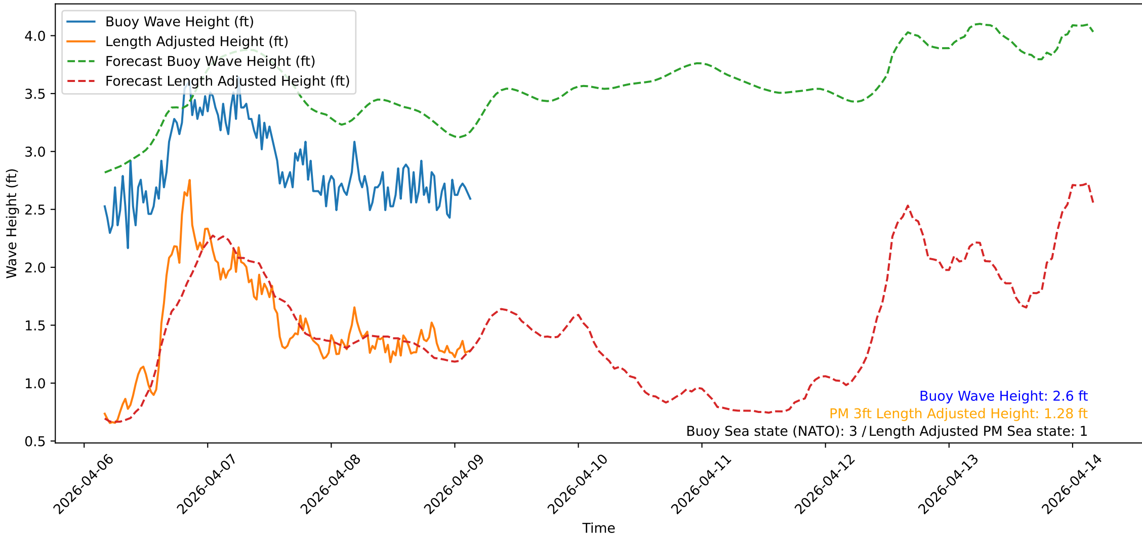
Wave Heights over Time for Oceanside Harbor at 2026-04-09 03:50:31
