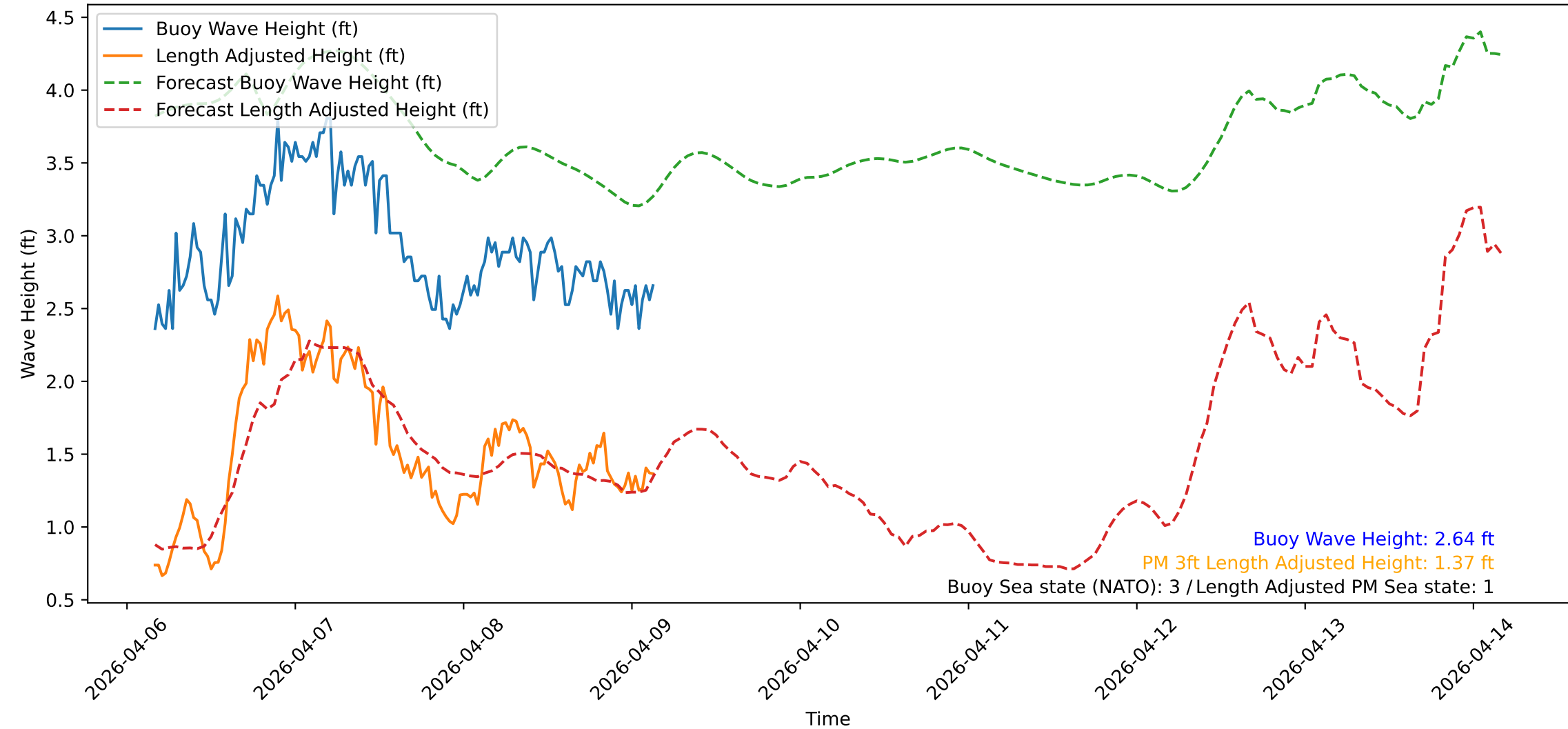
Wave Heights over Time for Green Beach at 2026-04-09 03:51:10
