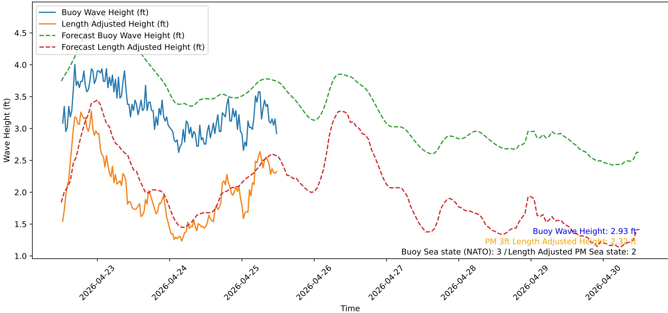
Wave Heights over Time for Green Beach at 2026-04-25 12:21:14
