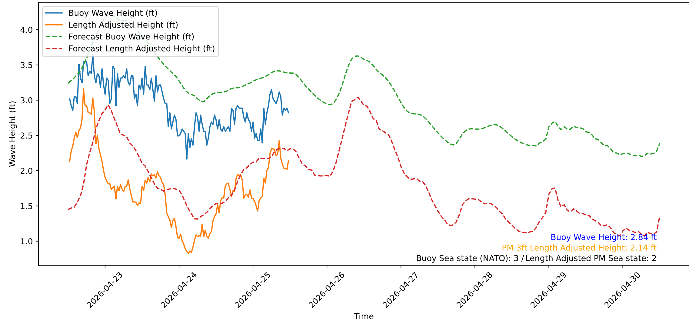
Wave Heights over Time for Red Beach at 2026-04-25 12:20:52
