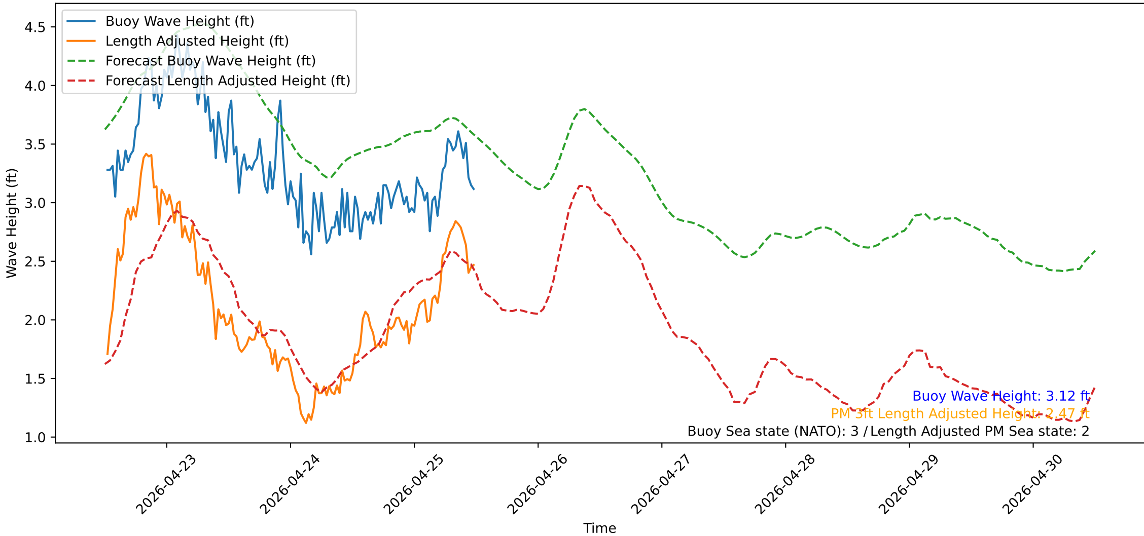
Wave Heights over Time for Oceanside Harbor at 2026-04-25 12:20:31
