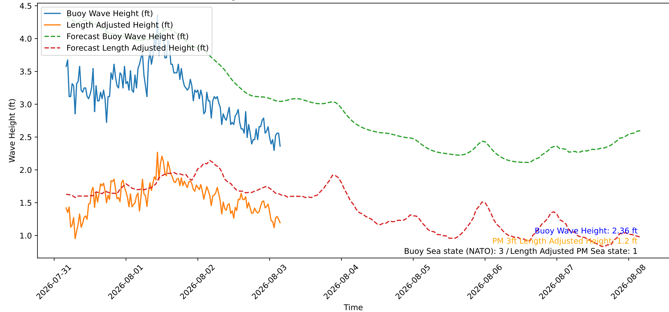
Wave Heights over Time for Oceanside Harbor at 2026-08-03 04:10:26
