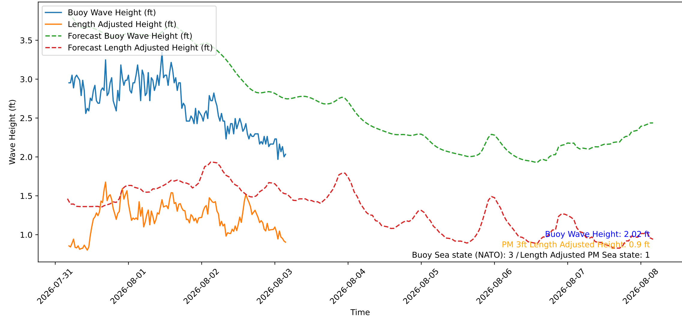
Wave Heights over Time for Red Beach at 2026-08-03 04:10:45
