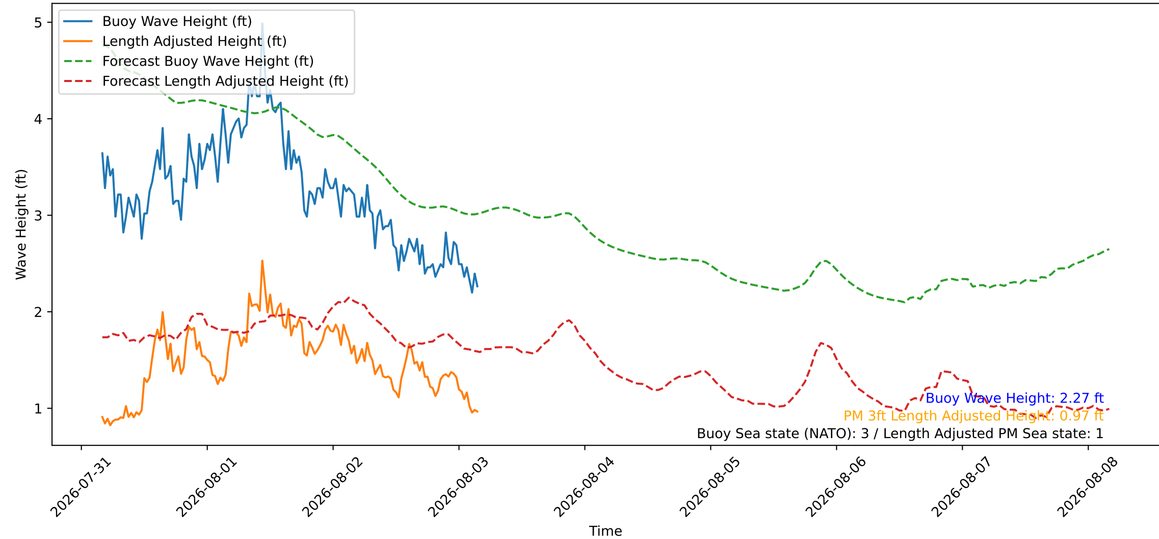
Wave Heights over Time for Green Beach at 2026-08-03 04:11:08
