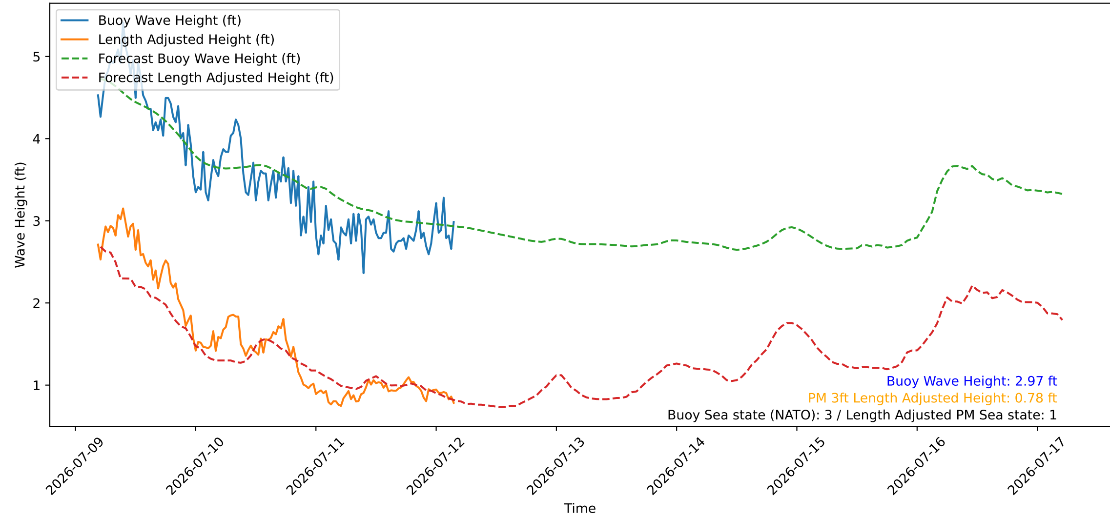
Wave Heights over Time for Oceanside Harbor at 2026-07-12 04:30:27
