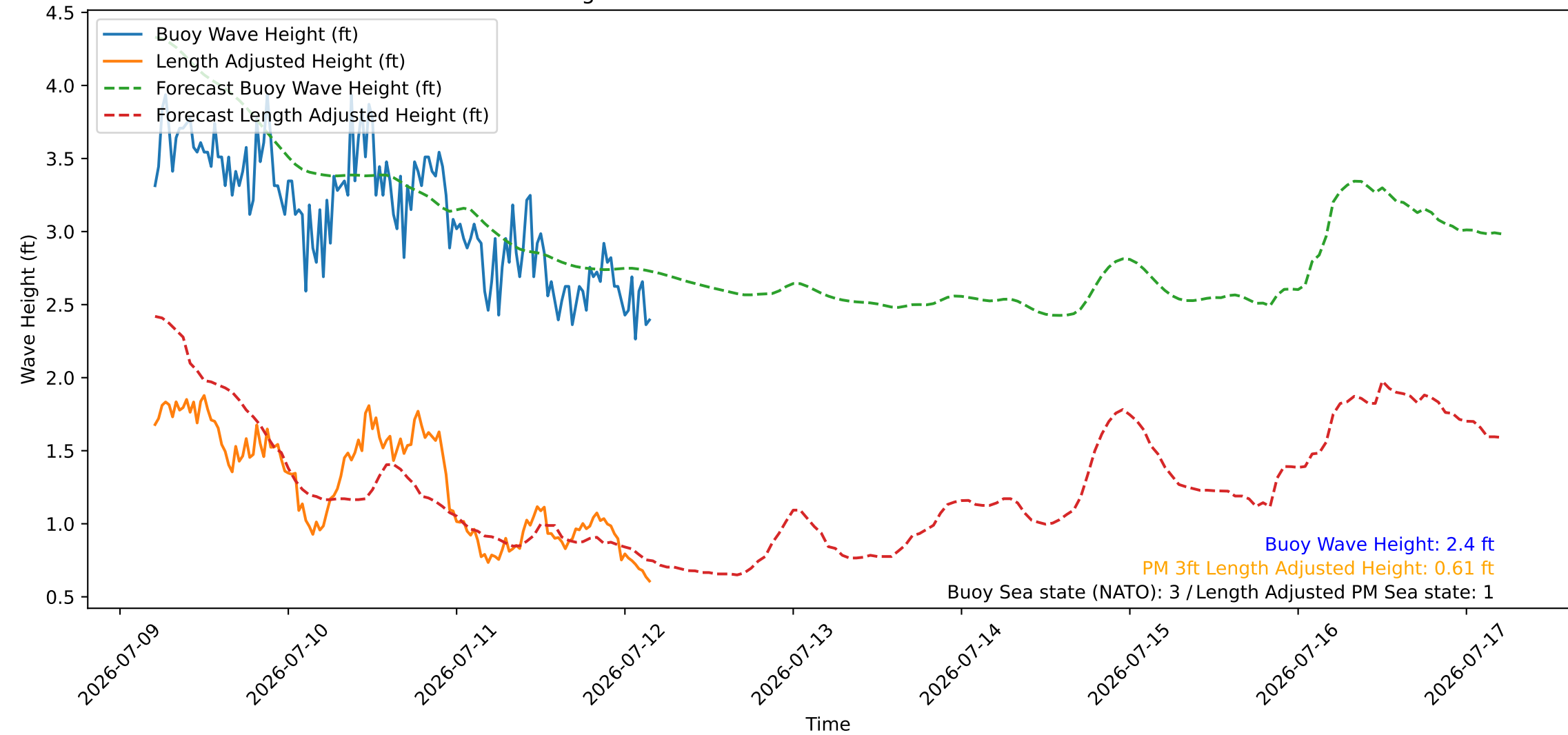
Wave Heights over Time for Red Beach at 2026-07-12 04:30:45
