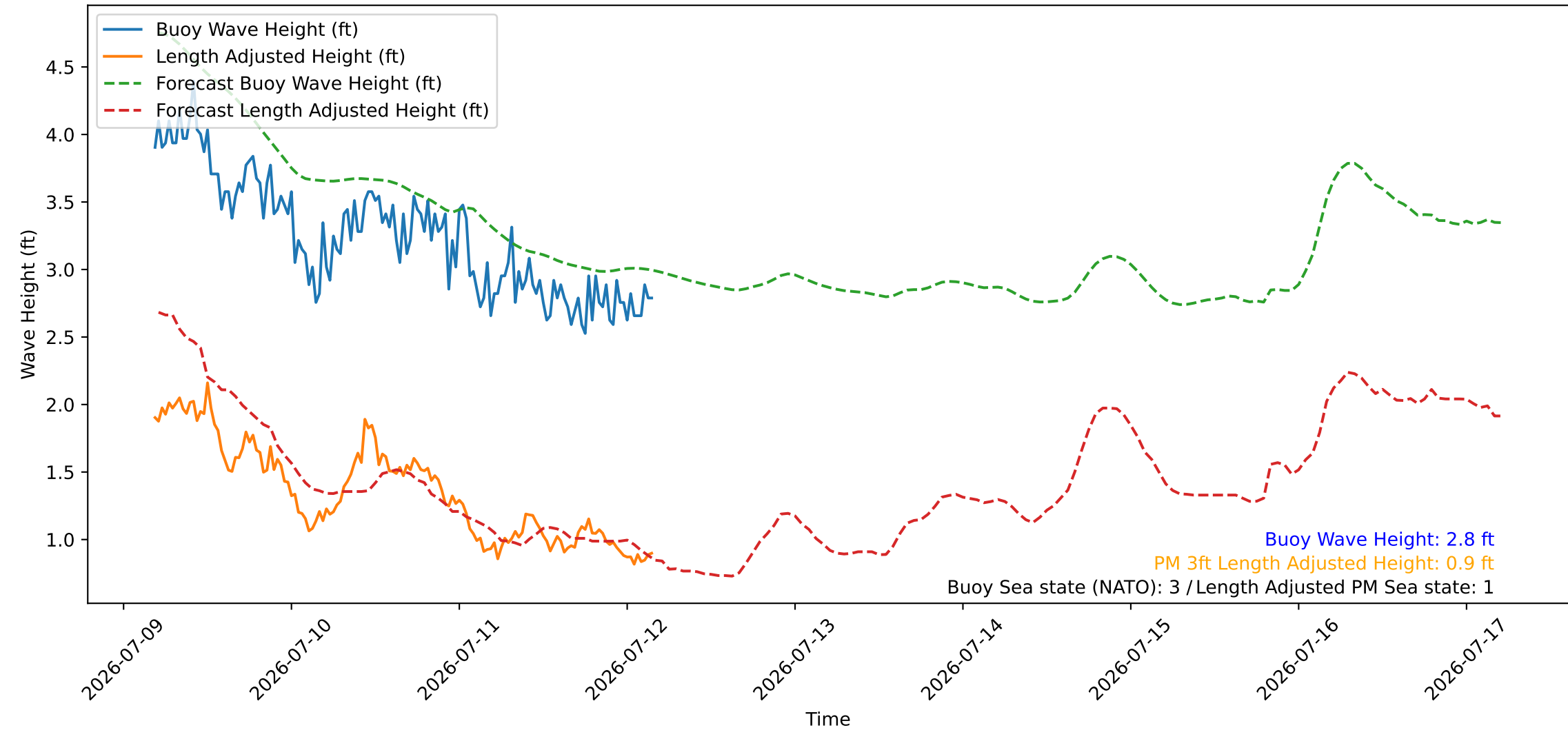
Wave Heights over Time for Green Beach at 2026-07-12 04:31:07
