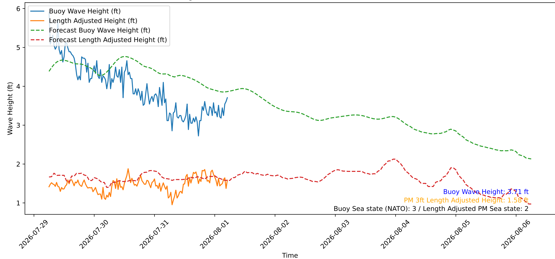
Wave Heights over Time for Oceanside Harbor at 2026-08-01 06:00:26
