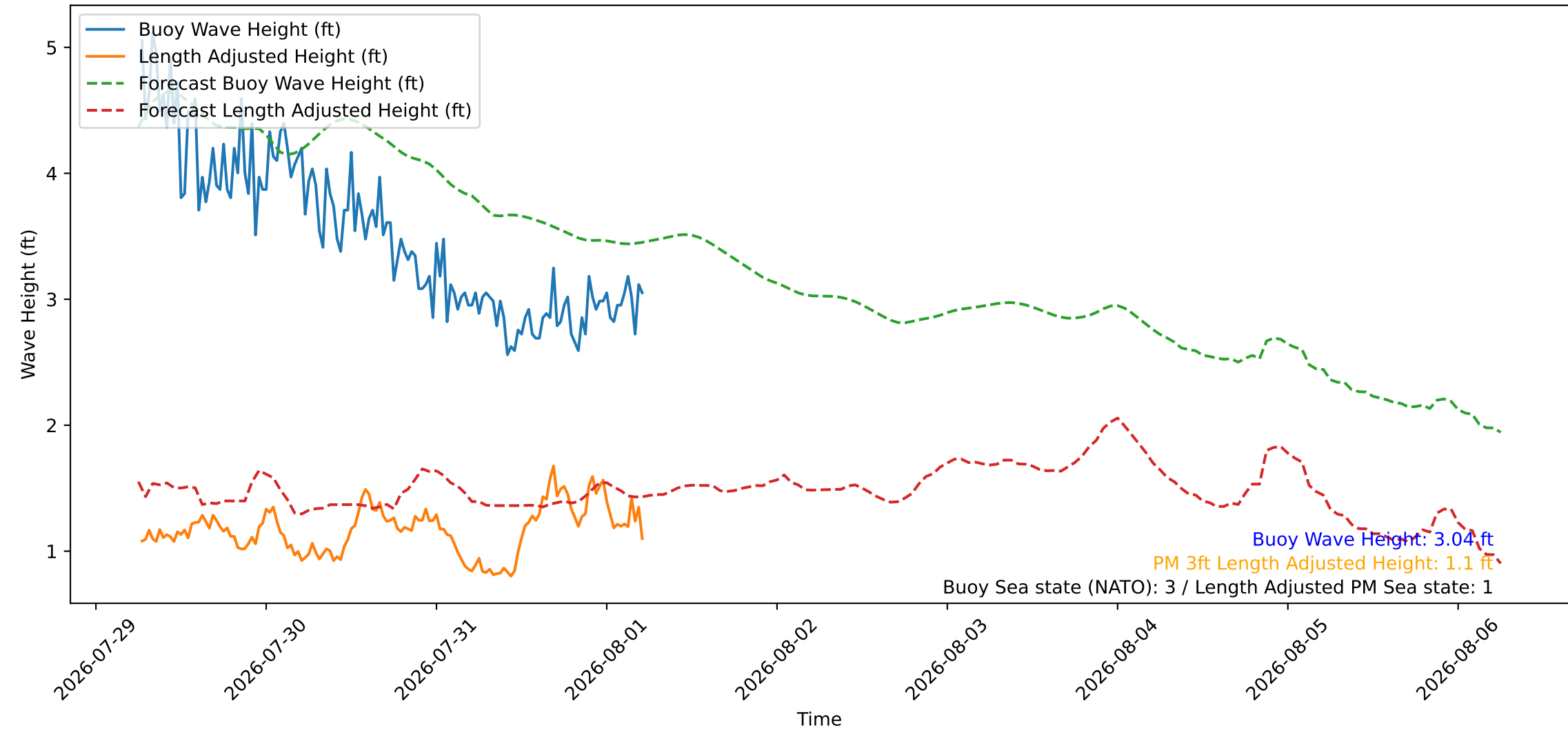
Wave Heights over Time for Red Beach at 2026-08-01 06:00:46
