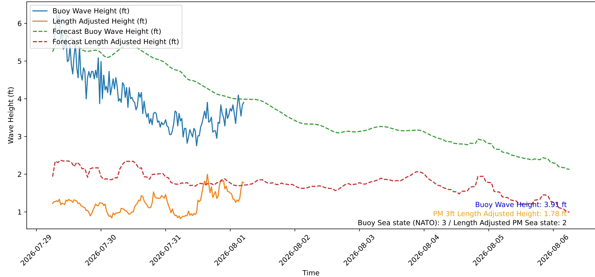
Wave Heights over Time for Green Beach at 2026-08-01 06:01:08
