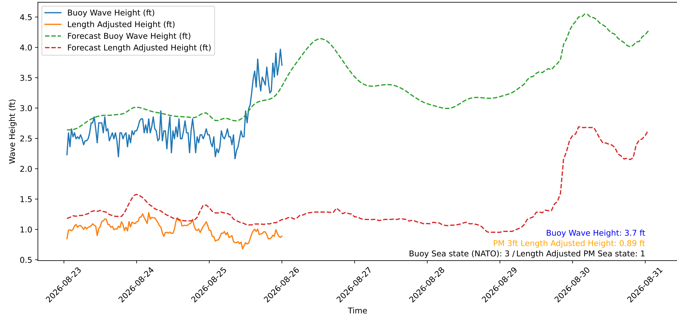
Wave Heights over Time for Red Beach at 2026-08-26 00:50:49
