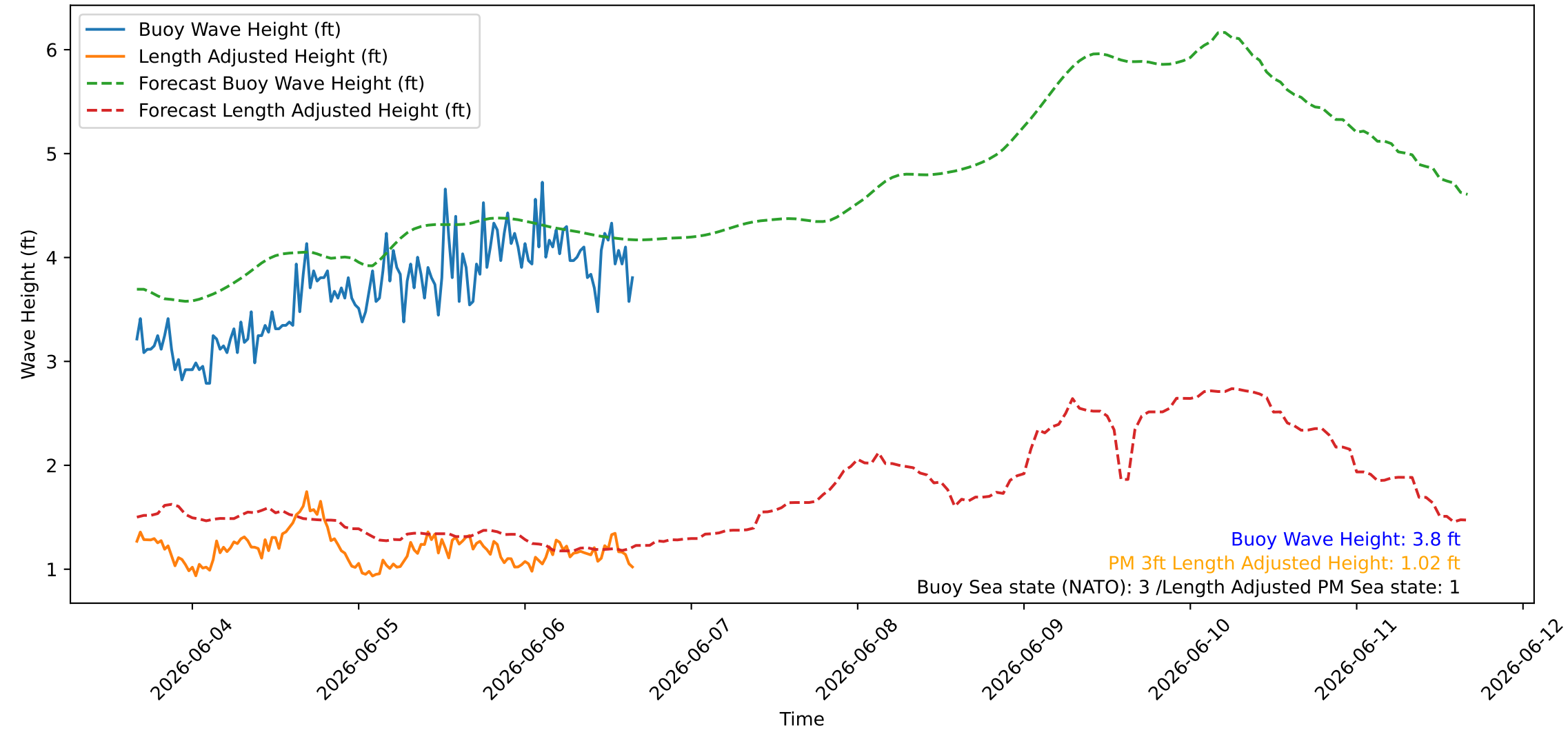
Wave Heights over Time for Green Beach at 2026-06-06 16:11:07
