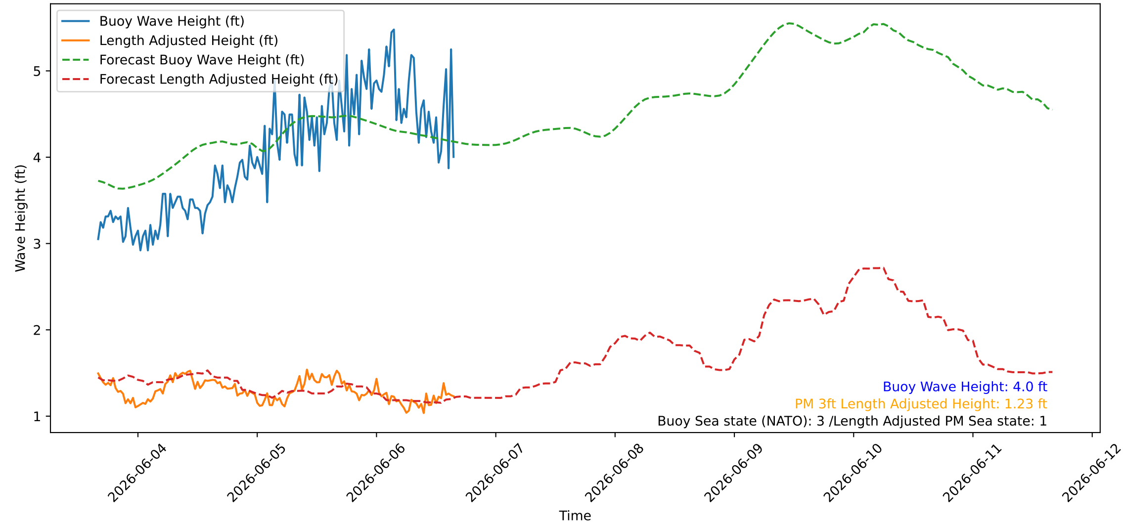
Wave Heights over Time for Oceanside Harbor at 2026-06-06 16:10:26
