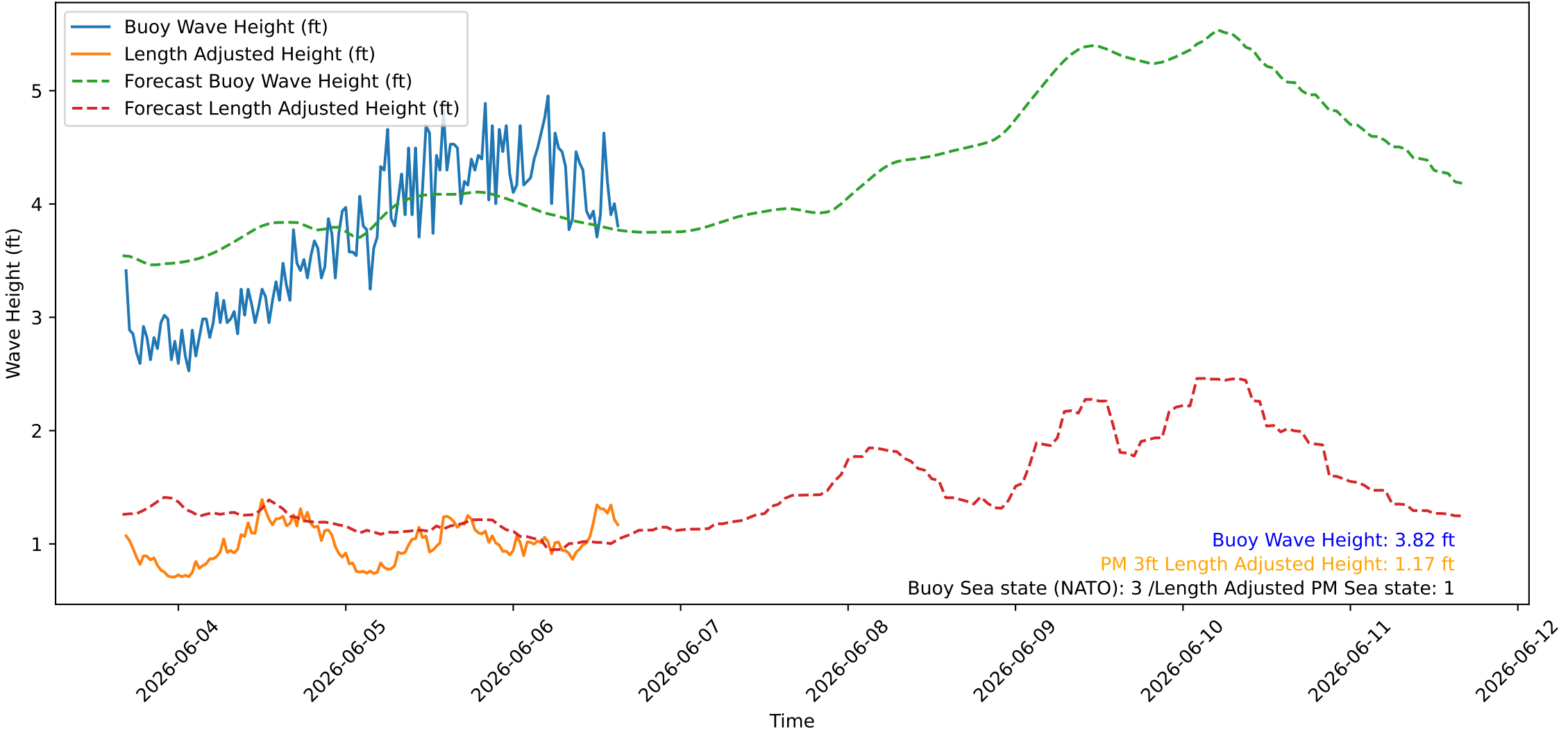
Wave Heights over Time for Red Beach at 2026-06-06 16:10:45
