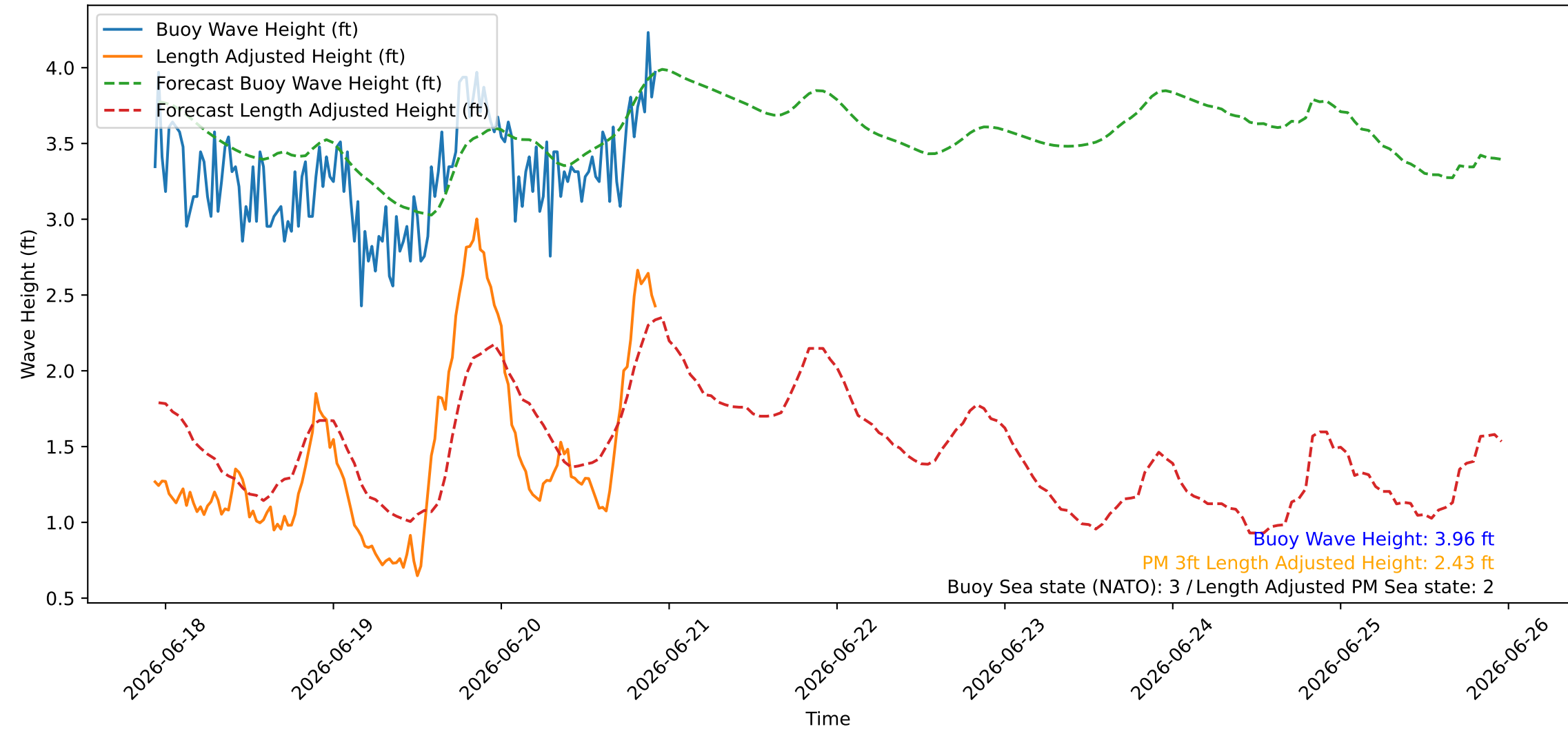
Wave Heights over Time for Green Beach at 2026-06-20 22:41:07
