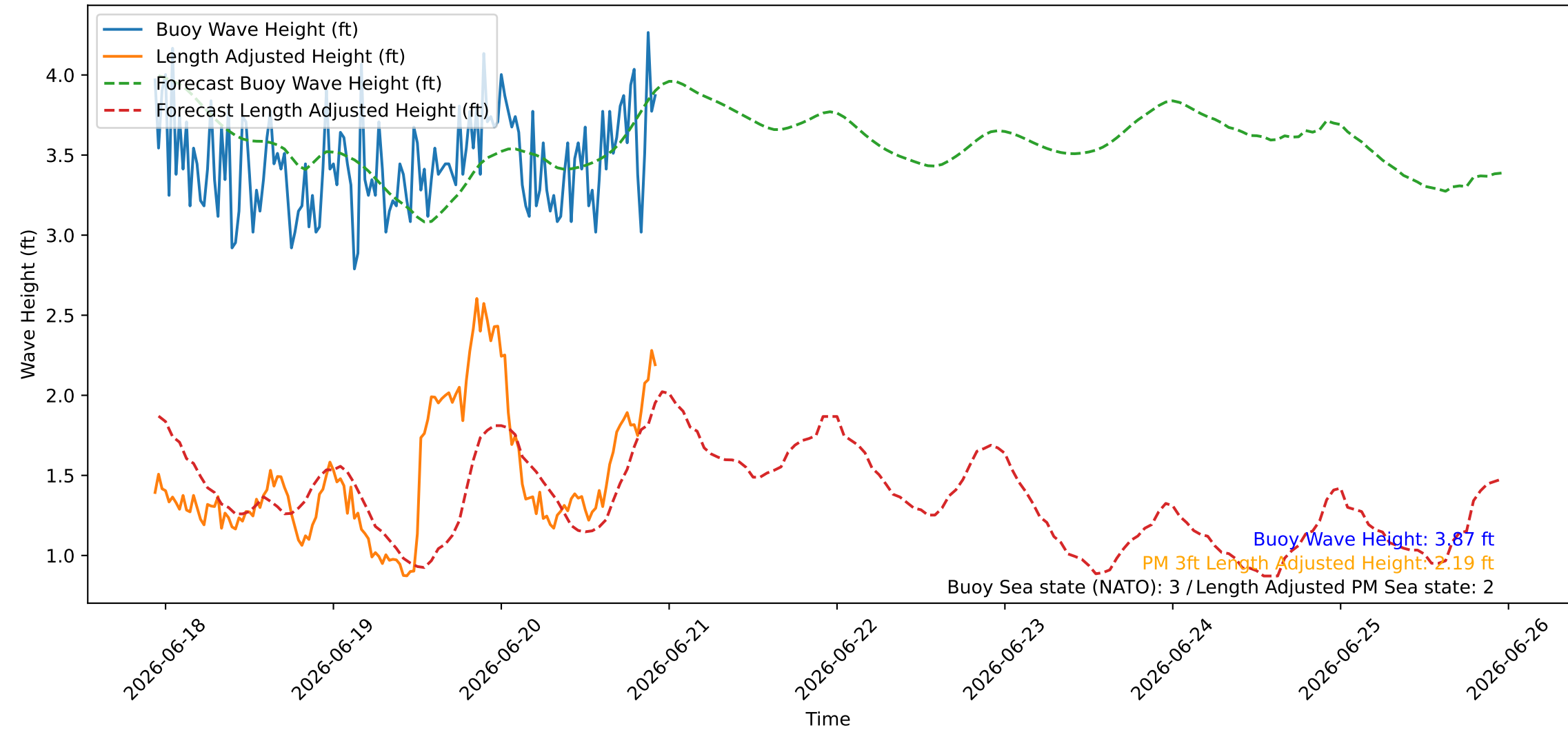
Wave Heights over Time for Oceanside Harbor at 2026-06-20 22:40:26
