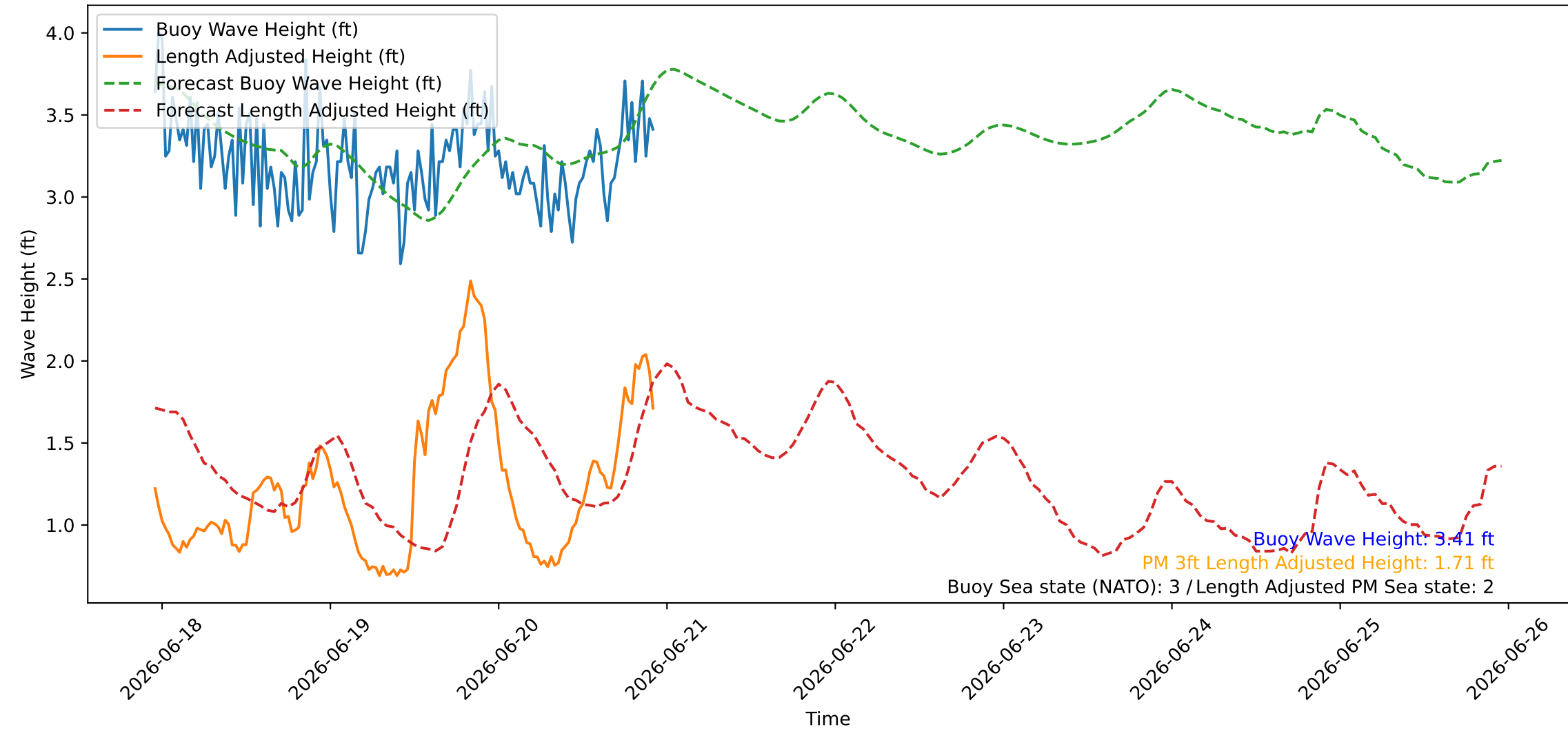
Wave Heights over Time for Red Beach at 2026-06-20 22:40:45
