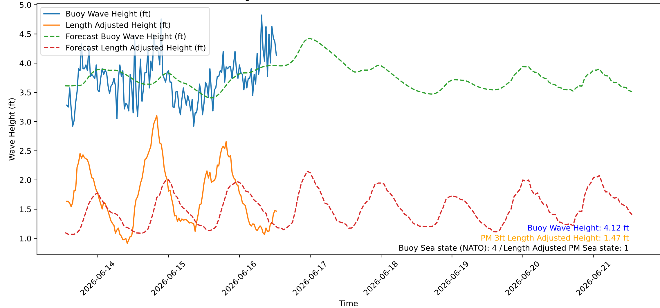
Wave Heights over Time for Red Beach at 2026-06-16 13:10:45
