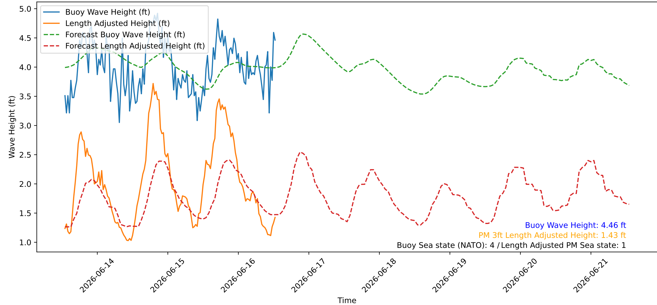
Wave Heights over Time for Green Beach at 2026-06-16 13:11:08
