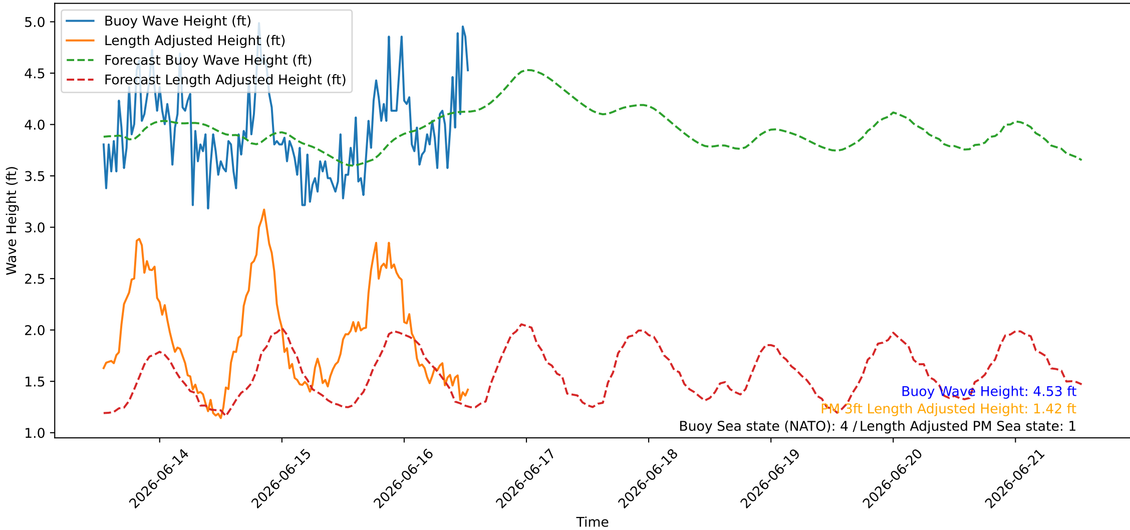
Wave Heights over Time for Oceanside Harbor at 2026-06-16 13:10:26
