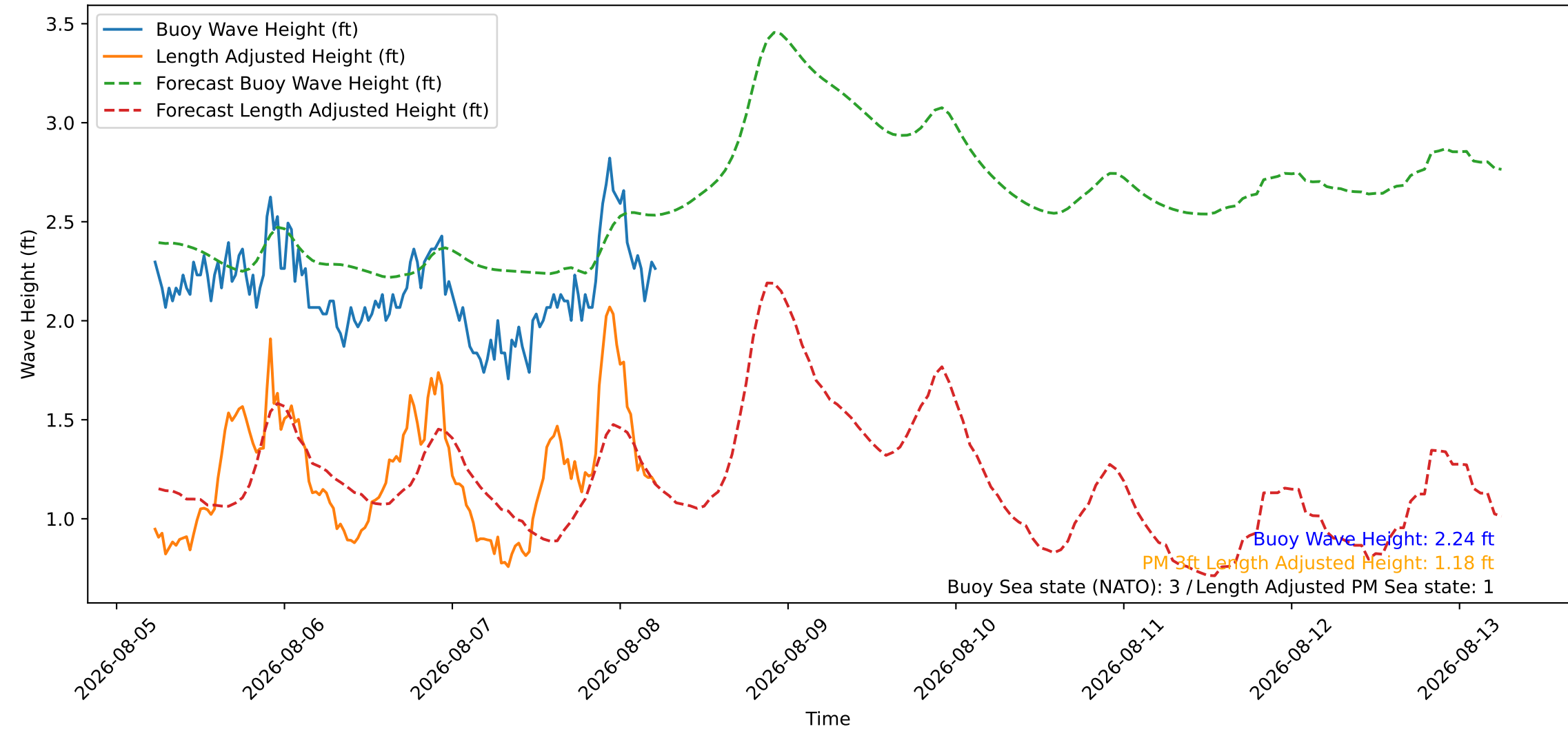
Wave Heights over Time for Green Beach at 2026-08-08 05:41:08
