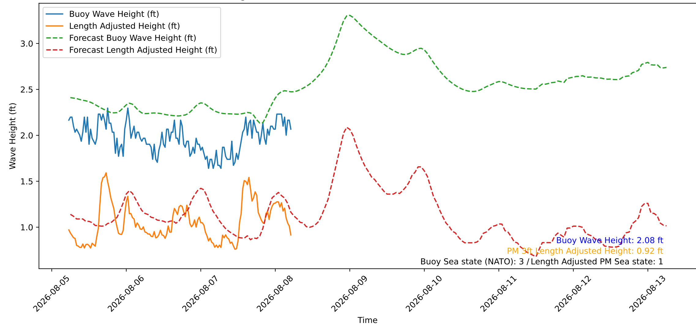
Wave Heights over Time for Oceanside Harbor at 2026-08-08 05:40:26
