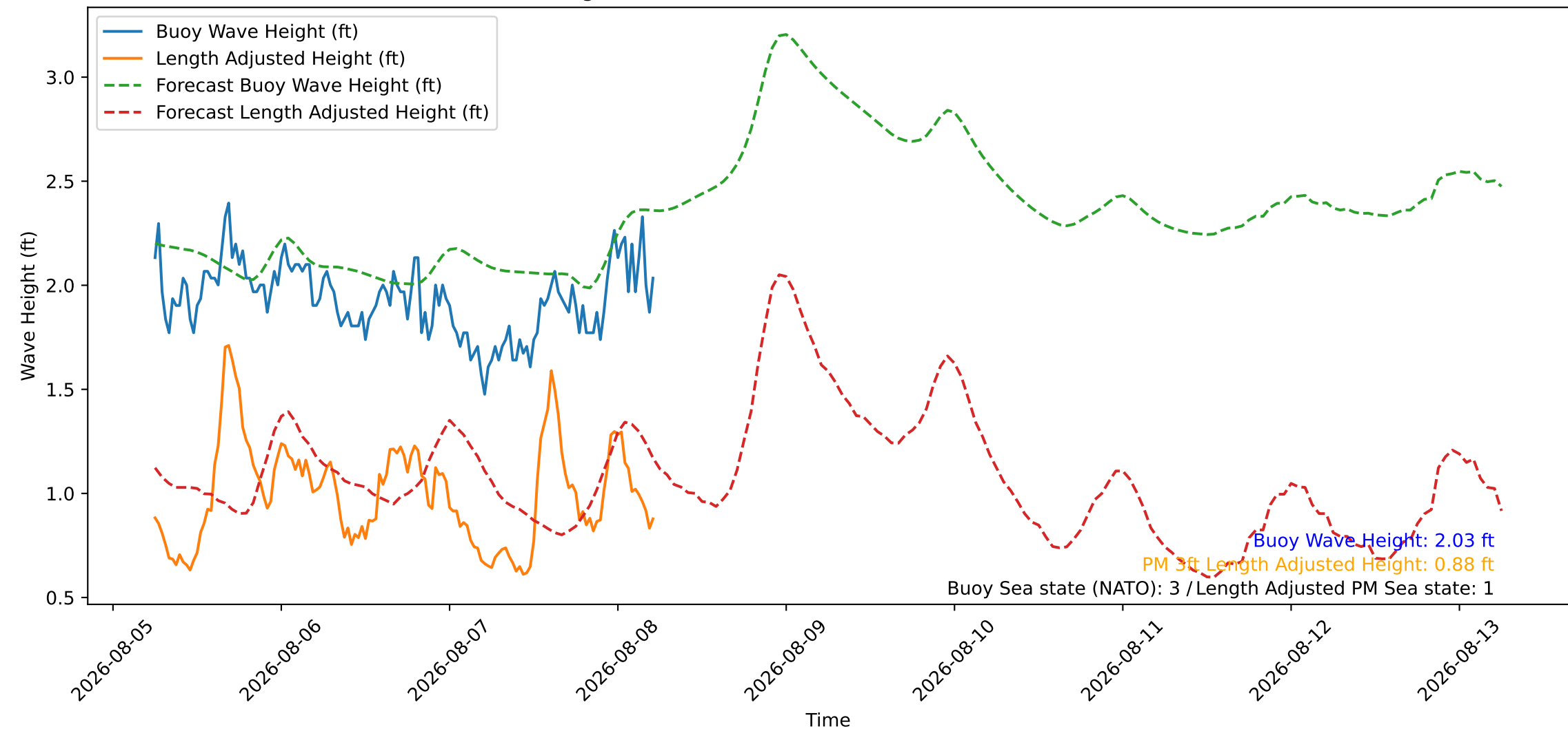
Wave Heights over Time for Red Beach at 2026-08-08 05:40:46
